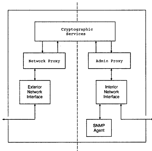
Figure 3: DNMS Implementation
