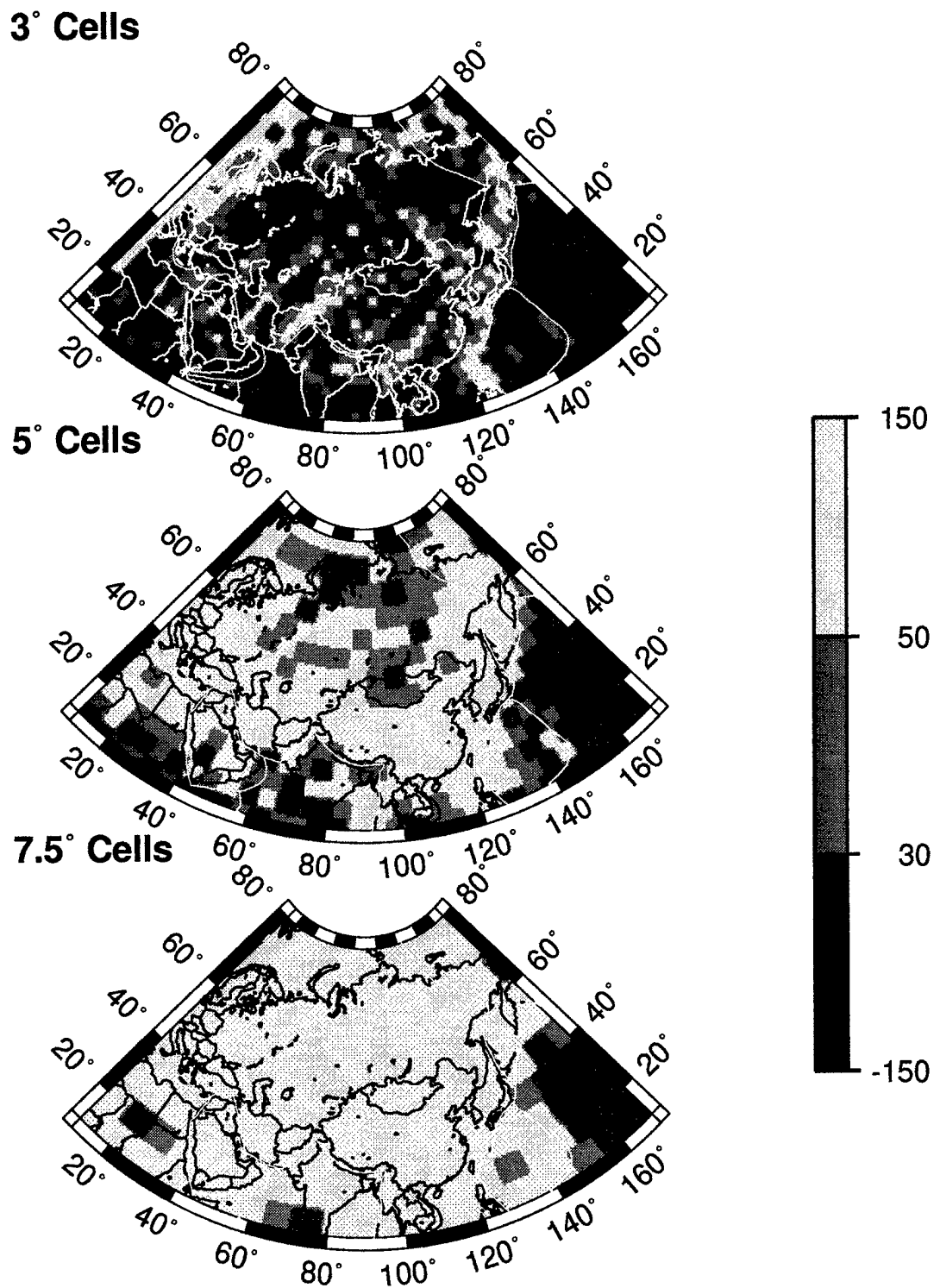
Figure 10b. Plots of the resolution index ( \mathcal{R} , eqn. (6)) for the 40 s Rayleigh wave with the same cell sizes as in Fig. 10a. Light grey cells are considered resolved, increasingly darker cells denote poorer resolution. The same sort of information is included in these figures as in Fig. 10a, but in this form it is more readily and quickly interpreted.
