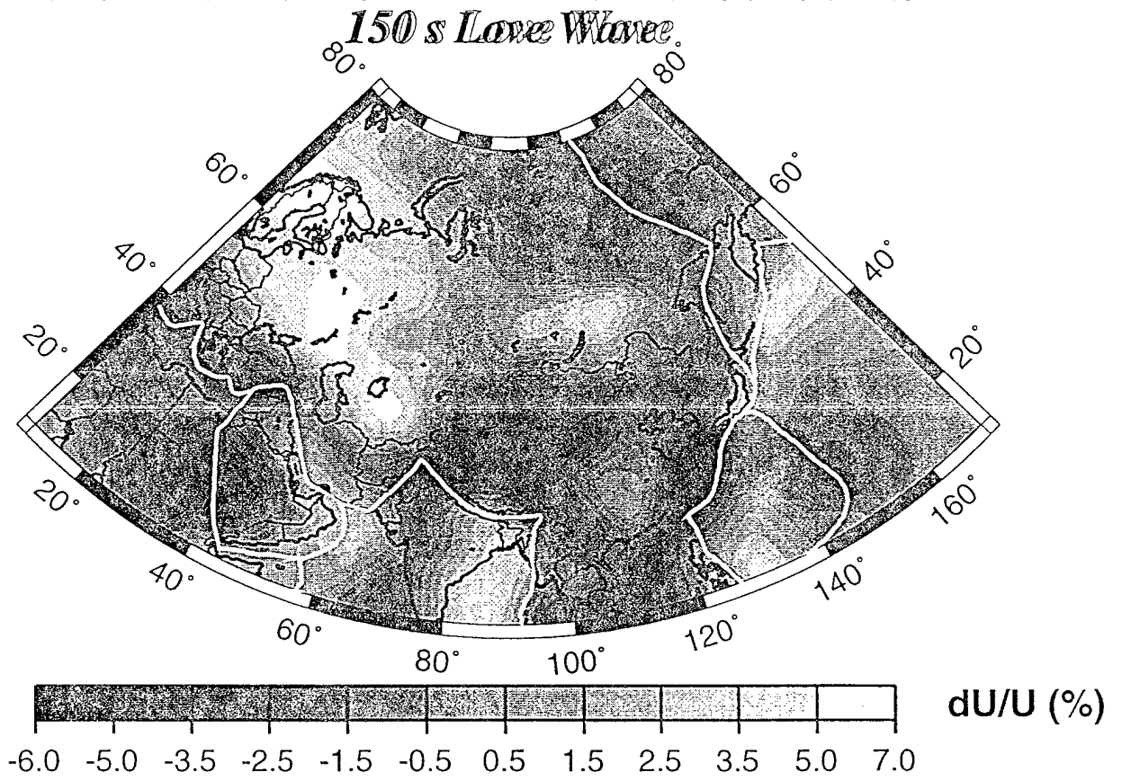
Figure 18f. Same as Figure 18a, except for the 125 s and 150 s Love waves.
