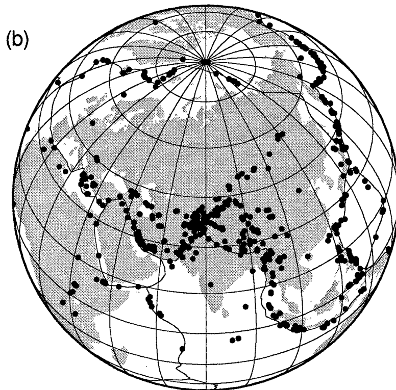
Figure 2. Station and event location. The locations of the stations used in this study are marked with triangles in (a) and event locations are marked with circles in (b).
