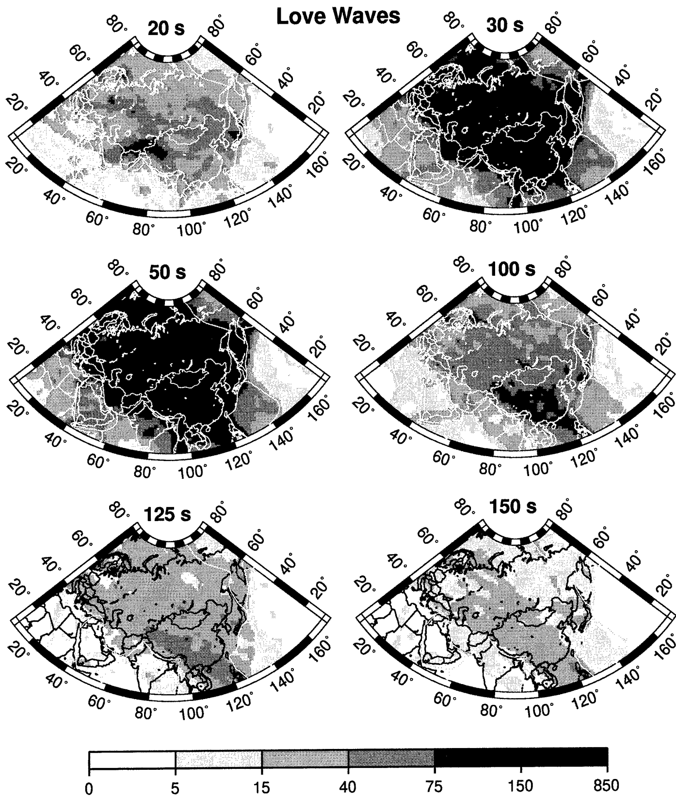
Figure 9b. The same as Figure 9a, but for Love waves at the indicated periods.
