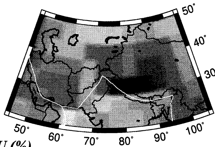
Rayleigh 50s: CRUST-5.1/S16B
