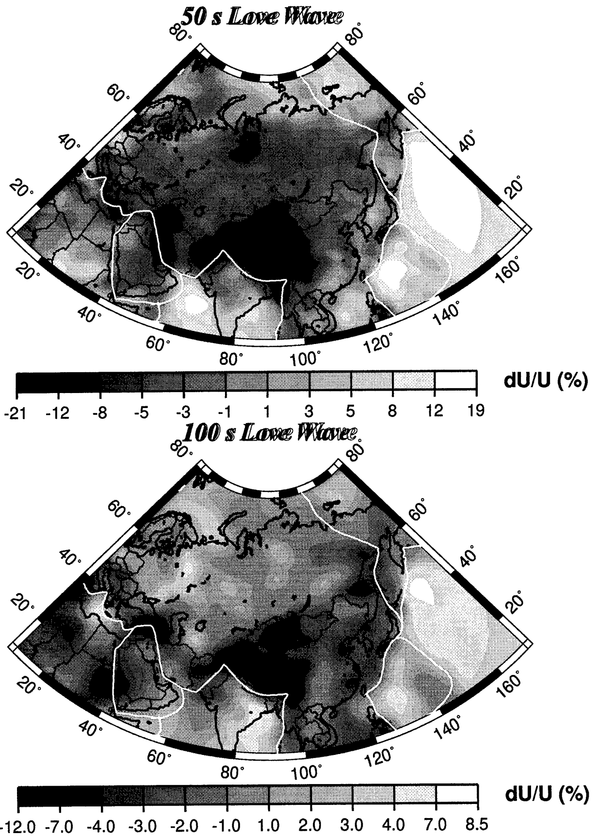
Figure 18e. Same as Figure 18a, except for the 50 s and 100 s Love waves.
