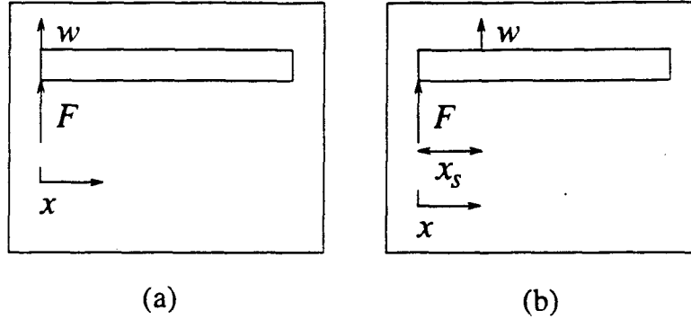
Figure 3.2: Free-Free Beams with (a) Collocated, (b) Noncollocated Point Actuator-Sensor Pairs
