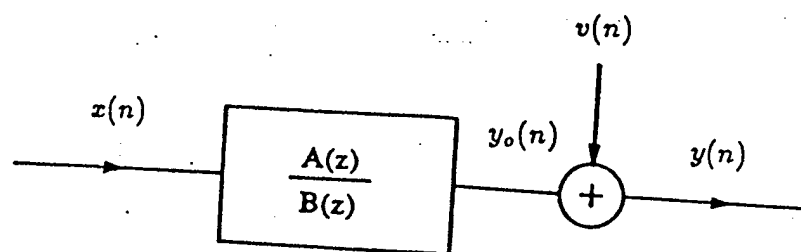
Fig. 1. The Output Error Model Structure
