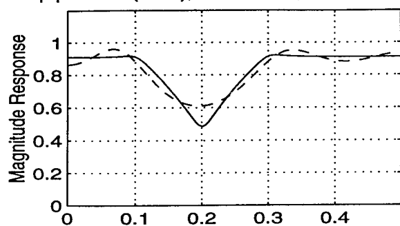
CLA ( M=4 ), Ncoeff = 8, error=-26.7dB
