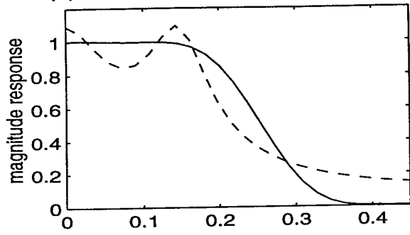
CLA ( M=4 ), Ncoeff=9, error=-19.5 dB
