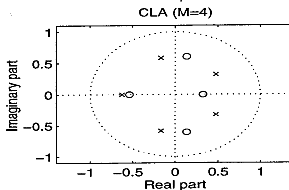
CLA ( M=4 ), Ncoeff = 8, error=-26.7dB
