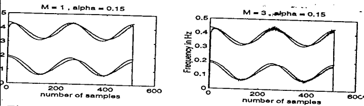
Figure 5: Adaptive tracking using (a) SLMS (b) PLMS
