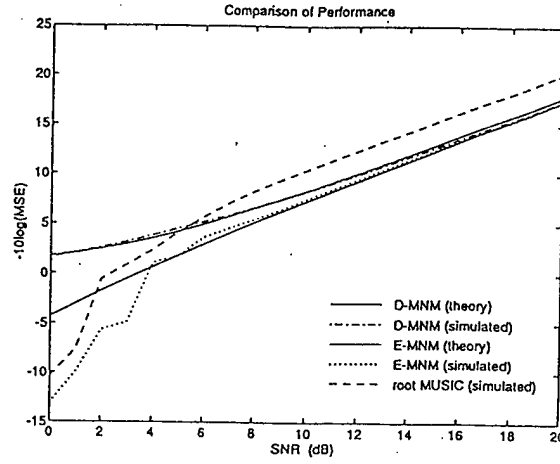
Fig.6 Performance comparison of three methods using all 200 trials.
