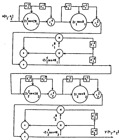
FIG 3: Implementation of the second-order blocks in both domains after 4-stages of scattered pipelining with decomposition technique inside the recursive loop.
