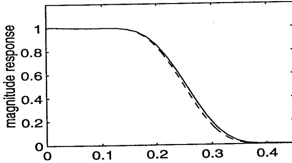
DLA ( M=4 ), Ncoeff=11, error=-32.5 dB
