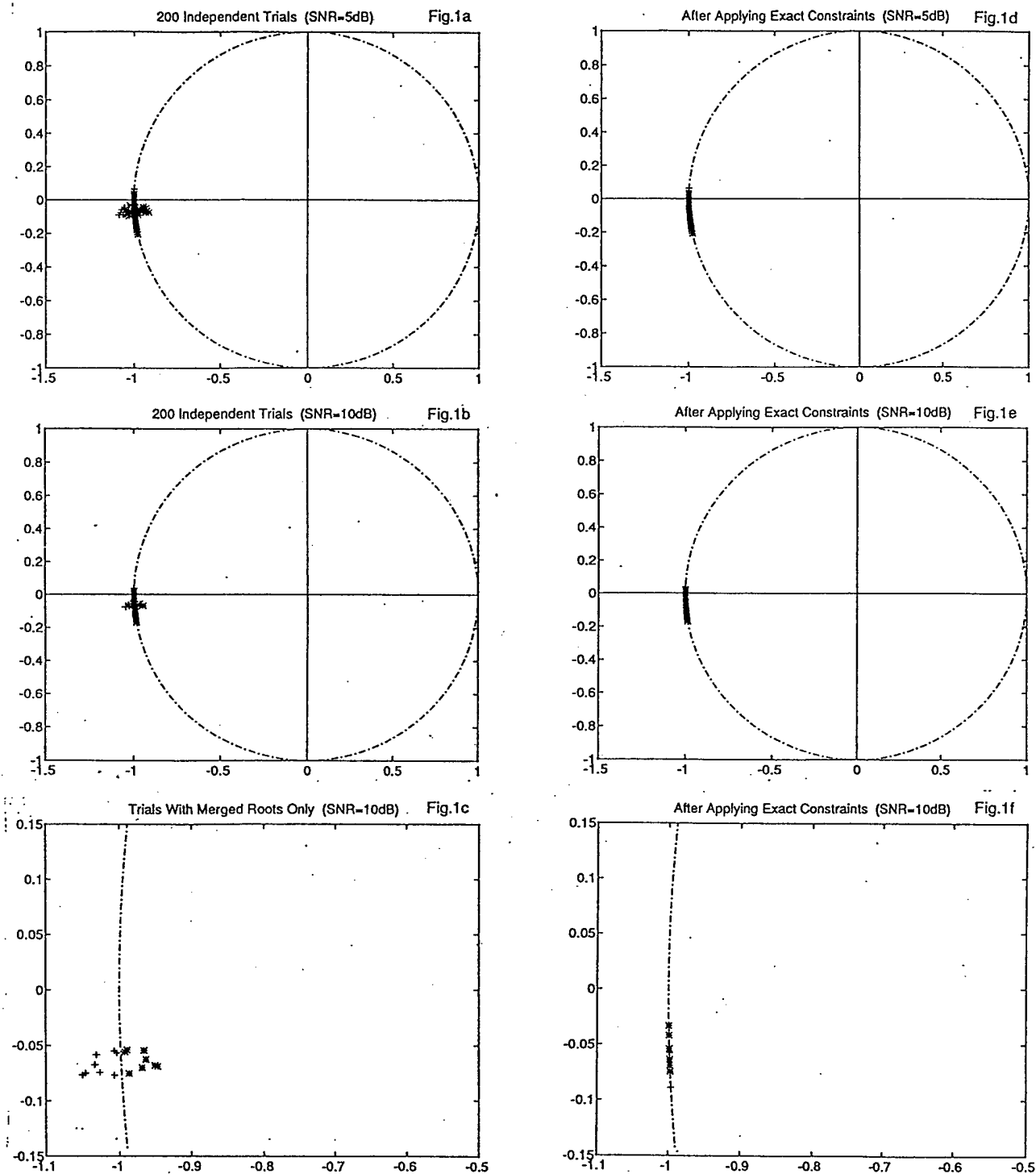
Fig. 1 : Superimposed plots of estimated roots for 200 independent trials using MLE (a-c) and C-MLE (d-f).
