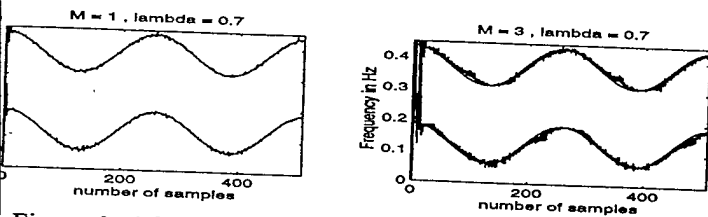
Figure 6: Adaptive tracking using (a) SRLS (b) PRLS
