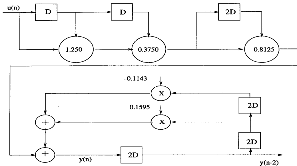
Figure 5: Implementation of a 4-stage DLA Pipelined recursive Filter Using Decomposition Technique
