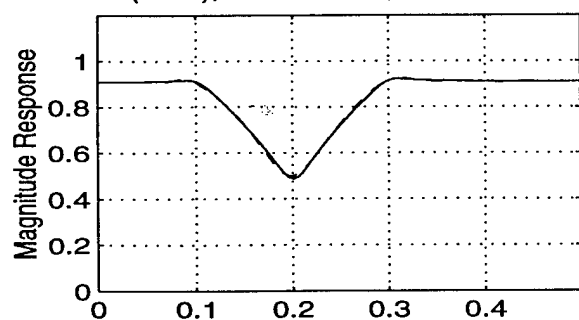
DLA ( M=4 ), Ncoeff = 12, error=-43.42dB
