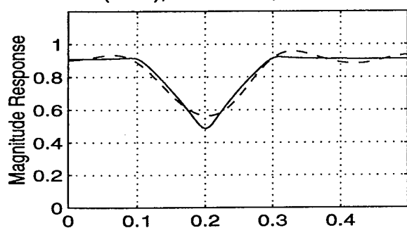
SLA ( M=4 ), Ncoeff = 20, error=-54.22dB
