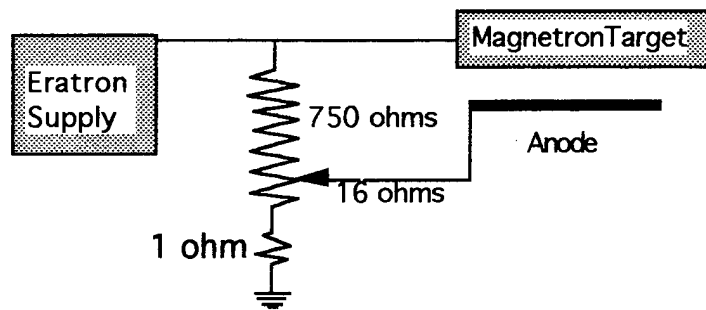
Figure 15 Anode for "low" plasma voltage
