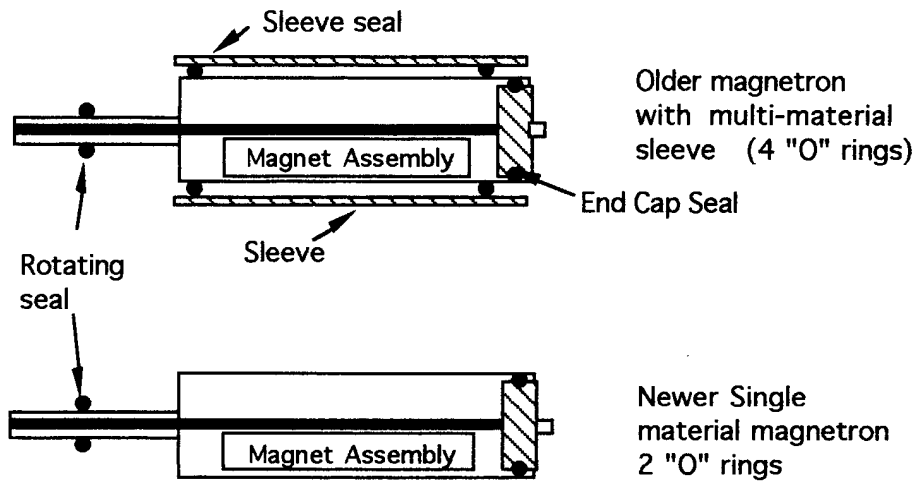
Figure 9 Magnetron designs
