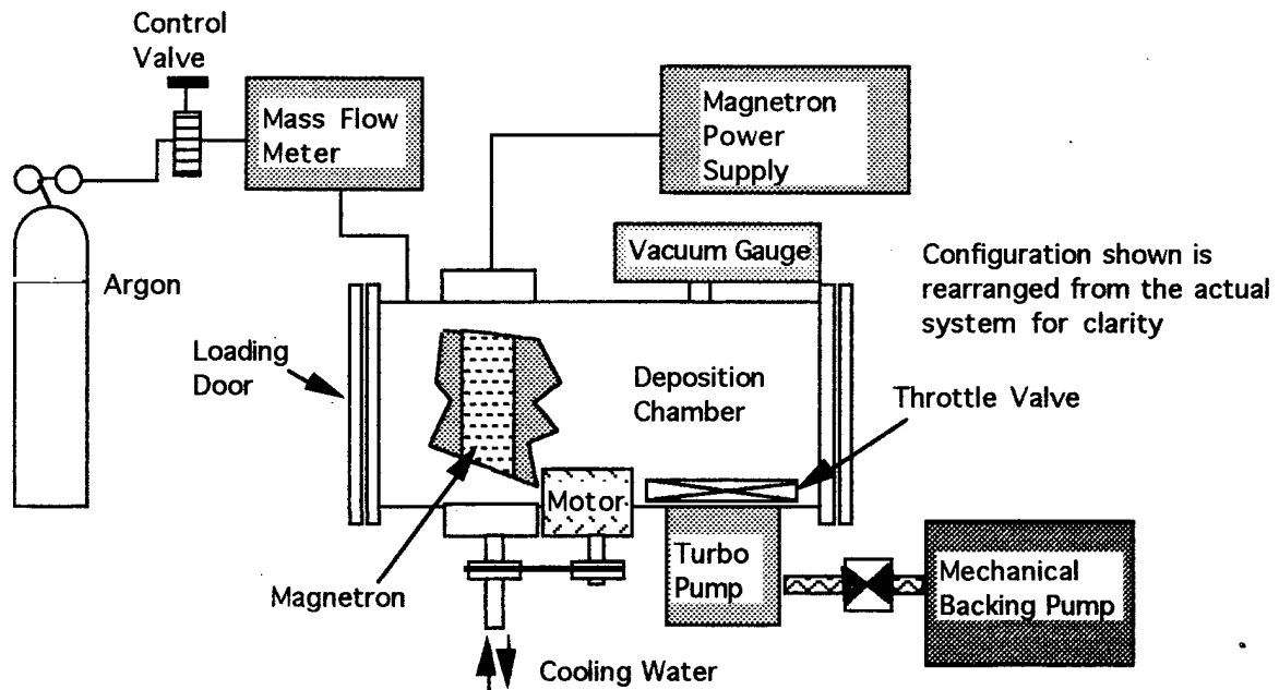
Figure 14 System diagram
