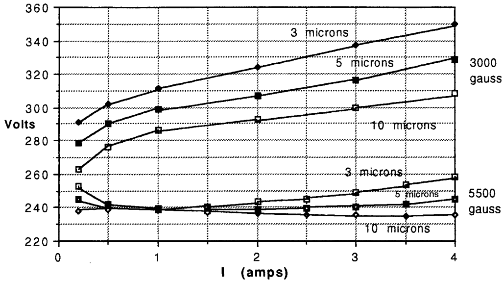
Fig 19 Stainless Steel IV curve
