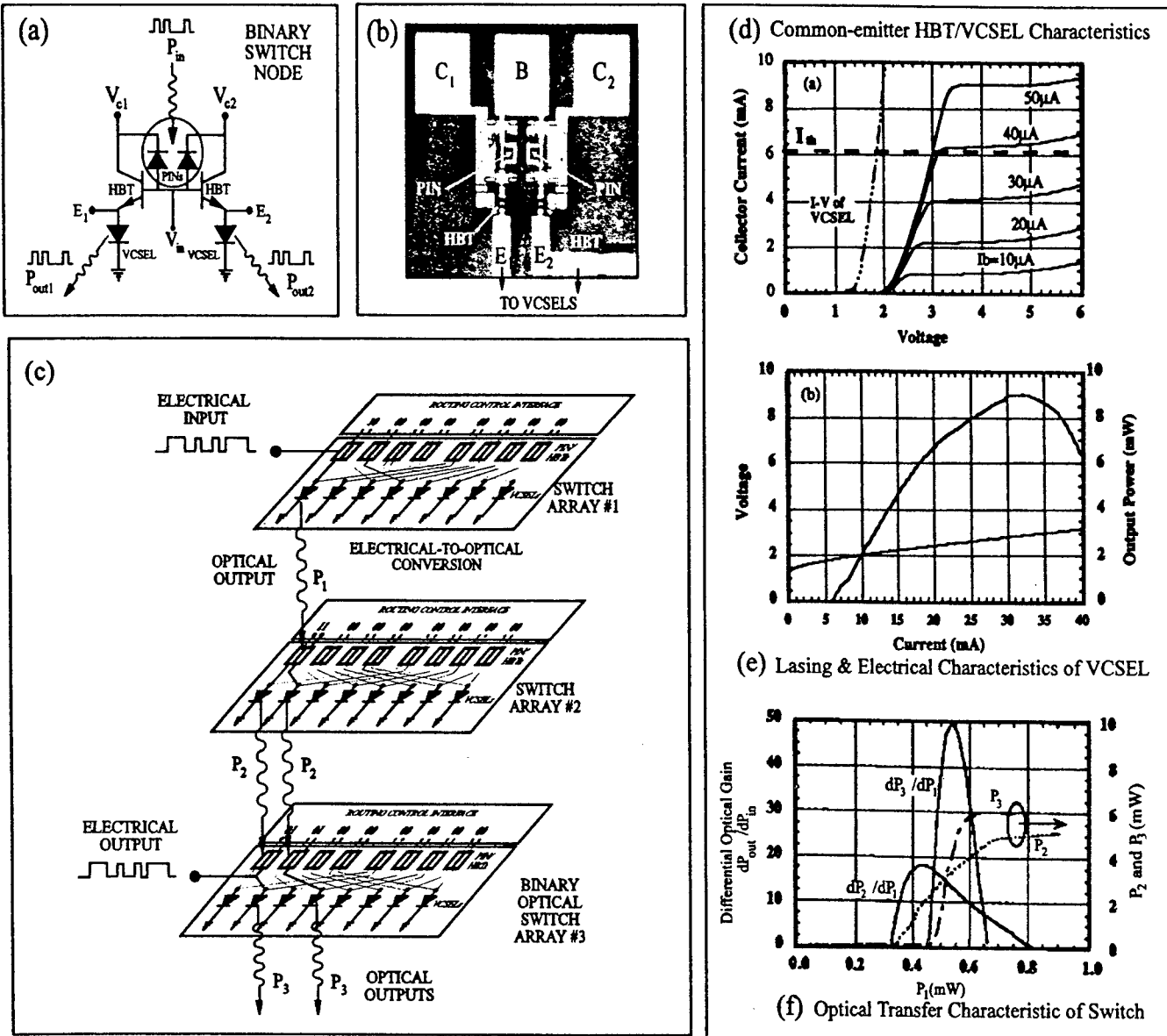
Figure . (a) The circuit design, and (b) layout of a reconfigurable binary PIN/HBT/VCSEL optical routing switch. (c) shows an optically-cascaded, multi-stage switching network using arrays of binary switches to perform optical routing functions. (d) shows the common-emitter characteristics of the HBT, (e) shows the lasing and electrical characteristics of the VCSEL, while (f) shows the differential optical gain of each of the two stages under optically cascaded dc switching operation.
