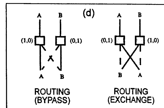
Figure 11 (a) Optical bypass-exchange routing operation using a reconfigurable binary optical routing switch consisting of two pairs of monolithic HPT/VCSEL switches. The switch layout is shown in (b), its circuit diagram in (c), and its switching functions in (d).
