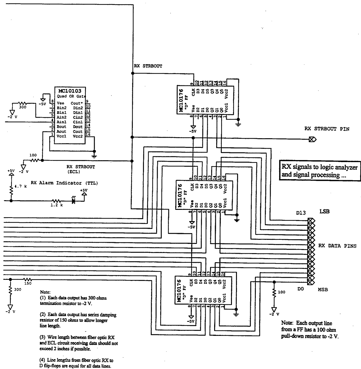
Figure 3.4(b): RX Control Board Schematic.
