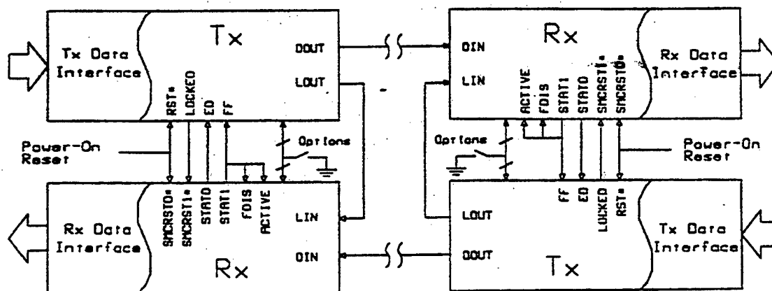
Figure 2.5: G-Link Full-Duplex Configuration [From Reference 14; p. 33].
