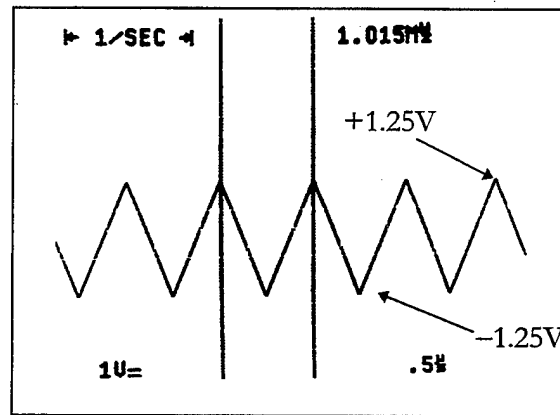
Figure 4.13: 1.015 MHz Triangular Wave ADC Analog Input.
