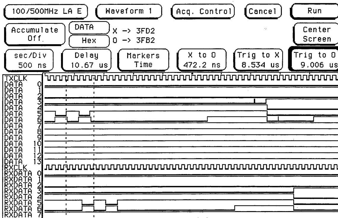
Figure 4.29: Measuring TX to RX Delay on Channel 5 (10 MHz Triangular Wave Input).
