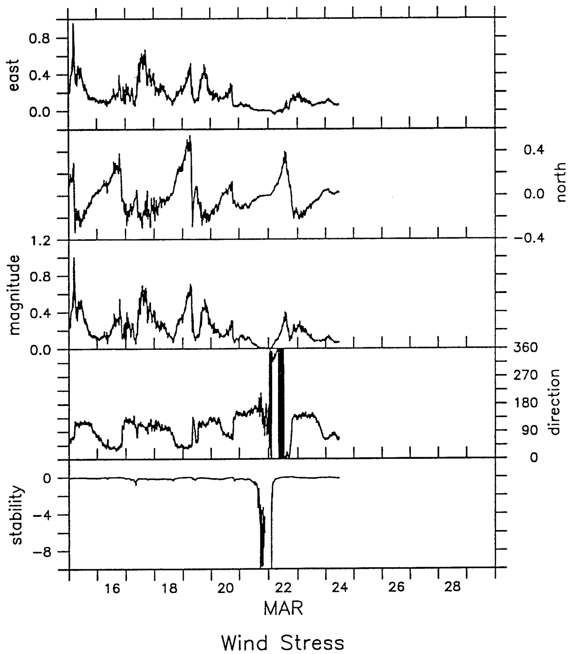
Figure 3.1.21 Wind Stress Time Series from the Composite Data Set.
