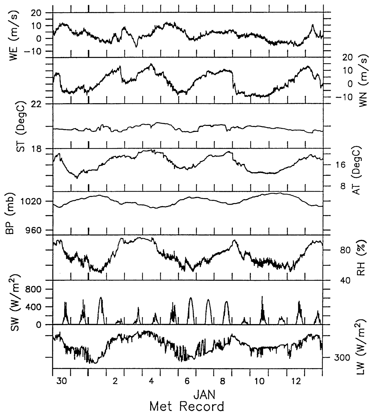
Figure 3.1.2: Meteorological Variables from the Composite Data Set.
