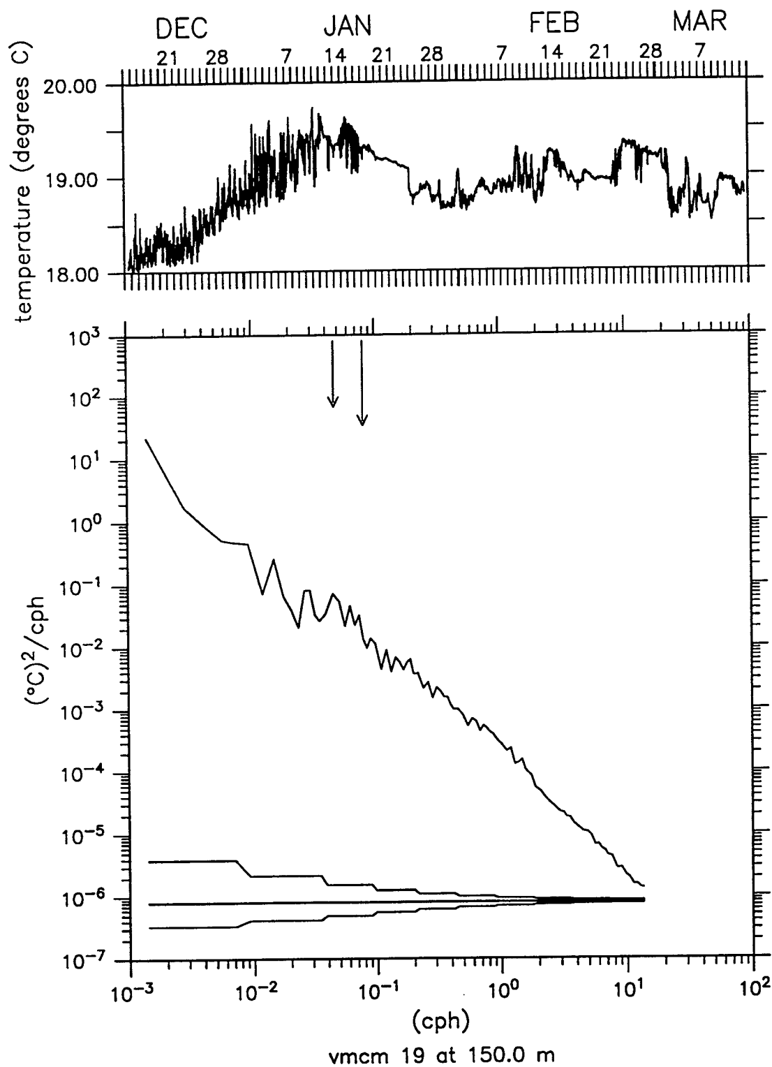
Figure 3.2.14: Temperature Time Series and Spectra at 150m. Long arrow indicates semi-diurnal tidal frequency, short arrow indicates Coriolis frequency.
