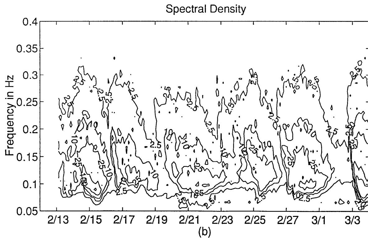
Figure 3.4.5: Spectral evolution of the surface waves. Contours of spectral density as a function of frequency over time. Contours are 2.5, 10, 25, 100, 250.
