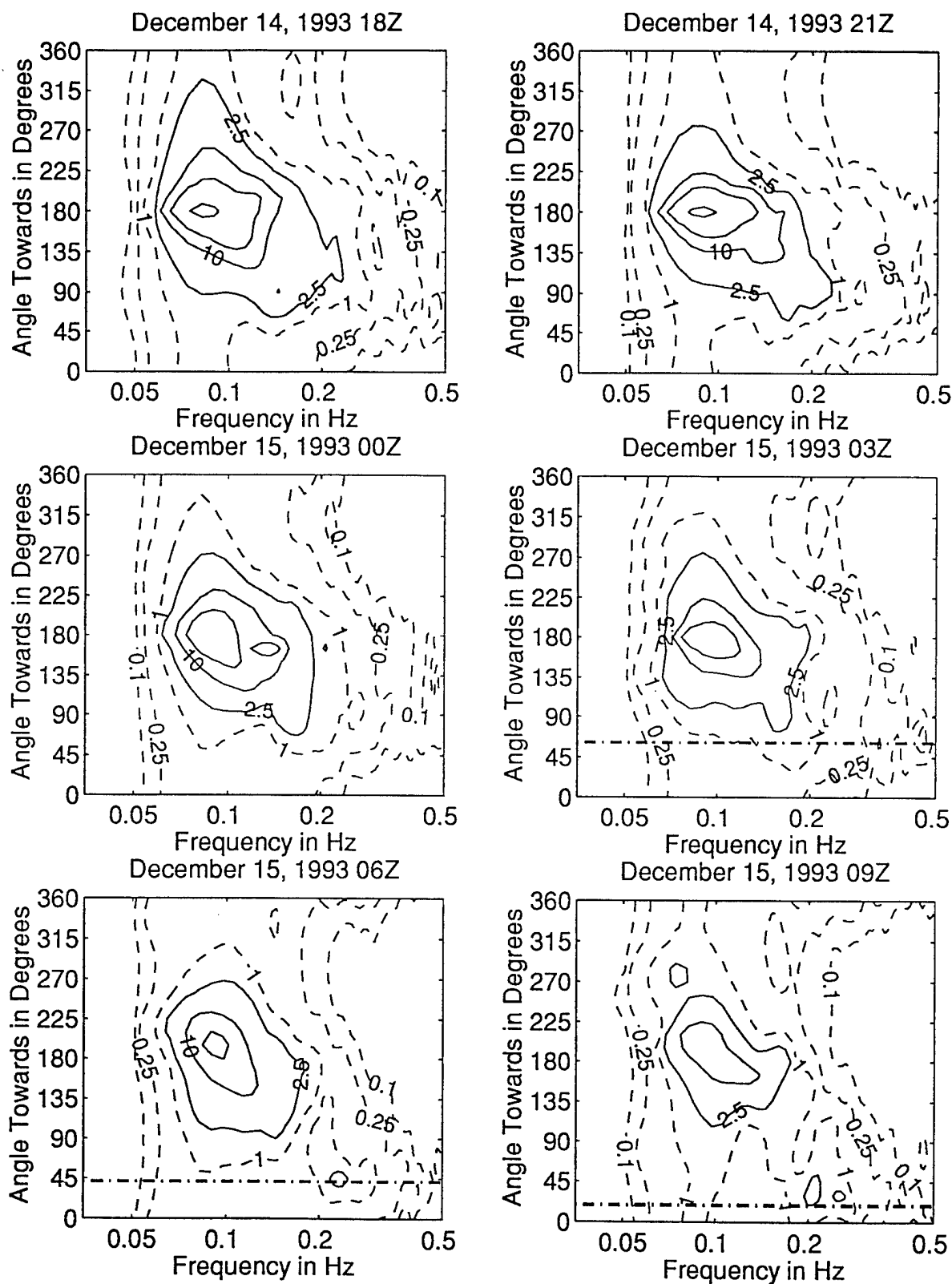
Figure 3.4.11: Directional wave spectra, computed using maximum entropy method. Contours of spectral density as a function of direction. Contours are 0.1, 0.25, 1 (dashed), 2.5, 10, 25, 100, and 250 (solid). Wind direction is shown by thick dashed line.
