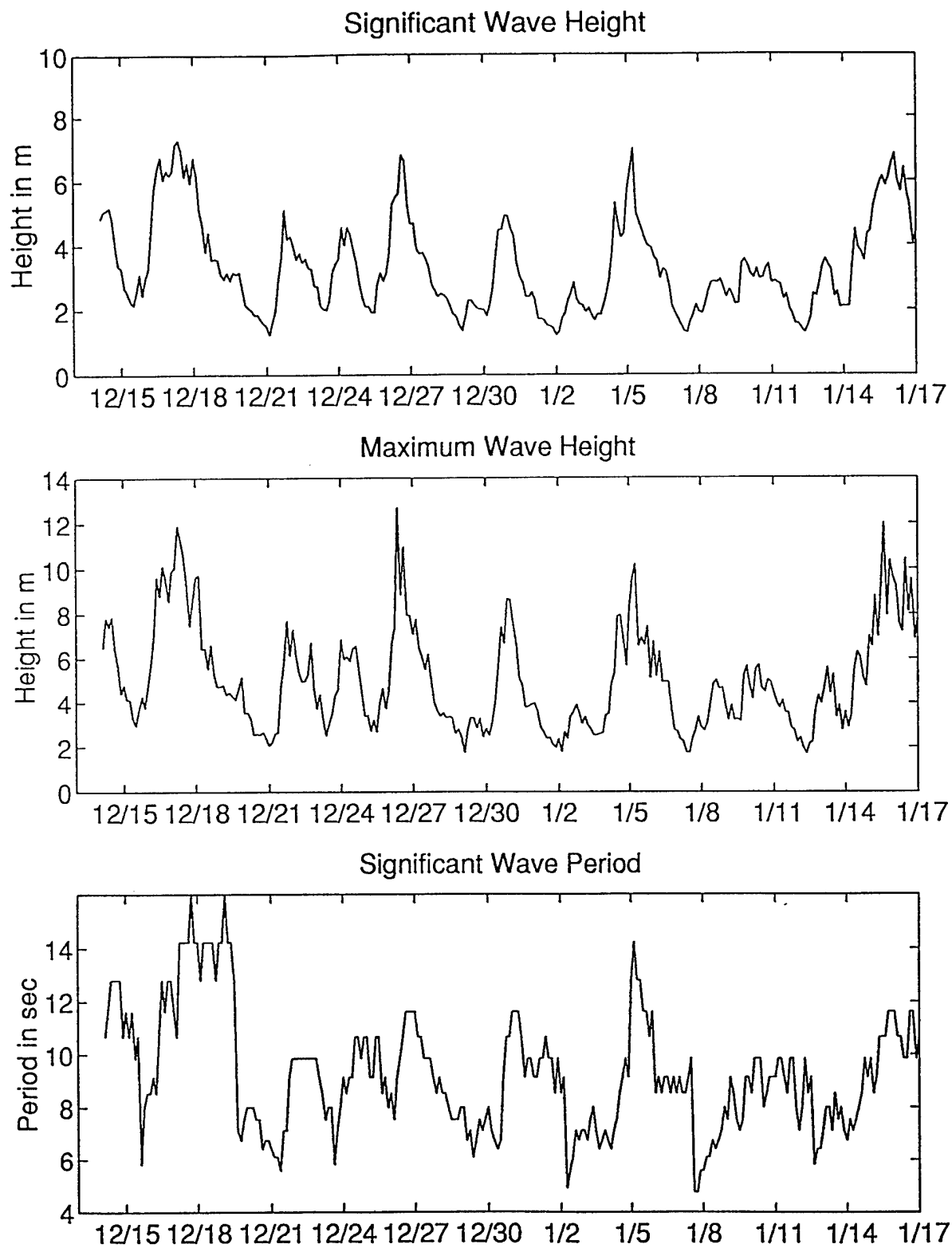
Figure 3.4.1: Nondirectional wave parameters. Significant wave height, maximum wave height, and significant wave period.
