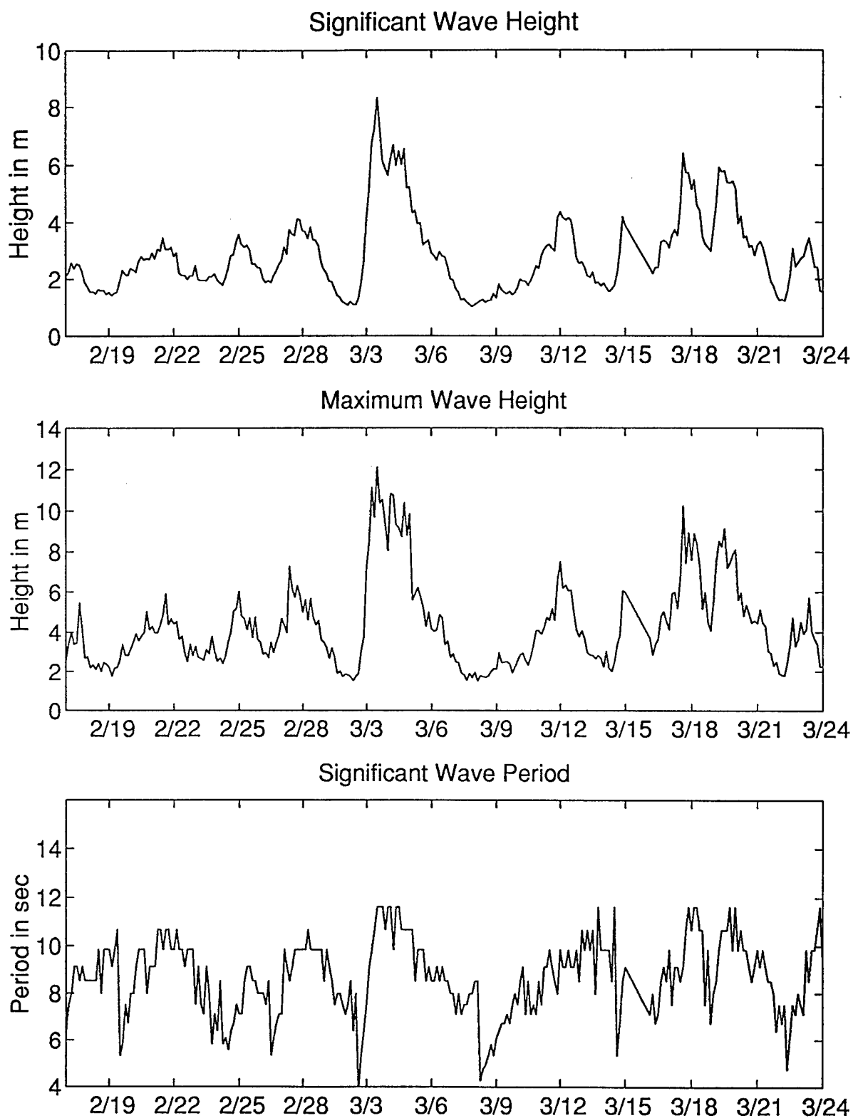
Figure 3.4.3: Nondirectional wave parameters. Significant wave height, maximum wave height, and significant wave period.
