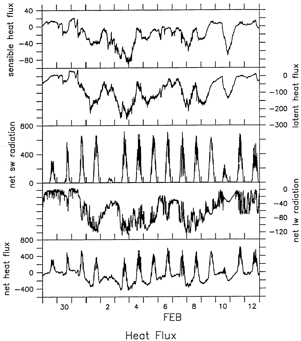
Figure 3.1.11: Heat Flux Time Series from the Composite Data Set.
