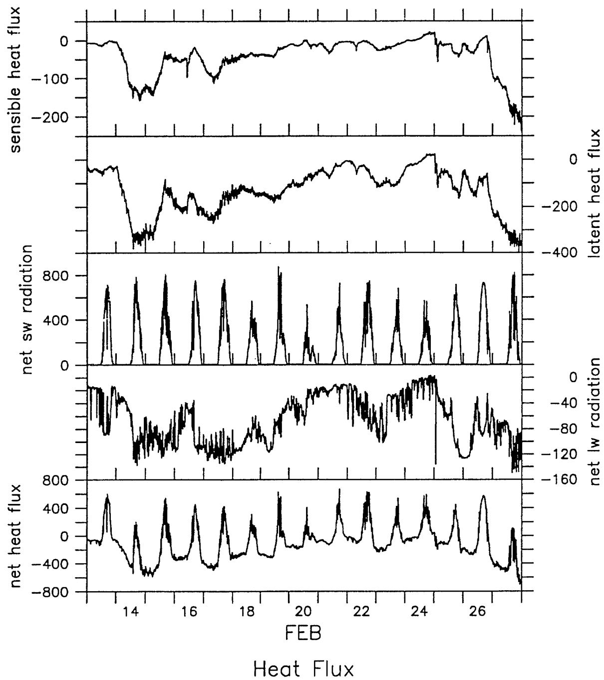
Figure 3.1.12: Heat Flux Time Series from the Composite Data Set.
