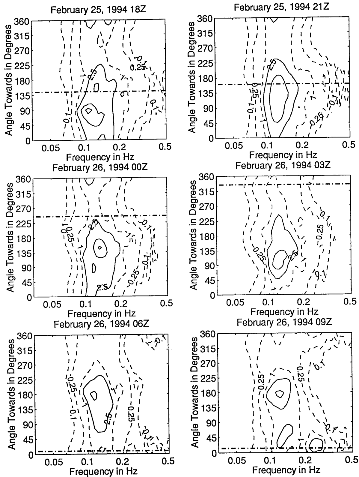
Figure 3.4.107: Directional wave spectra, computed using maximum entropy method. Contours of spectral density as a function of direction. Contours are 0.1, 0.25, 1 (dashed), 2.5, 10, 25, 100, and 250 (solid). Wind direction is shown by thick dashed line.
