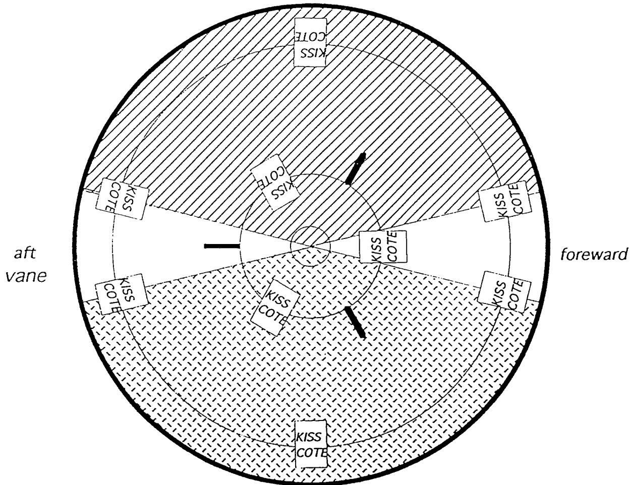
Figure A.3.2: ASREX antifouling paint test. Diagram of hull painting.
