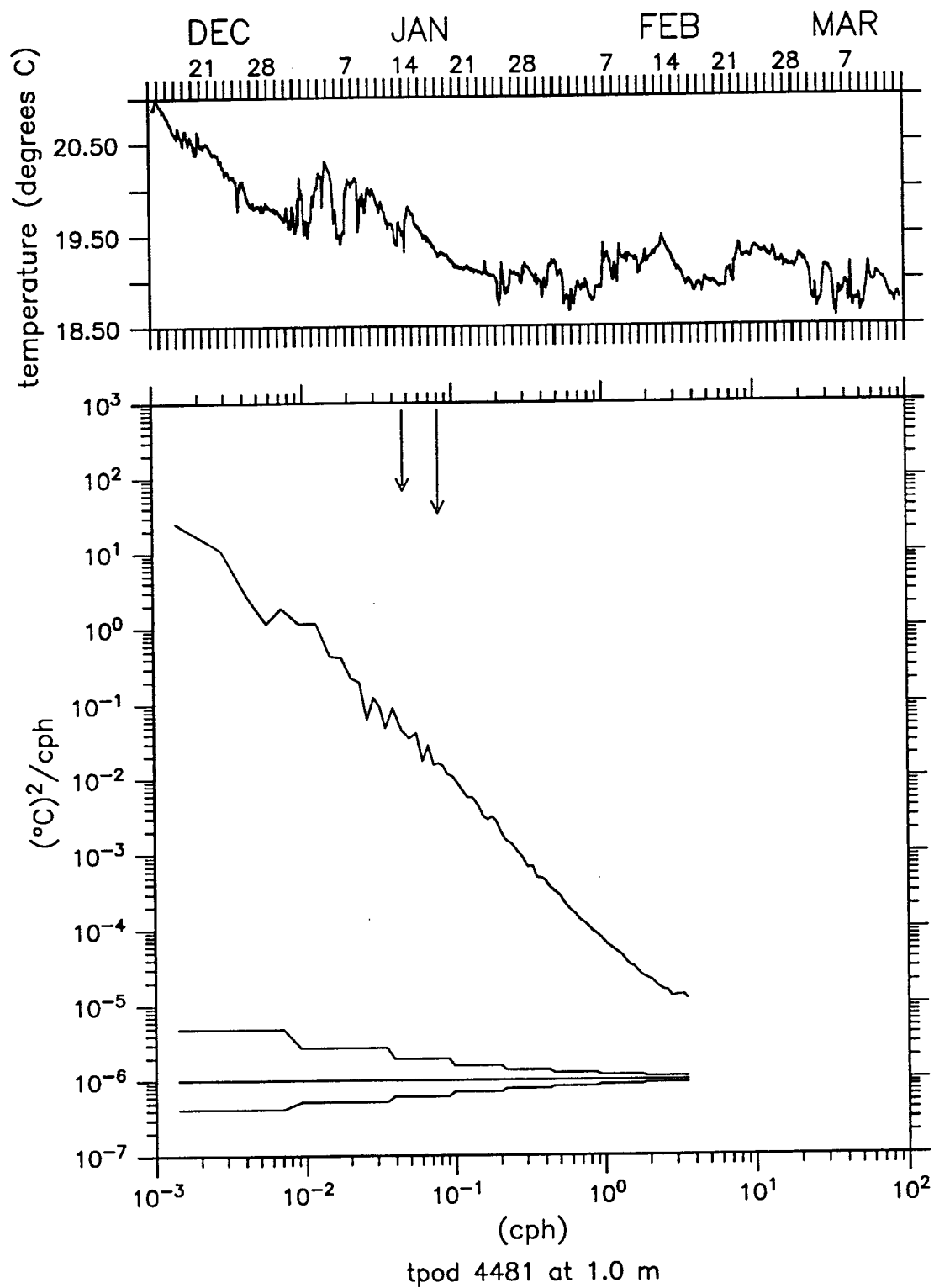
Figure 3.2.2: Temperature Time Series and Spectra at 1m. Long arrow indicates semi-diurnal tidal frequency, short arrow indicates Coriolis frequency.
