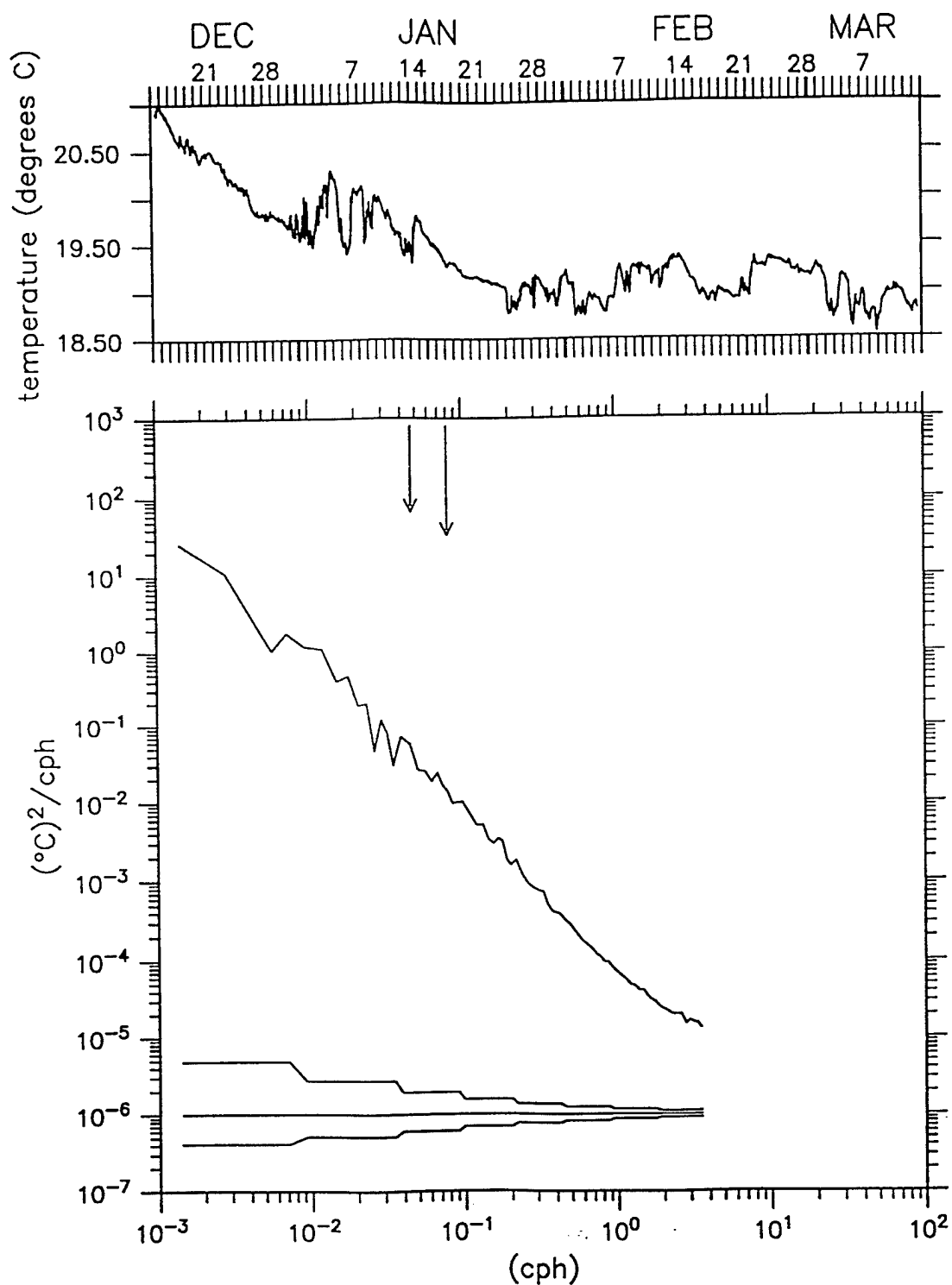
Figure 3.2.9: Temperature Time Series and Spectra at 37m. Long arrow indicates semi-diurnal tidal frequency, short arrow indicates Coriolis frequency.
