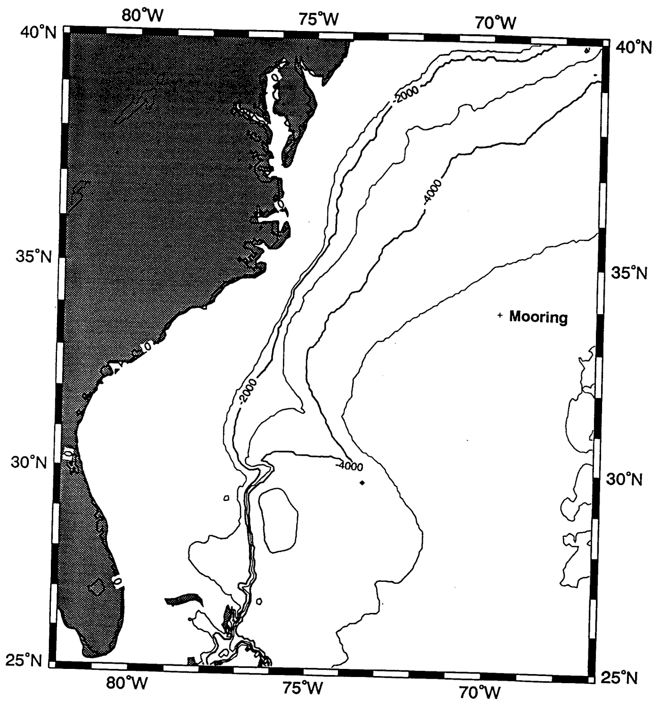
Figure 2.1: Bathymetric map of experiment site.
