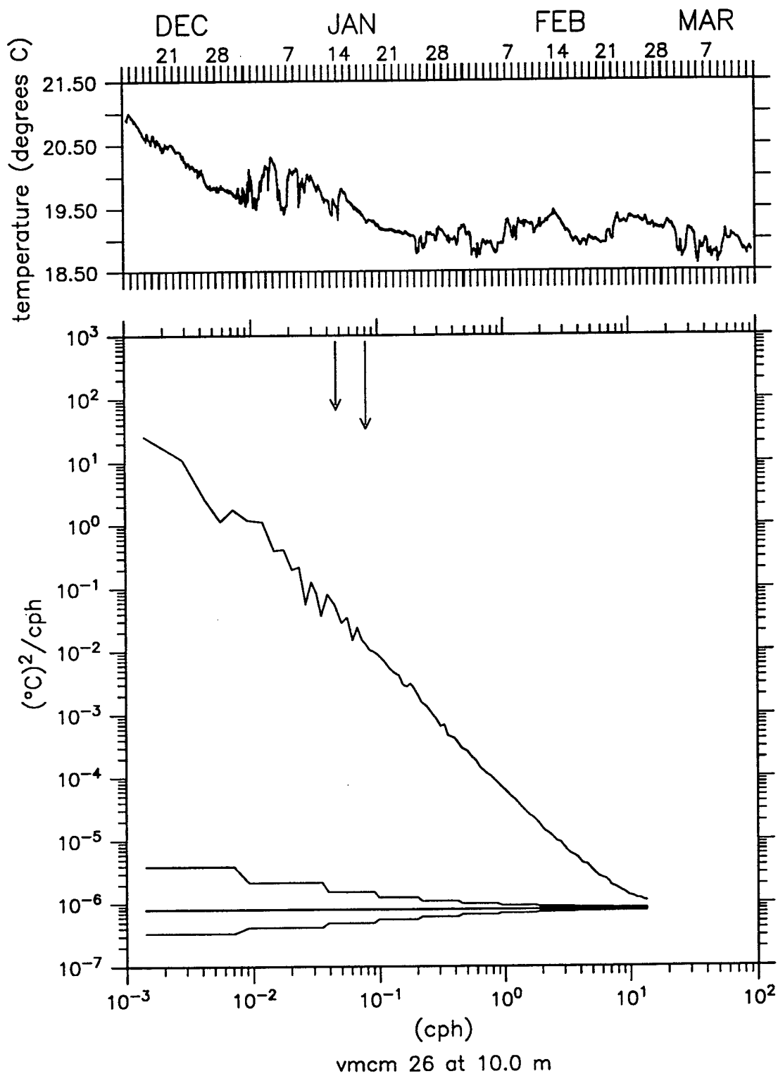
Figure 3.2.6: Temperature Time Series and Spectra at 10m. Long arrow indicates semi-diurnal tidal frequency, short arrow indicates Coriolis frequency.
