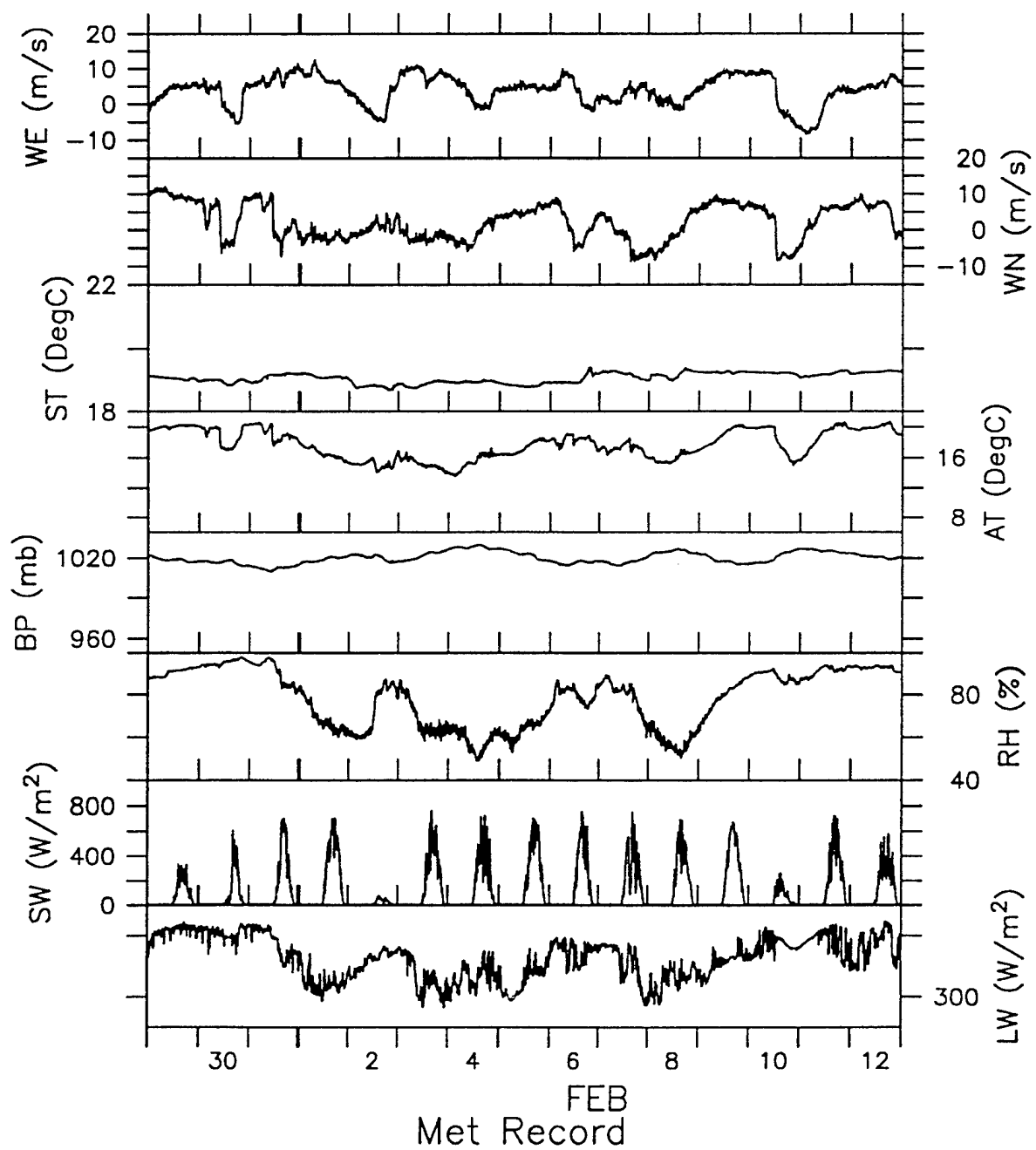
Figure 3.1.4: Meteorological Variables from the Composite Data Set.
