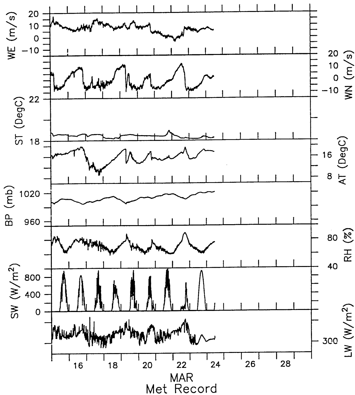
Figure 3.1.7: Meteorological Variables from the Composite Data Set.
