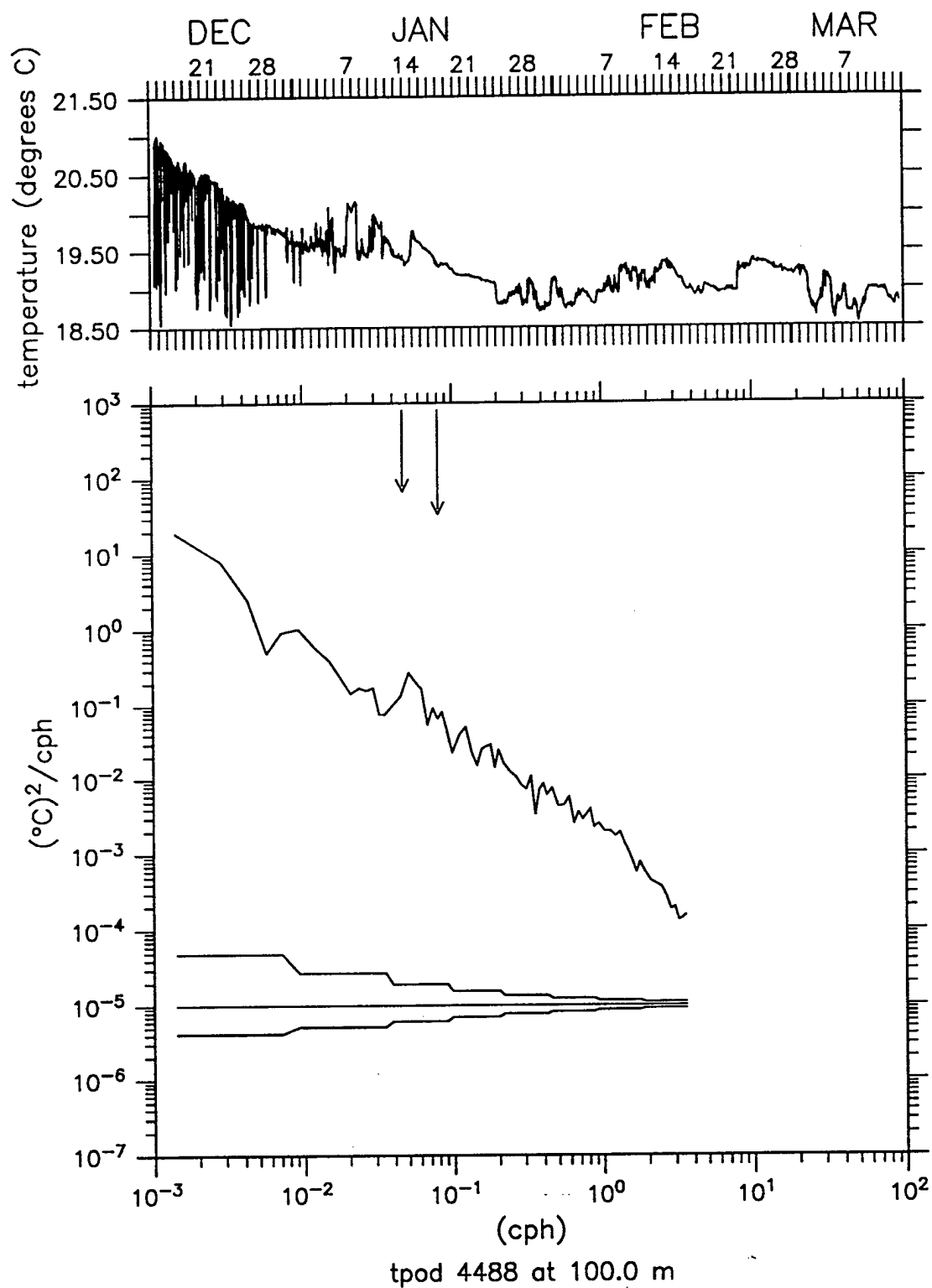
Figure 3.2.12: Temperature Time Series and Spectra at 100m. Long arrow indicates semi-diurnal tidal frequency, short arrow indicates Coriolis frequency.
