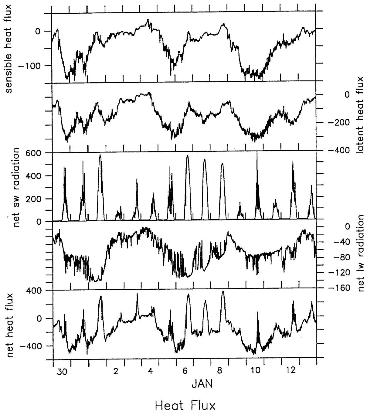
Figure 3.1.9: Heat Flux Time Series from the Composite Data Set.
