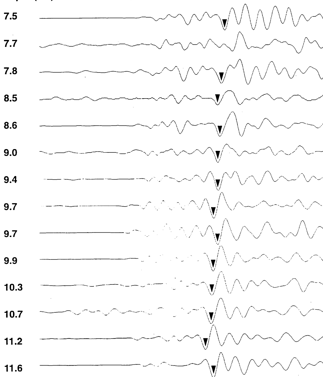
Figure 3-1. Seismograms and phase picks (arrows) from station HTW plotted in order of increasing hypocenter depth. Depths (in km) are listed to the left of the traces. Traces are: bandpassed at 1 to 3 Hz with a two pole Butterworth filter; 6 seconds in length; amplitude normalized; and aligned according to calculated P_g arrival times using a velocity of 6.0 km/s.
