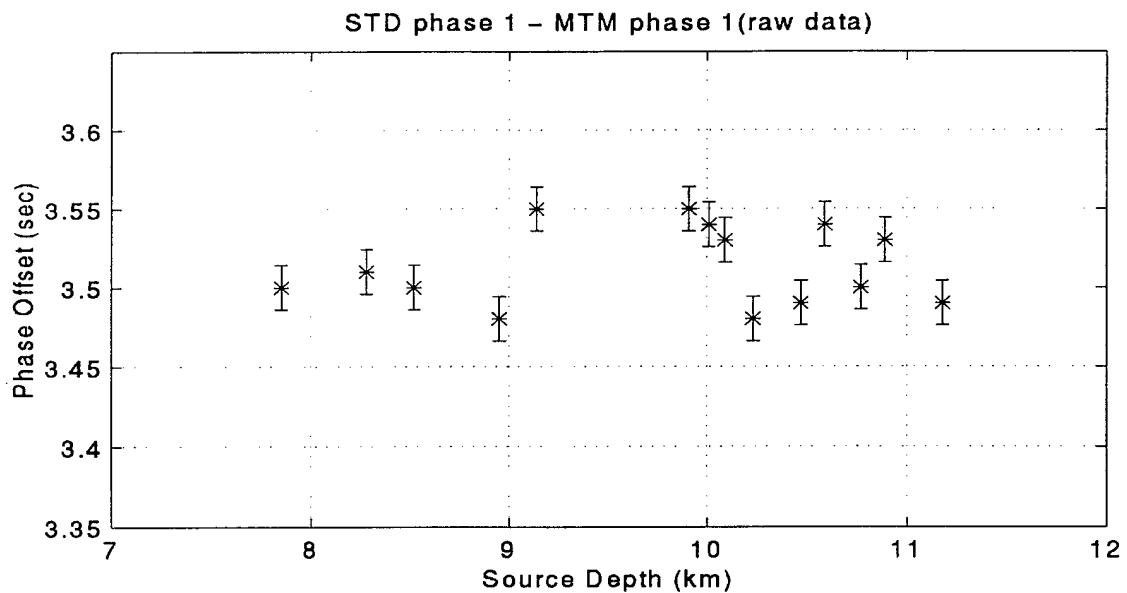
Figure 4-5. Phase offset plots between station STD and station MTM for 15 select events in the Scotts Mills sequence. The top plot has been corrected for inter-station epicentral shift, bottom shows uncorrected data. Error bars represent a standard deviation of \pm 0.014 s. Notice no clear change in offset times relative to depth. Probably, the same phase has been picked at each station.
