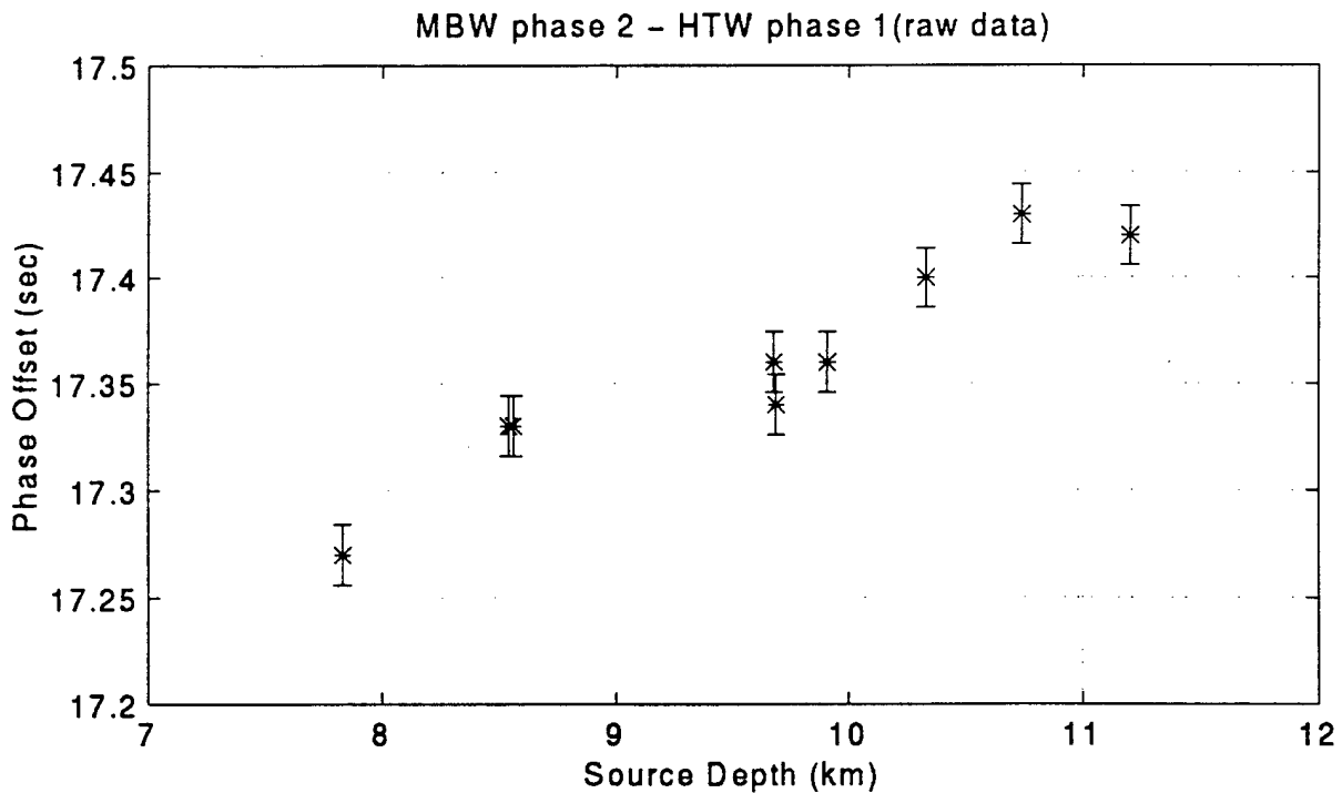
Figure 3-7. Phase offset plots between station MBW phase 2 and station HTW phase 1, corrected for epicentral shift (top) and uncorrected raw data (bottom). Error bars represent a standard deviation of \pm 0.014 s. Notice clear linear depth-dependent trend where phase offset increases with depth.
