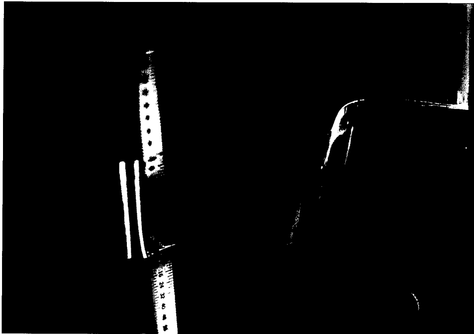
Figure 3-32 Demonstration of simultaneous two-color (He:Ne laser and argon laser) coupling and propagation in a single flexible ( 2.5\ \mu\text{m} ) polymer waveguide film.
