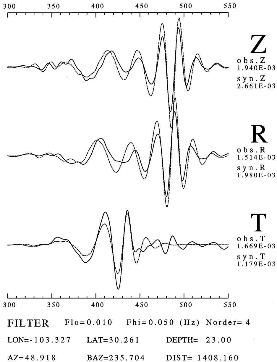
Fig. 5.18a. The waveform fit of the fine-tuning model shown at figure 5.17. Three different frequency ranges are shown: (a) 0.01-0.05 Hz.
