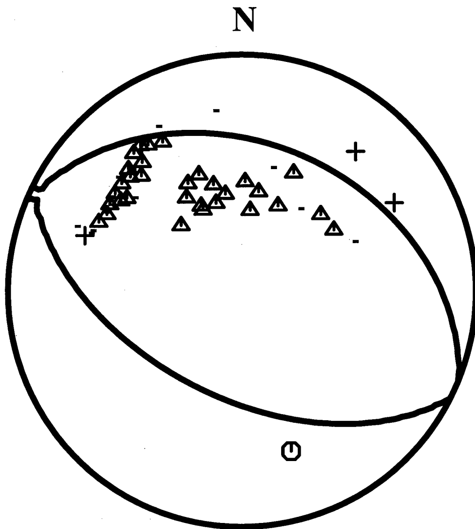
Fig. 2.10. This figure shows the focal mechanism of Harvard CMT solution and the observed P-wave polarities.
