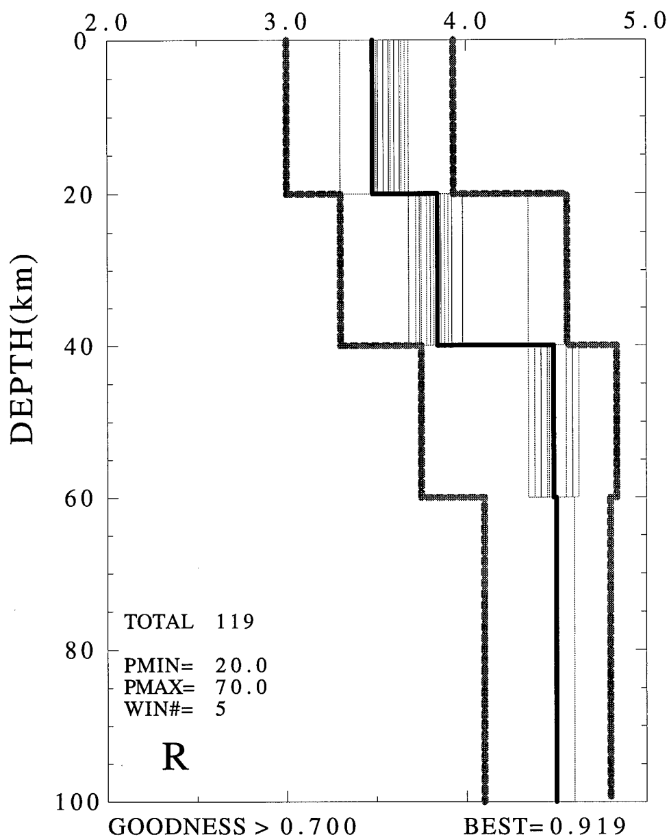
Fig. 4.14. The GA searched models for HRV.
