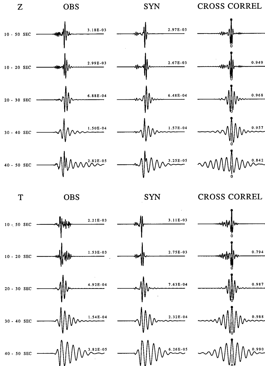
Fig. 4.9a. For TUC, the cross-correlations for the observed and synthetic seismograms which were generated using GA searched models. (a) The synthetics were computed using the best models from separated searched models for Love and Rayleigh wave (Figures 4.6ab).
