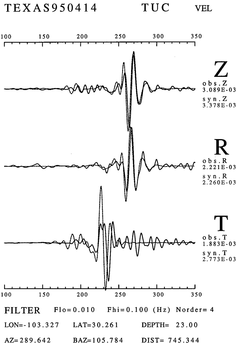
Fig. 4.8b. (cont'd). (b) The predicted seismograms were generated using the best model from a joint search for both Love and Rayleigh wave (Figure 4.7).
