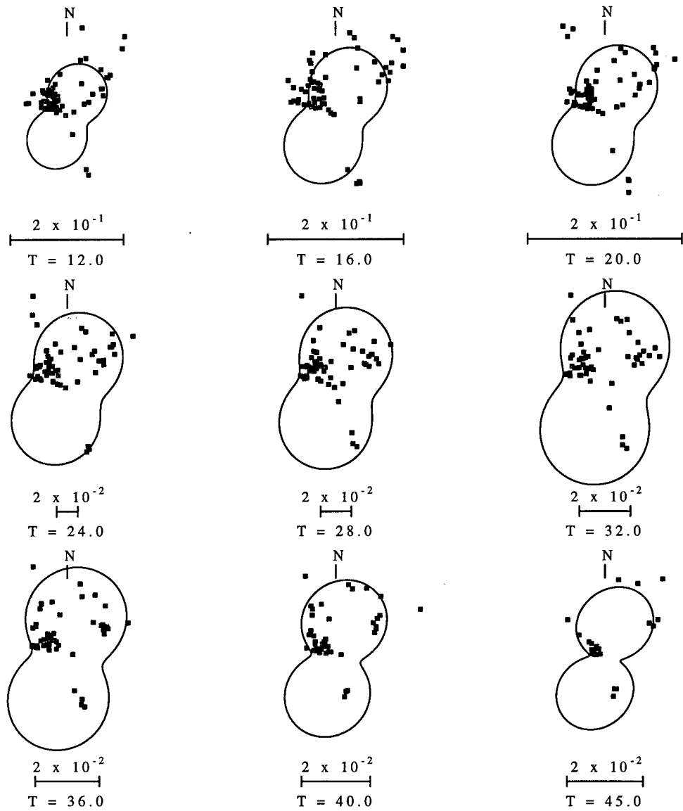
Fig. 2.6. The Rayleigh wave radiation patterns for the preferred focal mechanism at 23 km depth.
