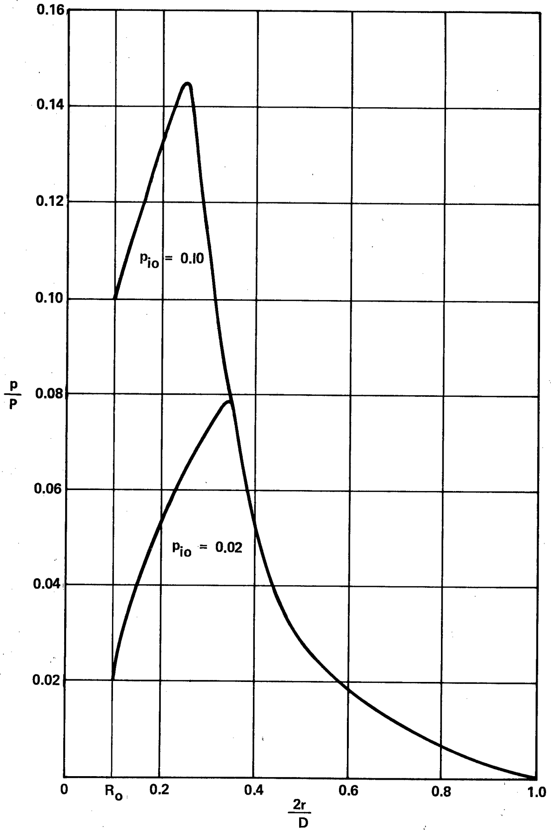
Figure 3. Surface Pressure Distributions for HR = 1,000 p_{i0} = 0.02 and 0.1
