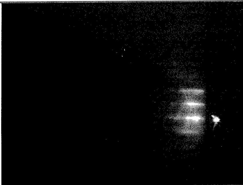
Figure 7 RHEED reconstruction for a sapphire substrate prior to growth of GaN.
