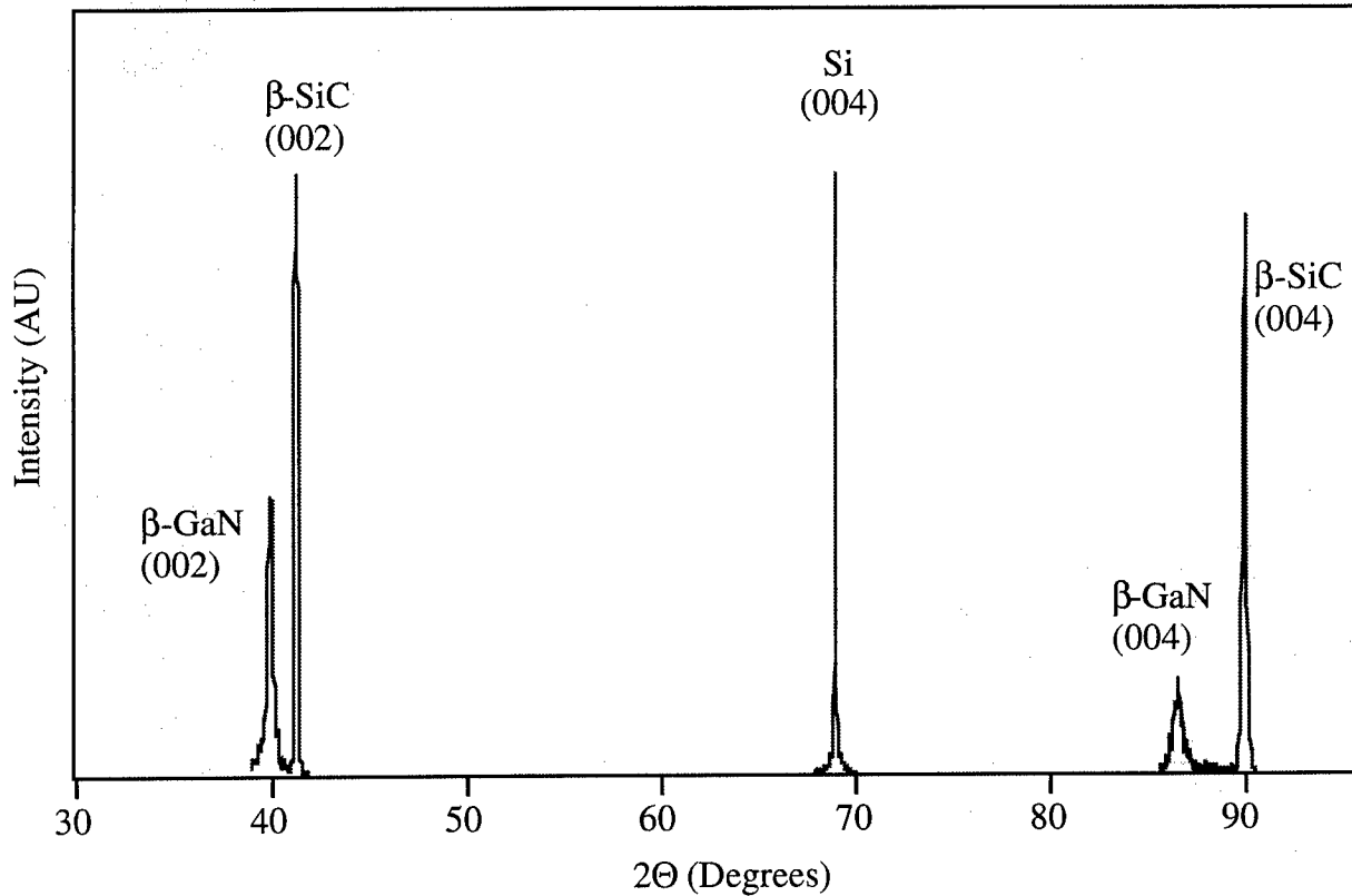
Figure 17 X-ray diffraction of 0.2 \mu m thick cubic GaN grown on SiC at Cornell at 600W RF power
