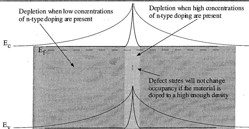
Figure 14 Model of band diagram surrounding vertically oriented defect in GaN which shows Fermi-level pinning at the defect level and band bending away from the defect.
