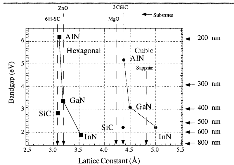
Figure 1 Bandgaps for Wurtzite and cubic III-nitrides
