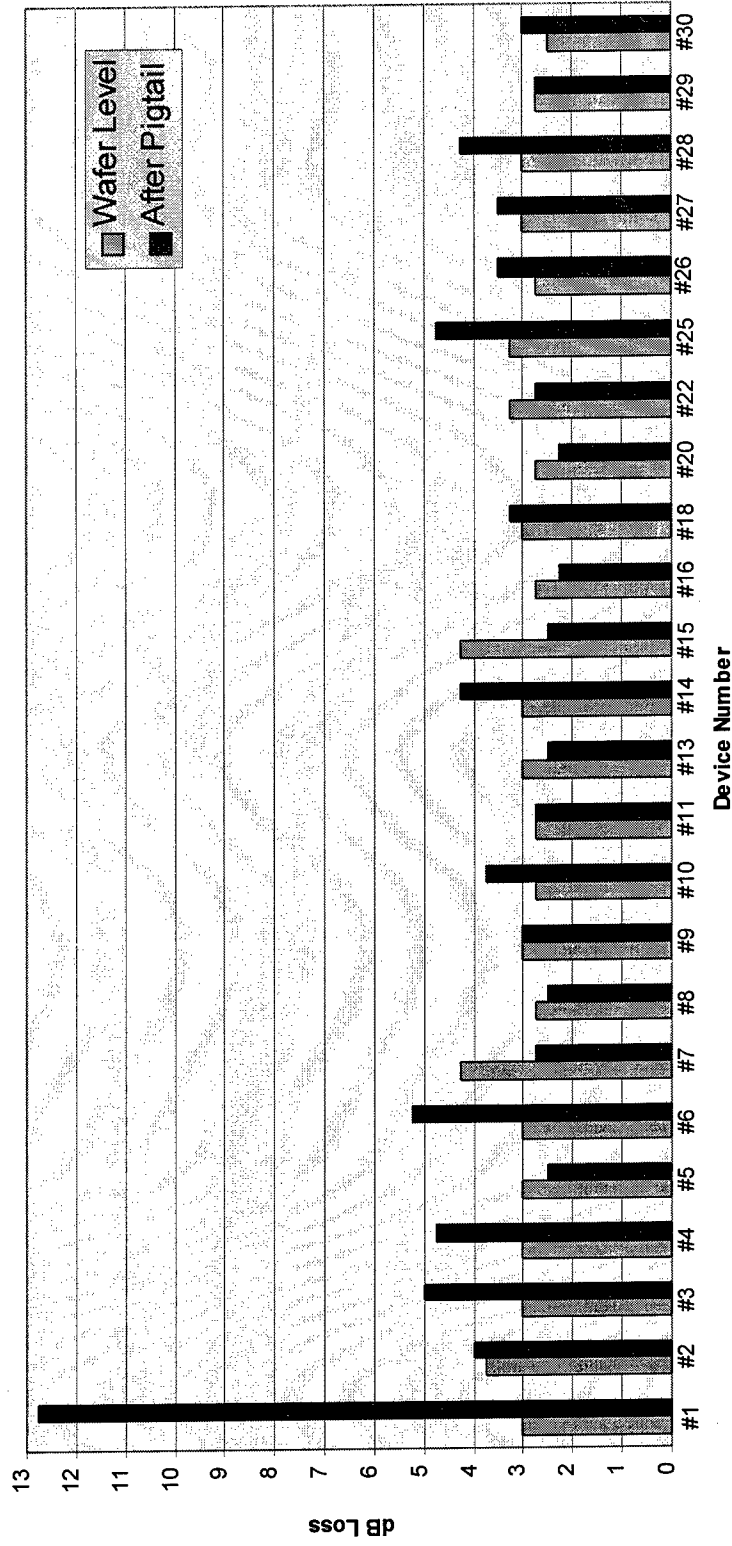
Figure 5: Comparison Loss
