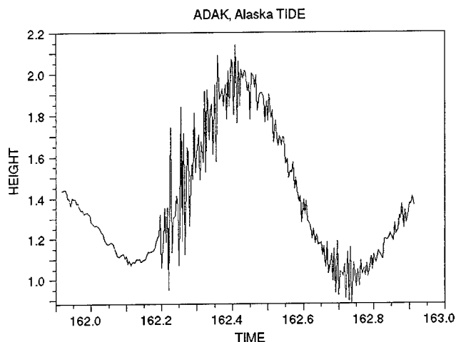
Record of the two June 10, 1996 tsunamis recorded on the tide gauge at Adak, Alaska. The time scale on the bottom of the record is in UTC Julian days. This graph was downloaded as a file in a standard graphics format from the WC/ATWC web site
