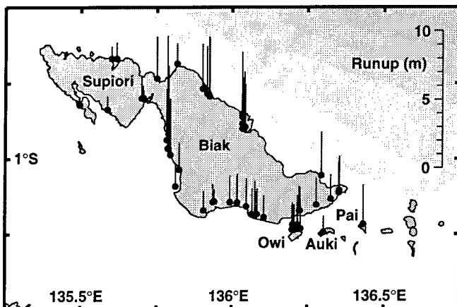
Runup measurements (dot = measurement location, vertical line = runup height) made by the international survey team following the February 17, 1996 tsunami in Irian Jaya, Indonesia. A small discrepancy between measurement locations reported by the team and the coastal database used to produce the underlying map causes certain data points to appear slightly inland or offshore.
