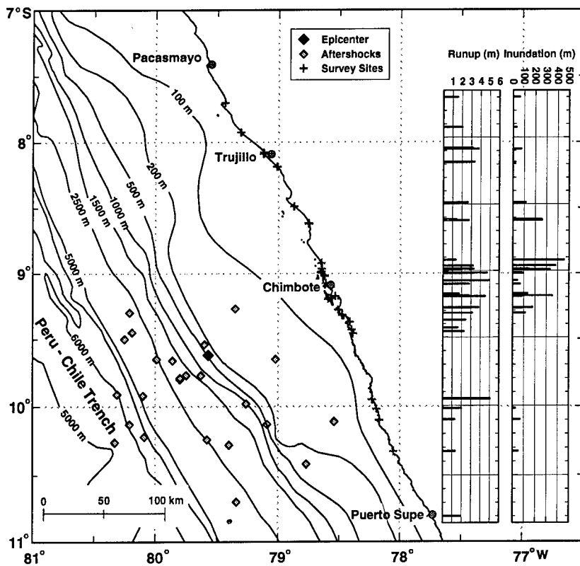
Runup and inundation measurements along the coast of central Peru for the tsunami of February 21, 1996 generated by a strong earthquake located southwest of Chimbote.
