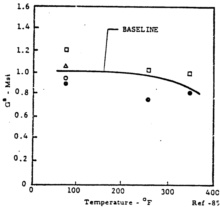
FIGURE 3-10 EFFECT OF VARIOUS HUMIDITY TREATMENTS ON LONGITUDINAL AND SHEAR ELASTIC PROPERTIES from Reference 2
