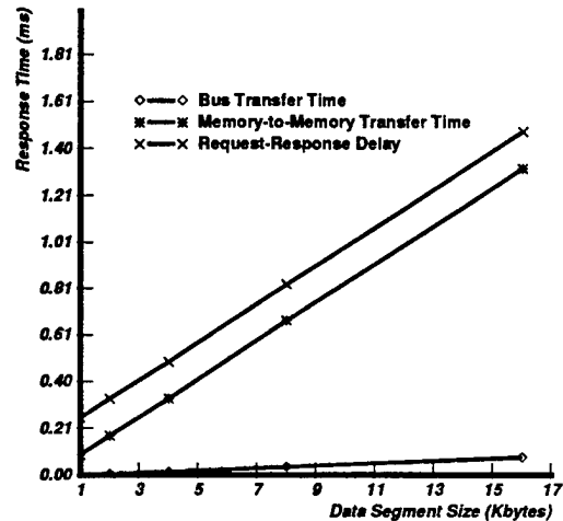
Figure 5.4: Response time for NAB using a 20-MIPS processor.
