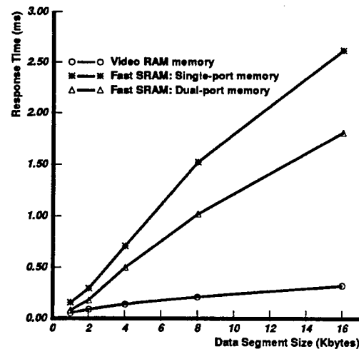
Figure 5.8: Response times of NAB with various memory organizations.
