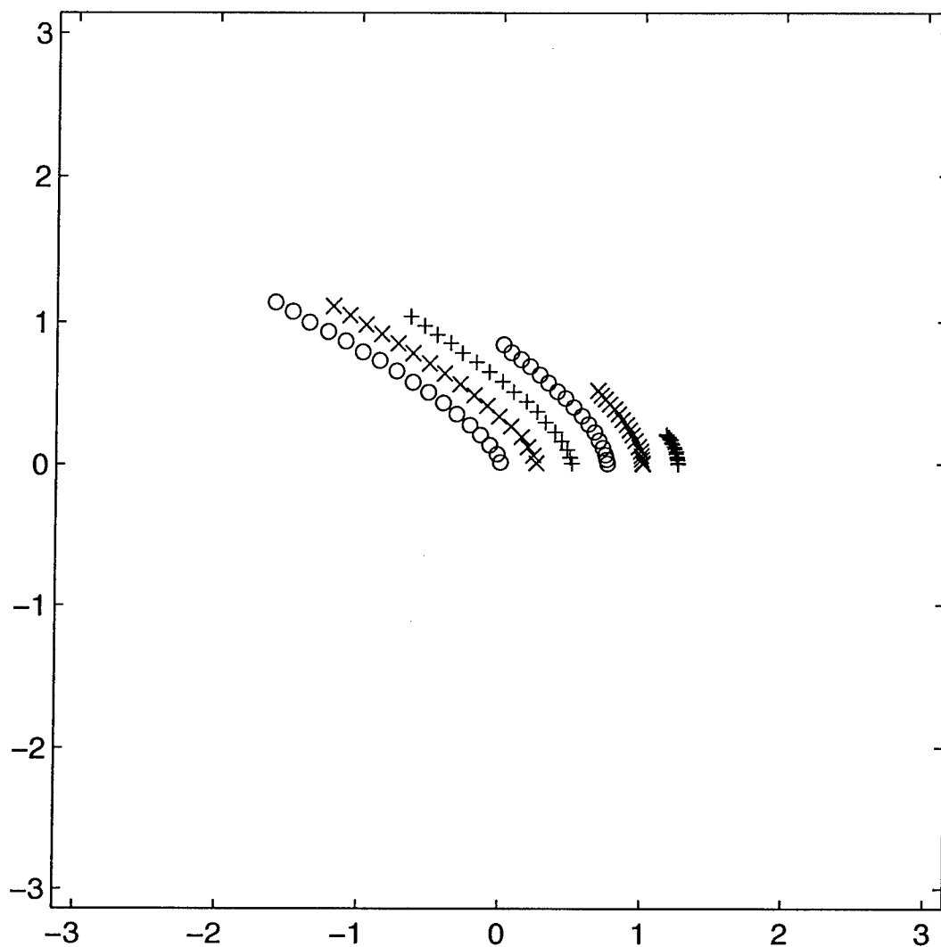
Figure 3.39: Non-isolated, surface-trapped potential vortex tracks with \frac{\beta_2 r_0^2}{U_1} = .009 . The tracks from left to right correspond to sizes r_0 = .9\lambda , .64\lambda , .45\lambda , .32\lambda , .23\lambda , .16\lambda , . . Positions are indicated every 3 time units.
