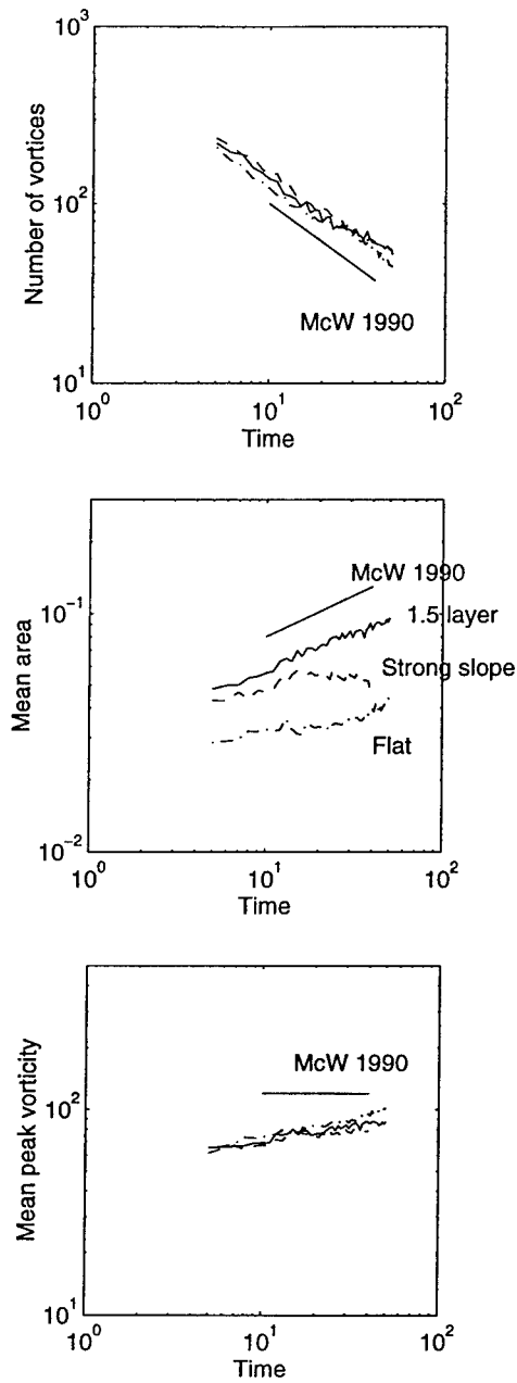
Figure 4.20: Vortex statistics for strong slope cases. Runs shown are the flat bottom case (dash-dot), the \Lambda = .1 case (dashed) and the one and a half layer case (solid). Vortices are connected regions with q_1 > 10 .
