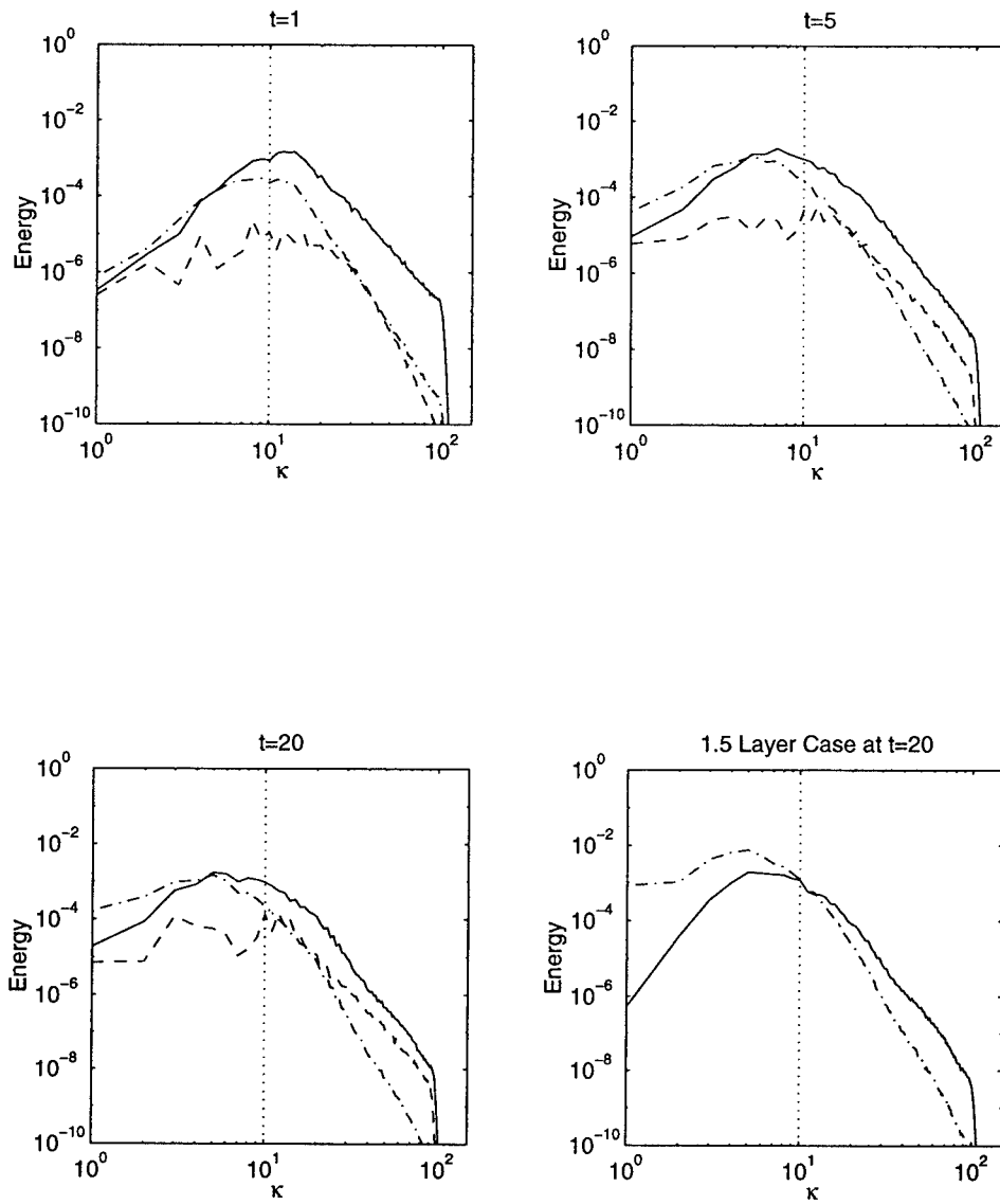
Figure 4.14: The energy spectra for the strong slope case and the one and a half layer case (lower right). The components are KE_1 (solid), KE_2 (dashed) and PE (dash-dot). The spectra have been averaged in unit wavenumber bins from [\kappa - .5, \kappa + .5) .
