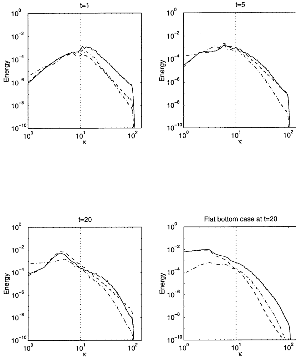
Figure 4.5: The energy spectra for the weak slope and flat bottom (lower right) cases. The components are KE_1 (solid), KE_2 (dashed) and PE (dash-dot). The spectra have been averaged in unit wavenumber bins from [\kappa - .5, \kappa + .5) .
