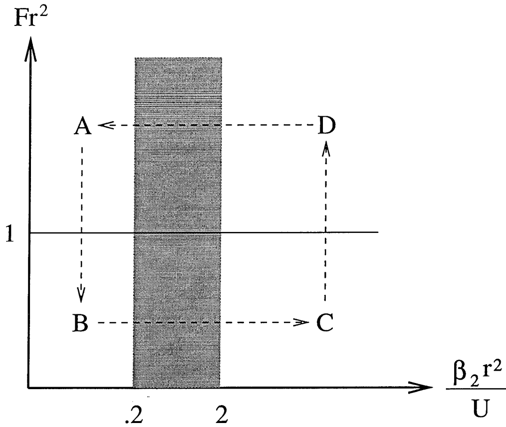
Figure 3.7: The two-layer parameter space. The x-axis is the non-dimensional slope parameter, and the y-axis is the (squared) ratio of vortex radius to the deformation radius. The cases A, B, etc. are labeled in order of appearance in the text.
