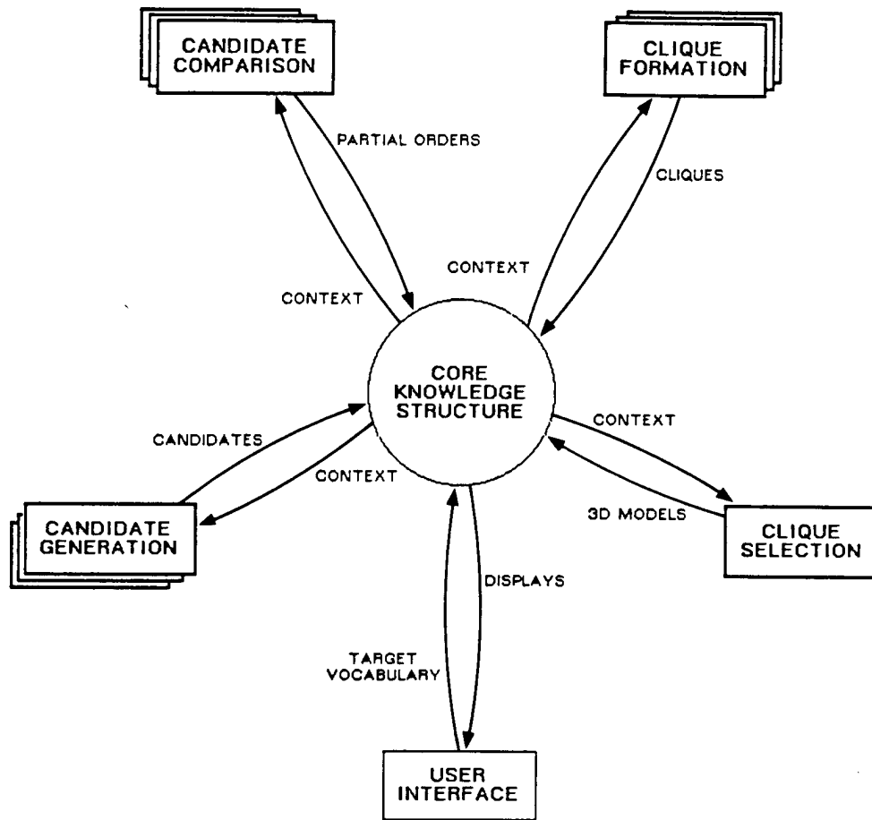
Figure 4.1: Conceptual architecture of Condor.
