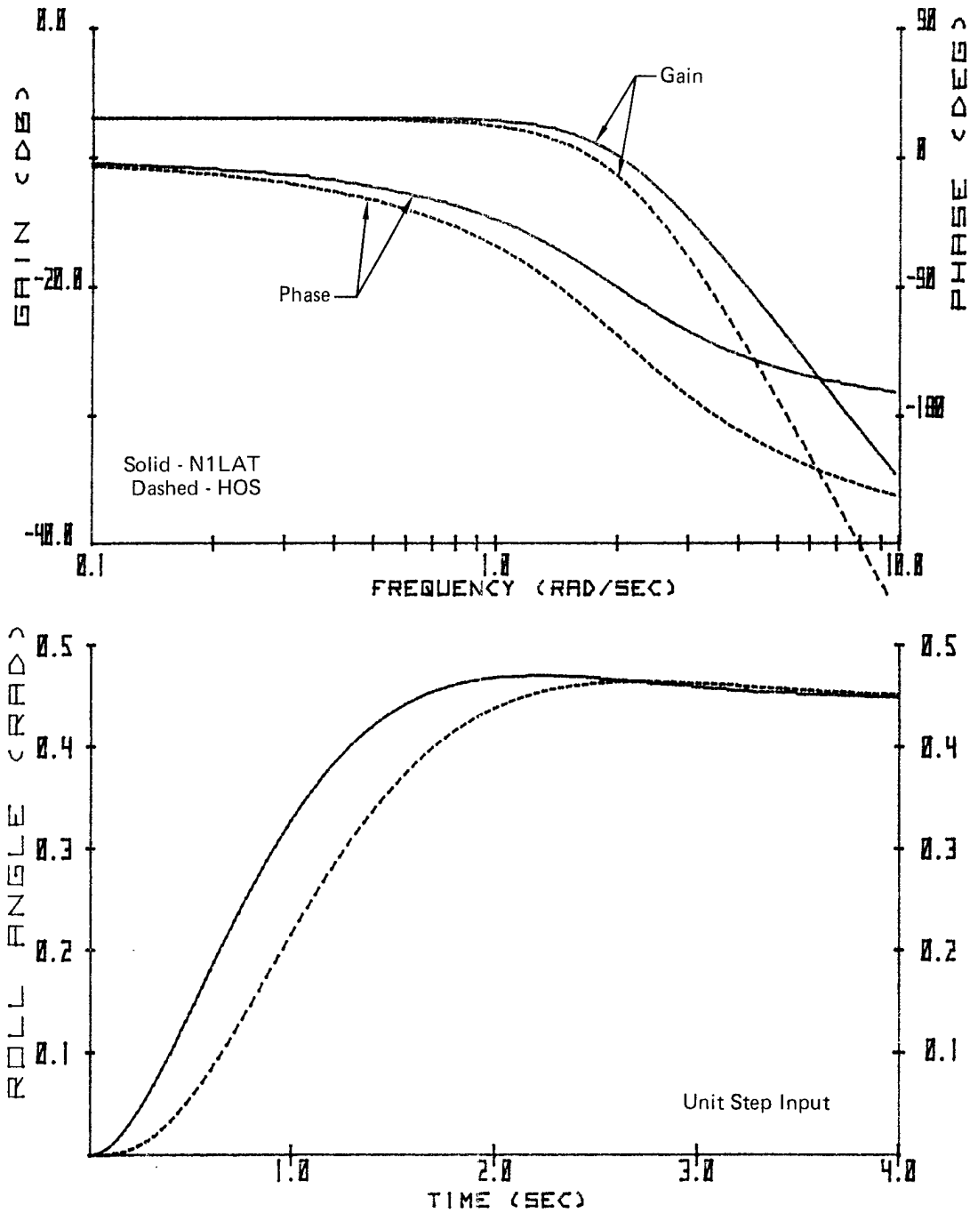
Figure A-6. Frequency and Time Response
