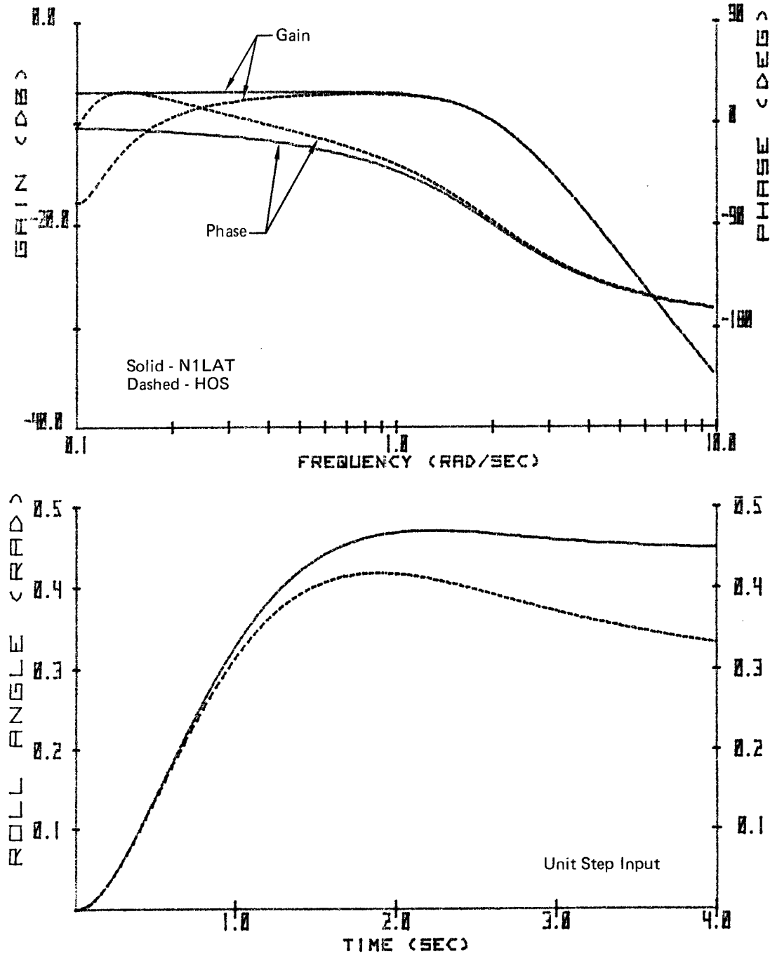
Figure A-23. Frequency and Time Response
