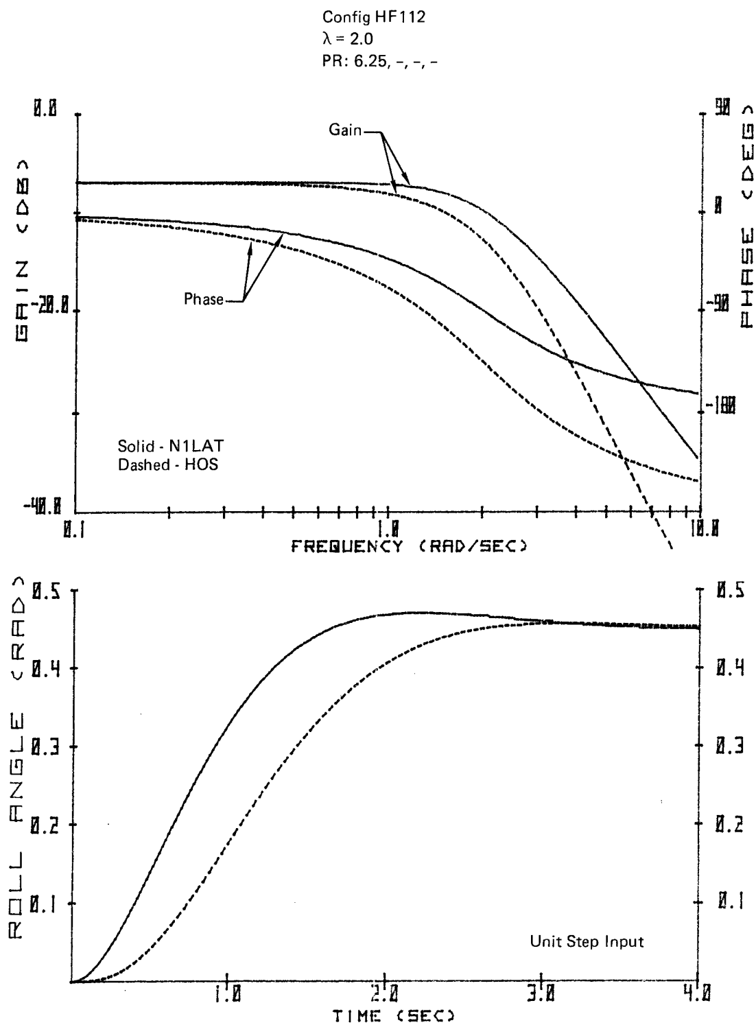
Figure A-5. Frequency and Time Response
