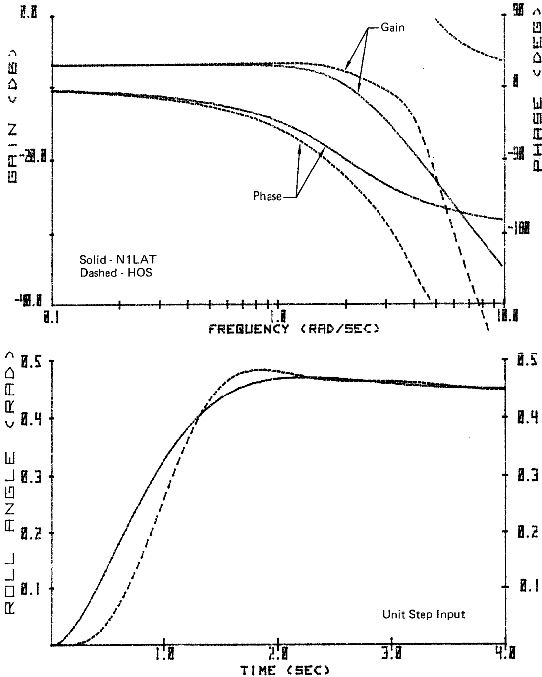
Figure A-11. Frequency and Time Response
