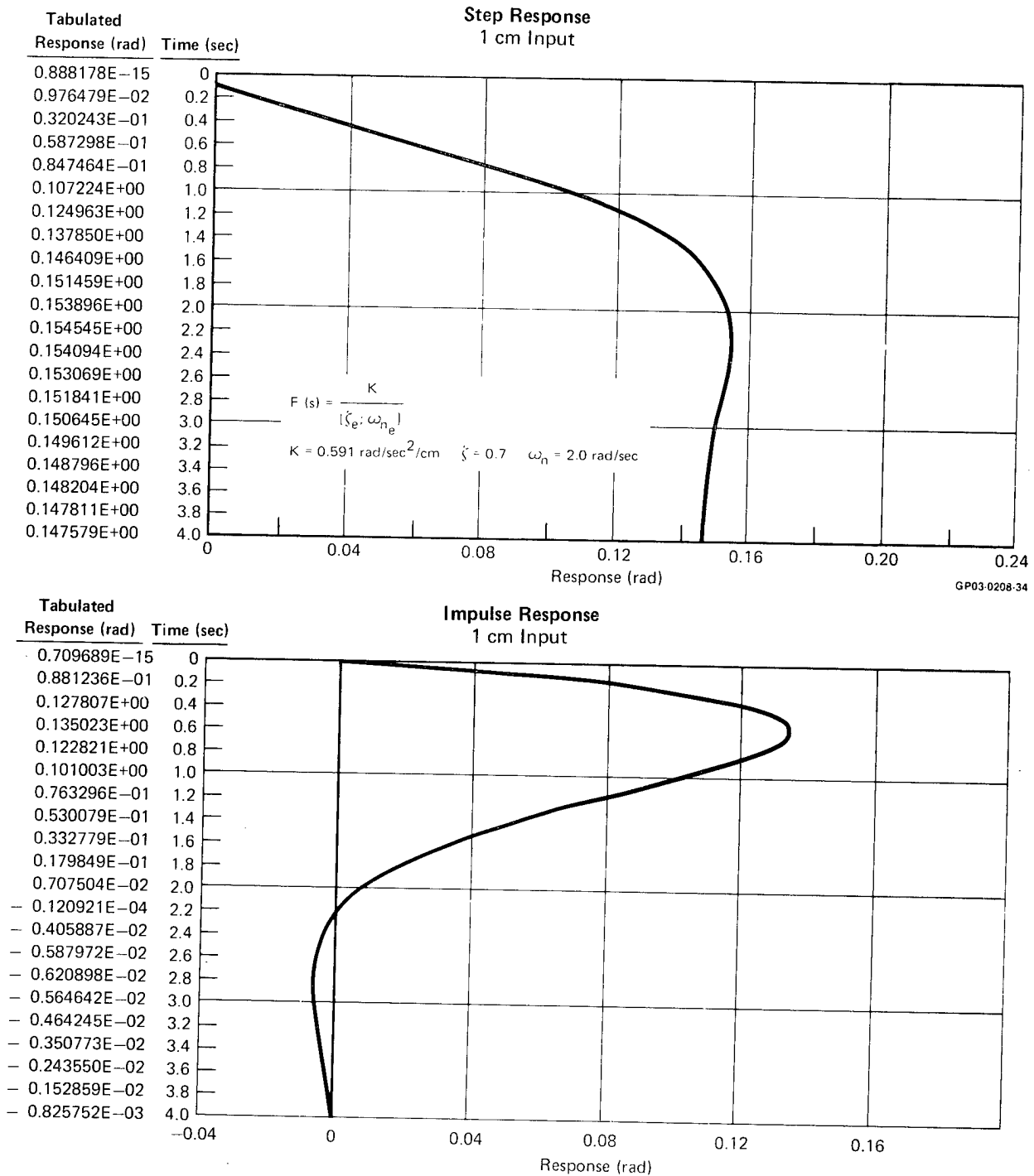
Figure 7. Longitudinal Dynamics, \theta I_{\delta ST}
