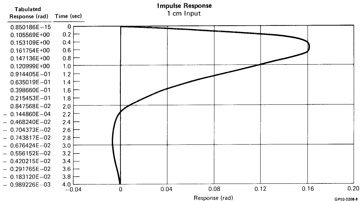
Figure 5. Lateral Dynamics, \phi/\delta_{ST} N1LAT
