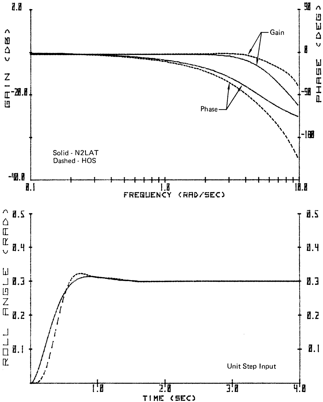
Figure A-40. Frequency and Time Response
