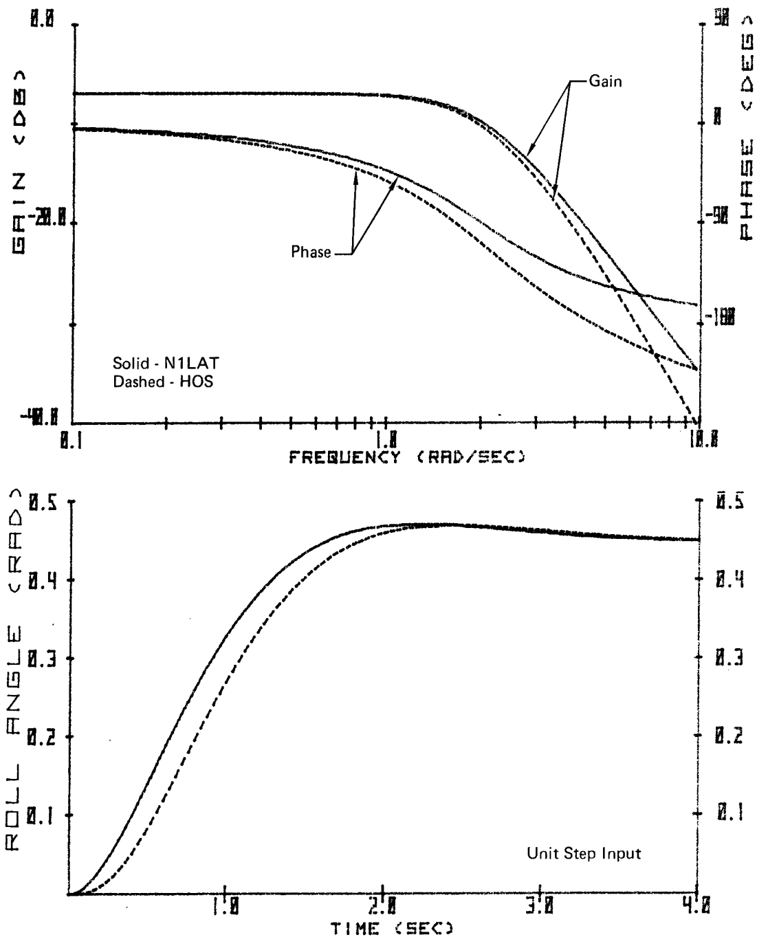
Figure A-9. Frequency and Time Response
