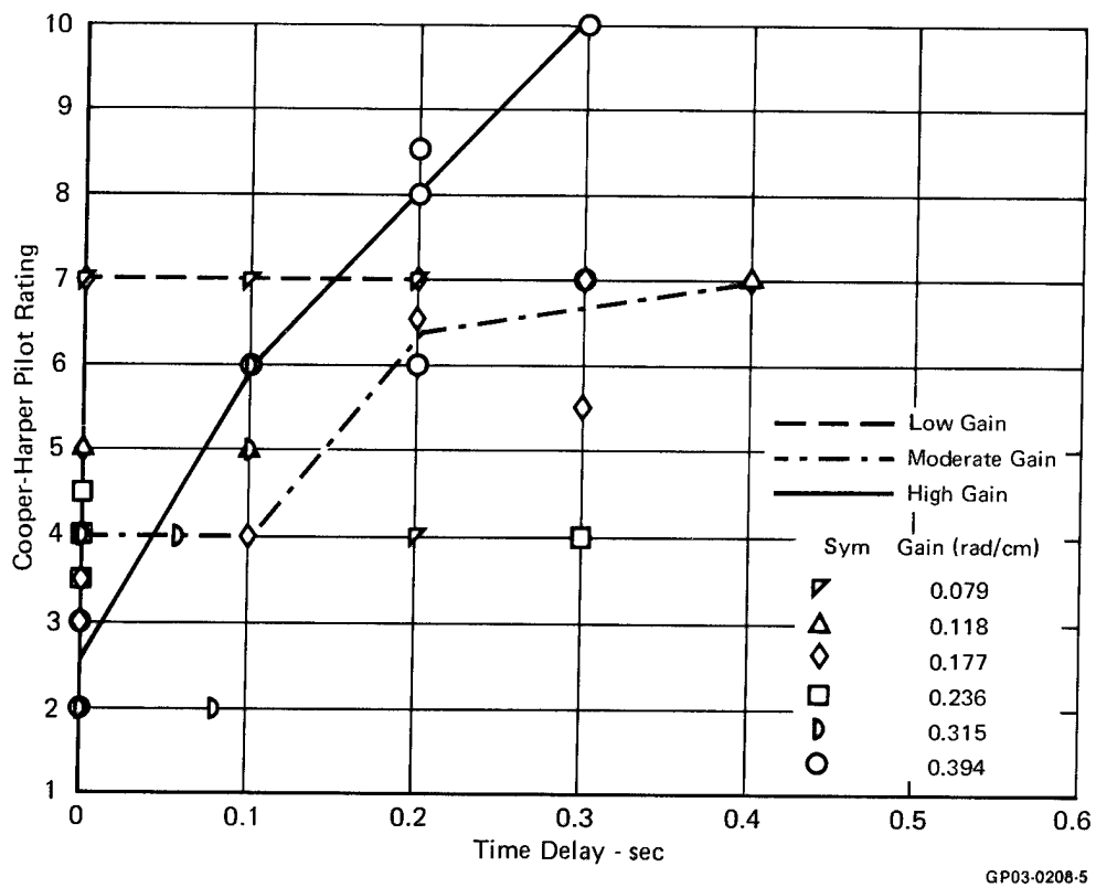
Figure 28. Interaction of Command Gain and Time Delay Baseline Dynamics: [0.7; 2.0]
