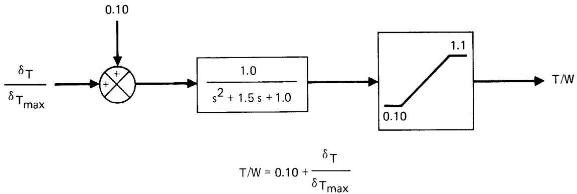
Figure 9. Thrust-to-Throttle Dynamics
