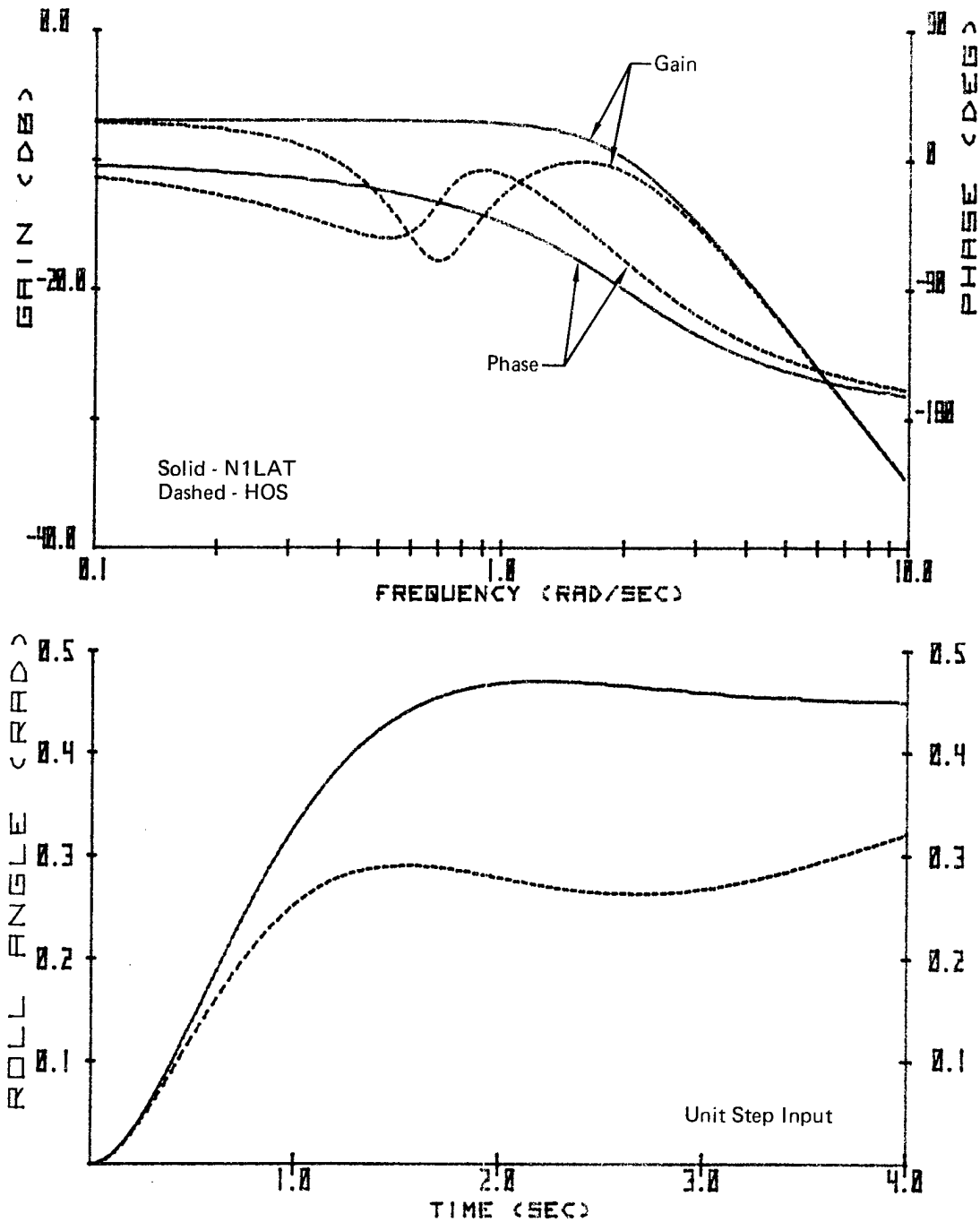
Figure A-26. Frequency and Time Response
