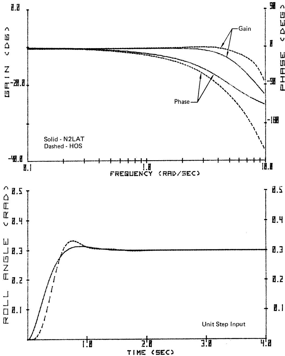
Figure A-39. Frequency and Time Response
