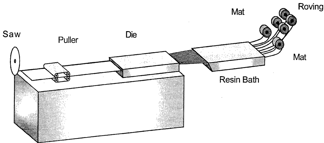
FIGURE 32. PULTRUSION
