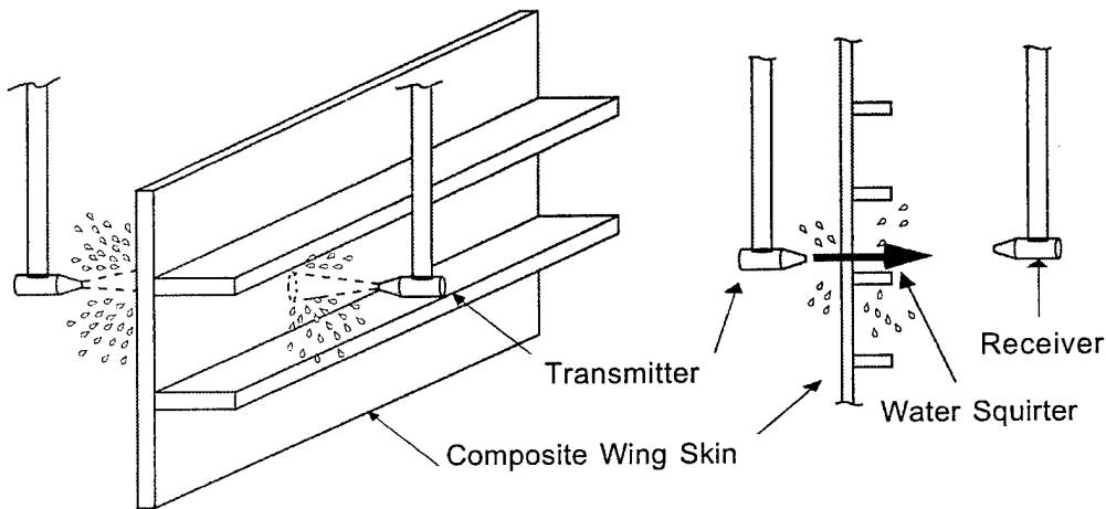
FIGURE 51. ULTRASONIC TESTING
