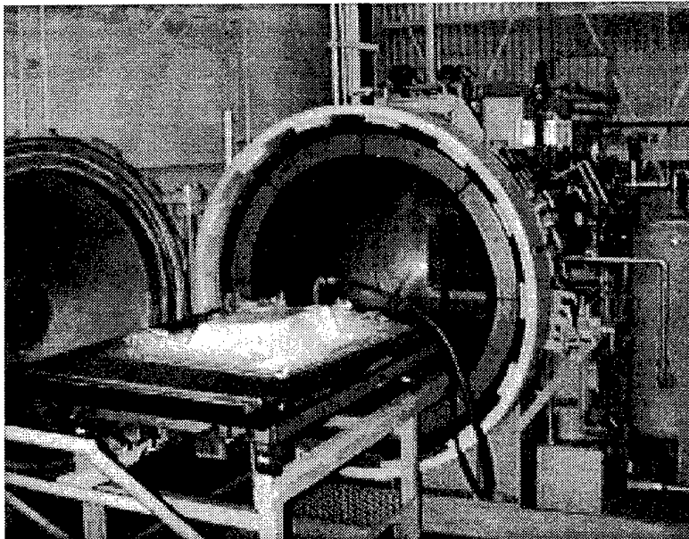
FIGURE 33. AUTOCLAVE
