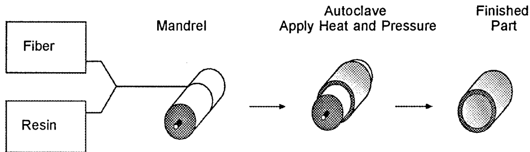
FIGURE 29. FILAMENT WINDING
