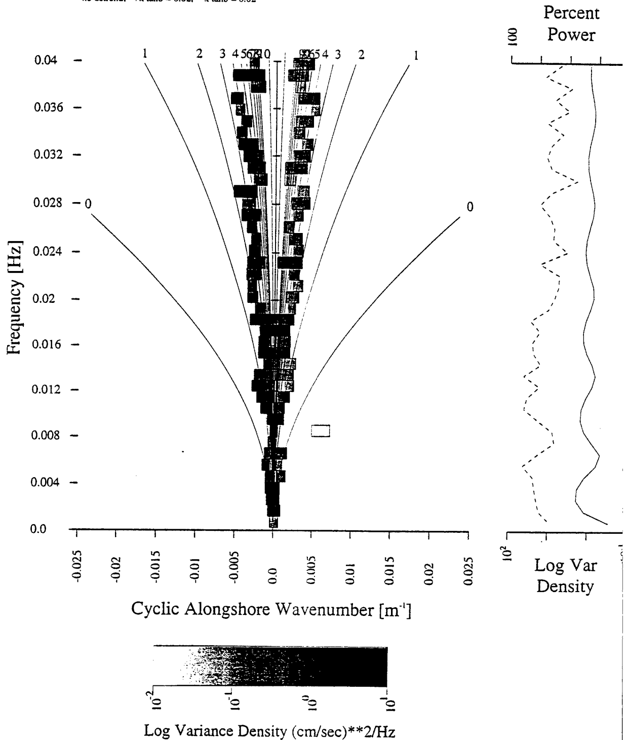
Figure 1.1.3-5. Simulated k-f spectrum for a beach of slope 0.02 and observation depth of 5m.
