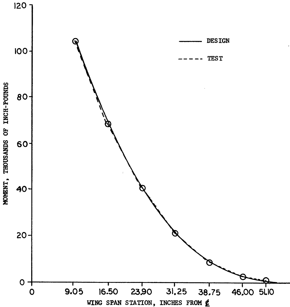
FIGURE 4 - WING LIMIT BENDING MOMENT
