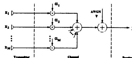
Fig. 1: Fading channel with M transmit antennas.
