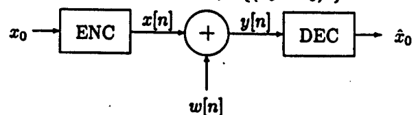
Figure 1. Joint Source-Channel Coding of a Uniform Source over an AWGN Channel
