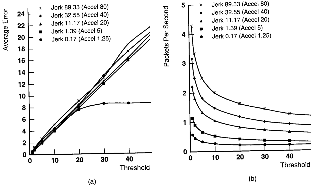
Figure 8: Average History-Based Protocol (a) Error and (b) Packet Rate for Circular Motion
