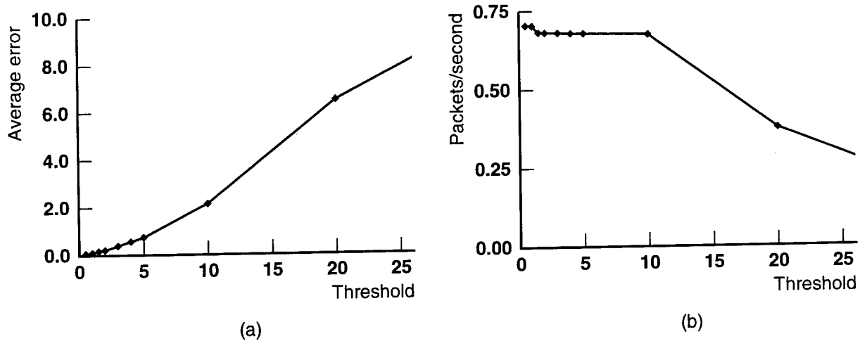
Figure 10: Average History-Based Protocol (a) Error and (b) Packet Rate for Bounce Motion
