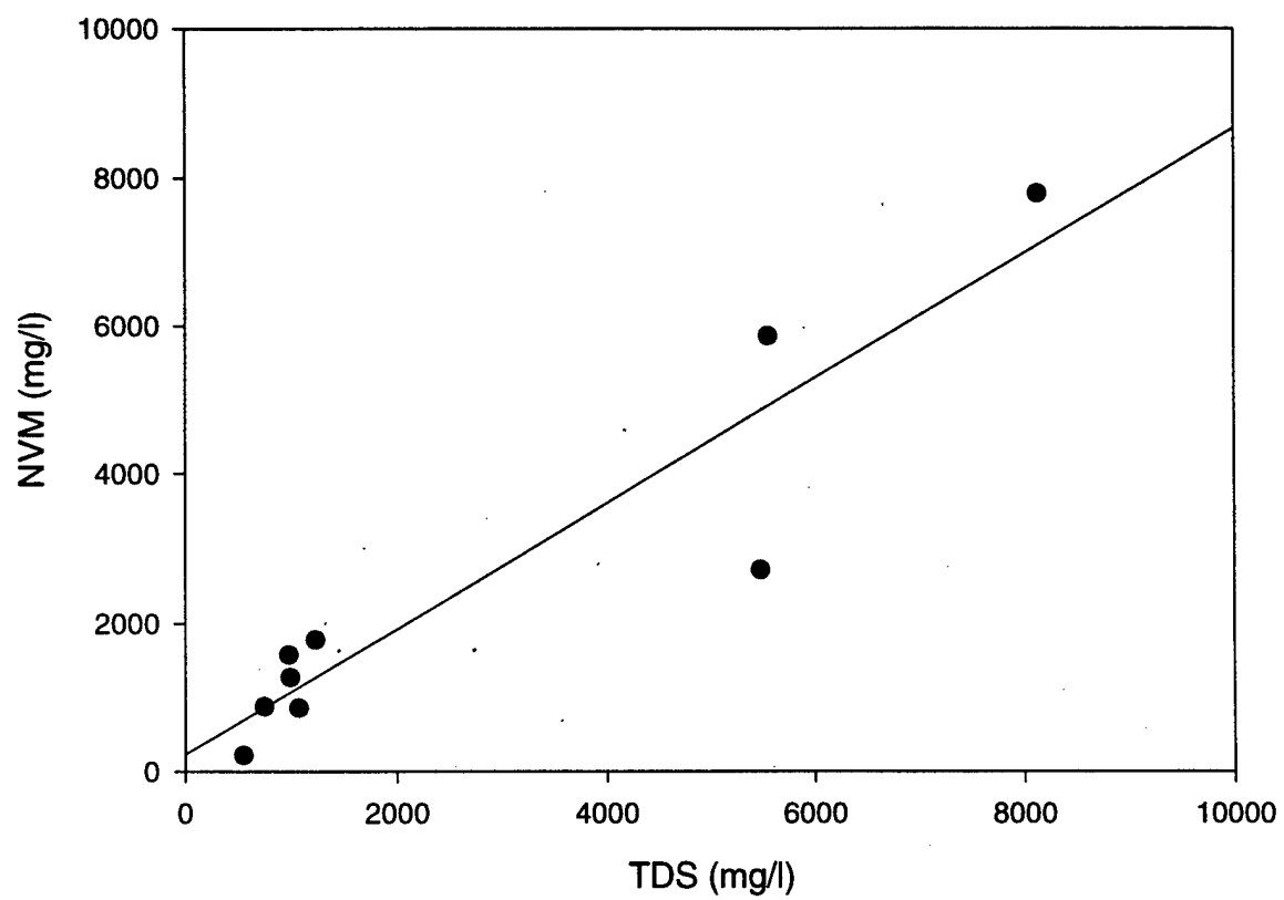
Figure 2. Sample components do not correlate. For each sample, Total Dissolved Solids was plotted against Non-Volatile Material(A). NVM(○) and TDS(●) were plotted against Chemical Oxygen Demand(B). TDS(●) and COD(○) were plotted against protein concentration(C).
