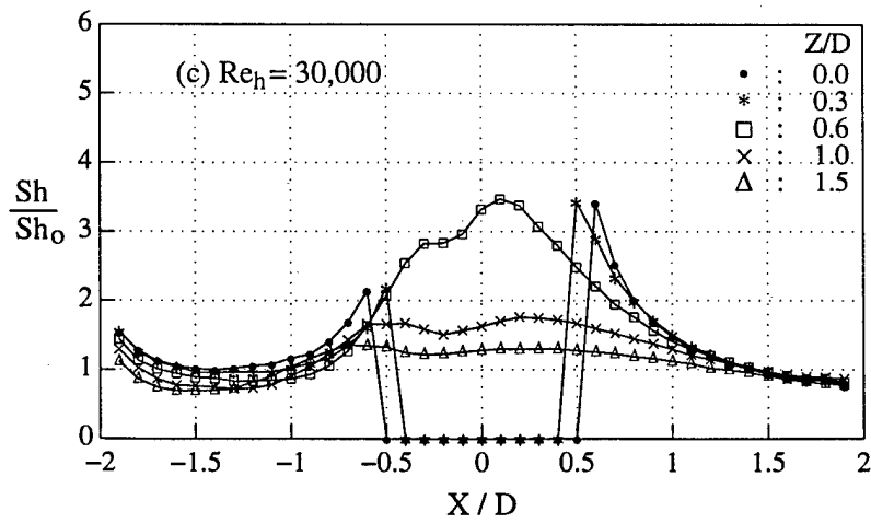
Fig. 25 Normalized Sh on plenum wall with one open hole.
