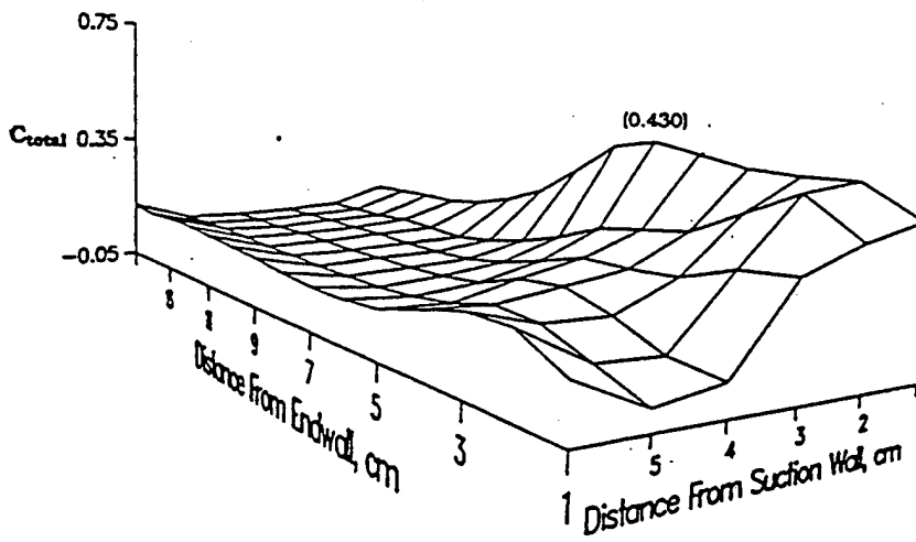
Fig. 14 b Distribution of the Total Loss at the Plane (with fence).
