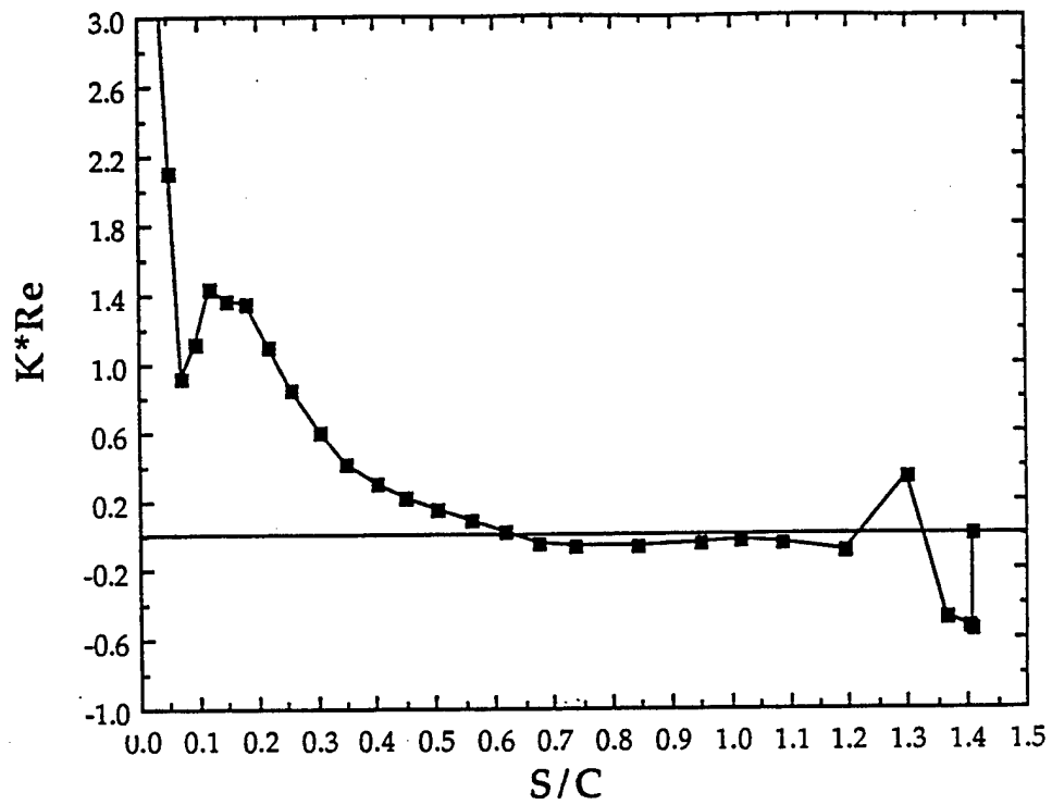
Fig.11 K*Re product distribution along suction wall side ( Re=634244 and 186045 )
