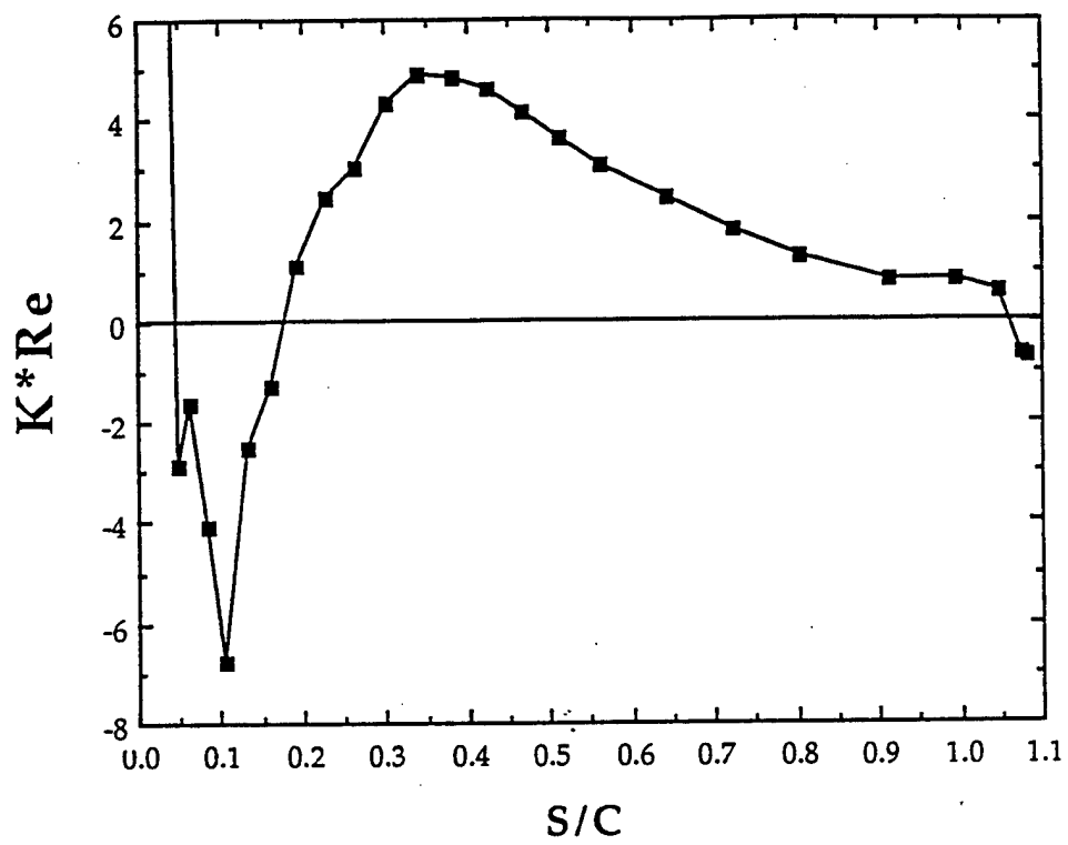
Fig. 10 K*Re_{\epsilon} product distribution along pressure wall side ( Re_{\epsilon}=634244 and 186045 )
