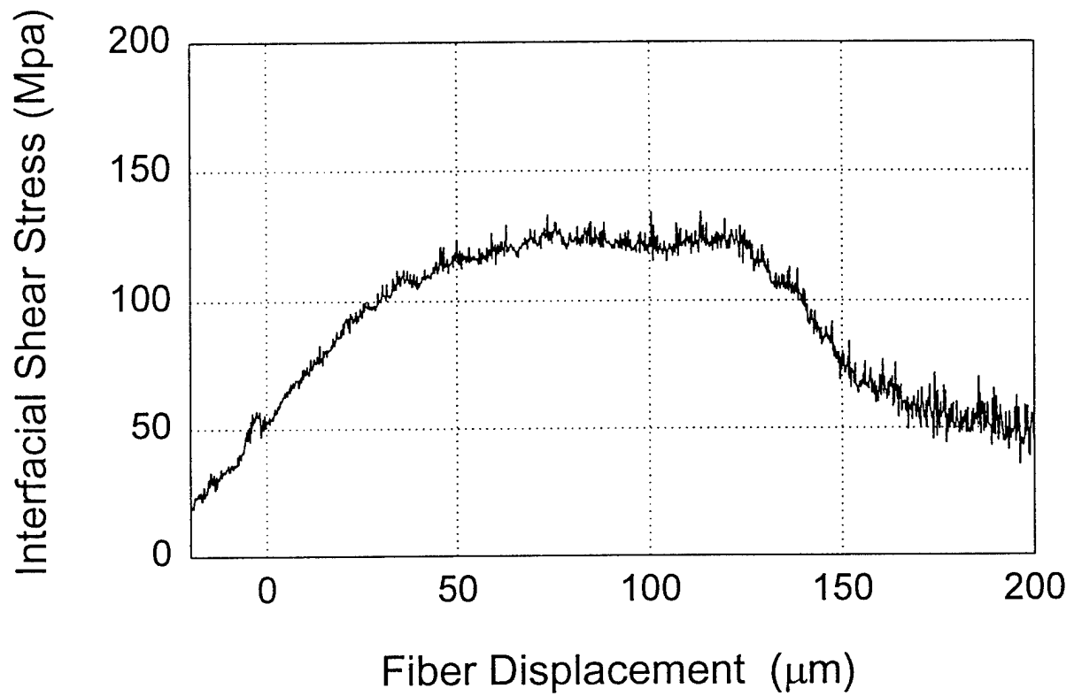
Fig. 2-12(a) Typical room temperature fiber pushout curve for Scs-6/Timetal-21S at 500°C / 5 hour aging condition. Thickness, H = 0.28 mm
