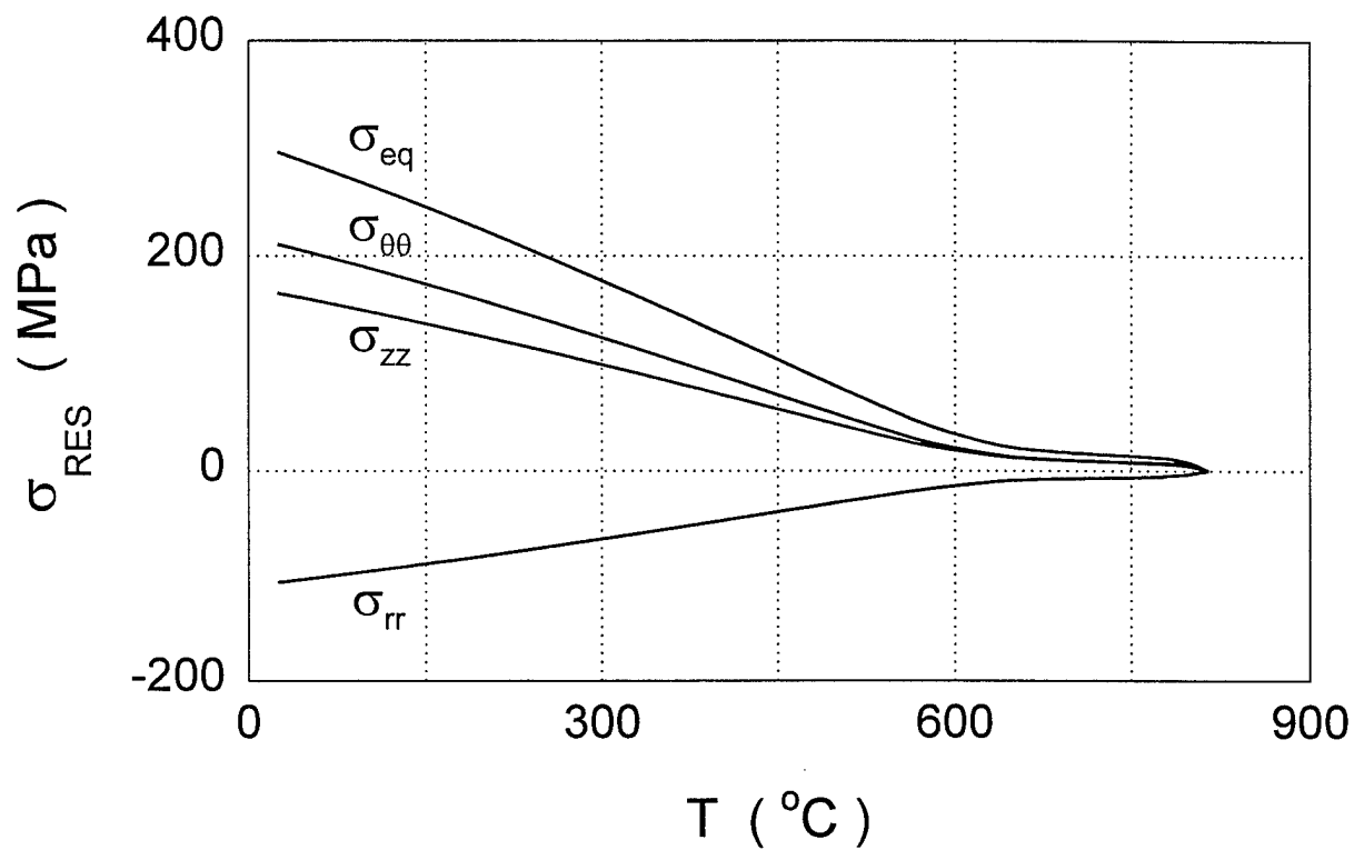
Fig. 3-3 Evolution of residual radial, axial, and hoop stress upon cooldown from 815 ^{\circ}\text{C} to room temperature in SCS-6/Timetal-21S
