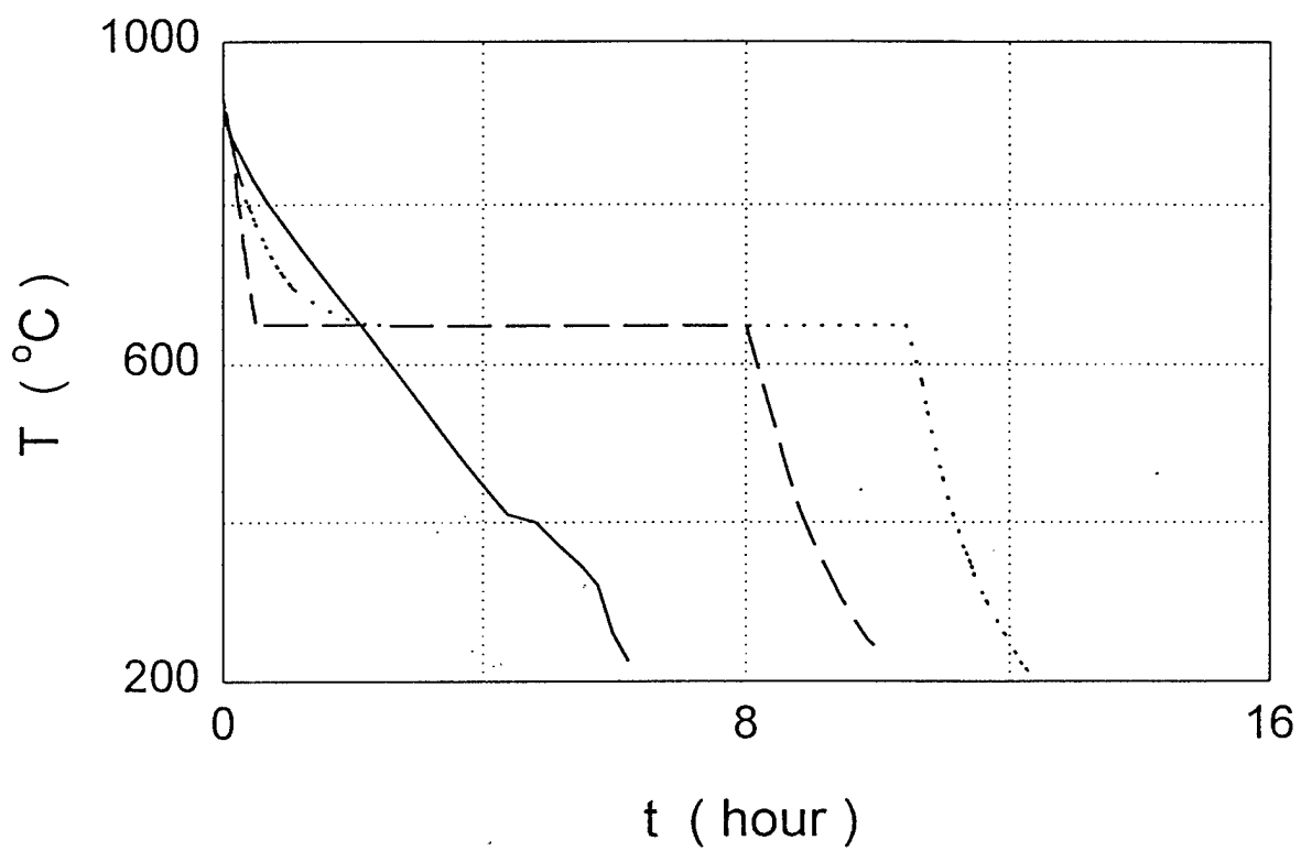
Fig. 4-1(a) Processing control variables employed during post-fabrication cool down of the composites - temperature profile
