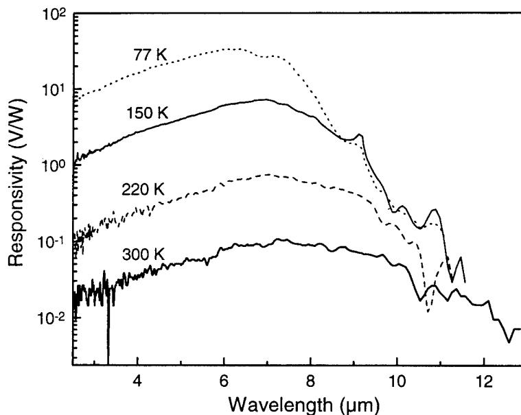
Figure 15: Photoresponse of p-π-n InSb/InAs 0.15 Sb 0.85 /InSb double heterojunction photodiode.
