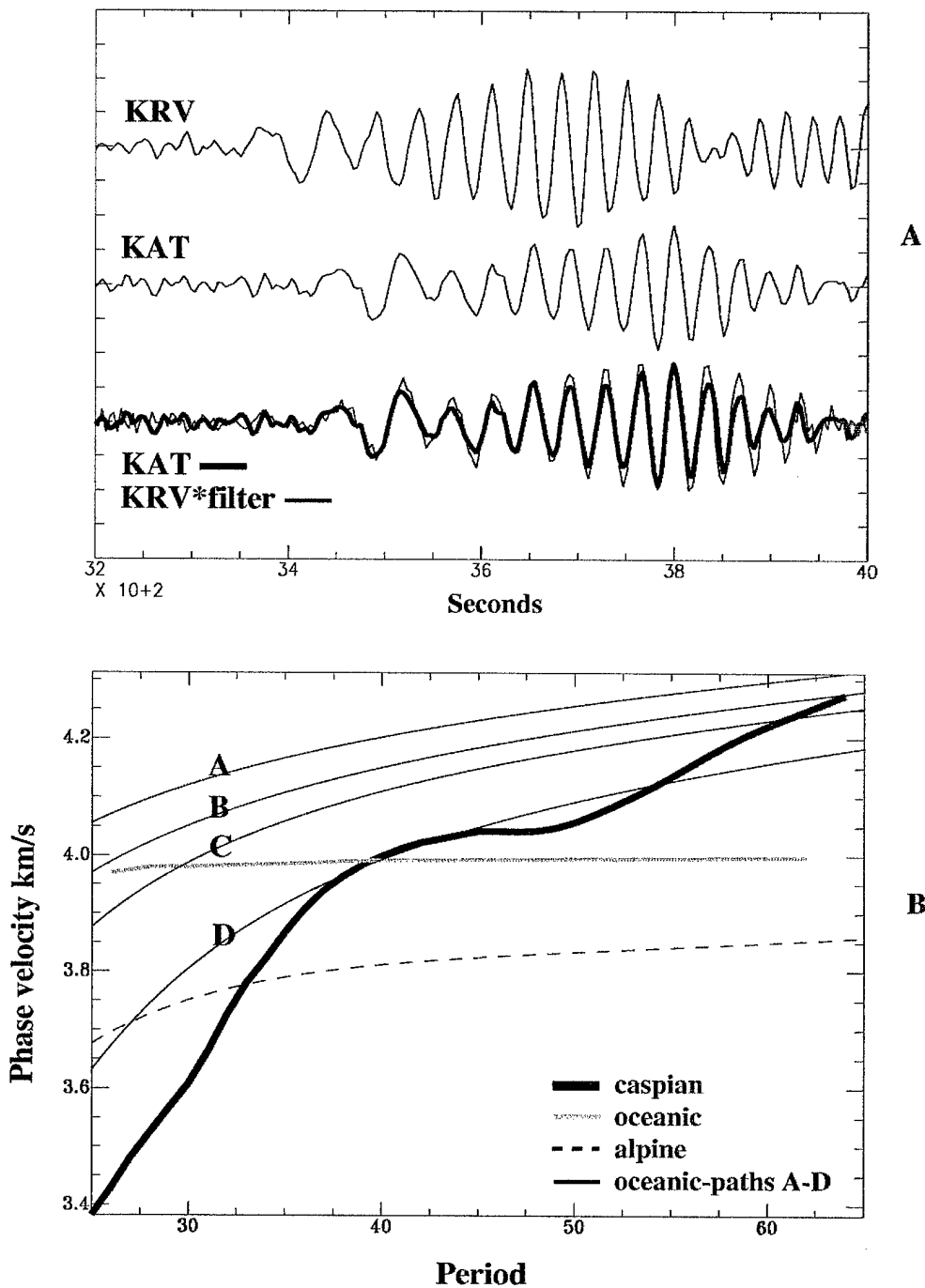
Figure 14. Fundamental mode Rayleigh wave phase velocity dispersion curve for the KRV-KAT path. This curve was computed from four seismogram pairs using a constrained least-squares algorithm (Gomberg et al. 1988). The KRV-KAT phase velocity curve is compared with observed dispersion curves for an ocean basin (Kuo et al. 1962), a continental tectonic region (Knopoff et al. 1966), and the Bay of Bengal (Brune and Singh 1988) region. The primary differences in paths "A" to "D" is an increase in thickness of the near surface sedimentary layer and an increase in Moho depth from "A" to "D".
