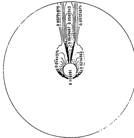
b) Contours of Molecular Nitrogen
