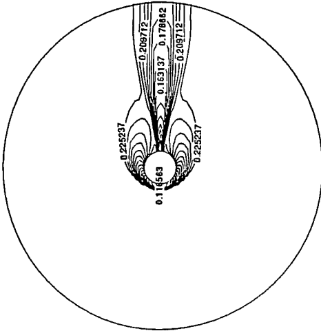
c) Contours of Molecular Oxygen
