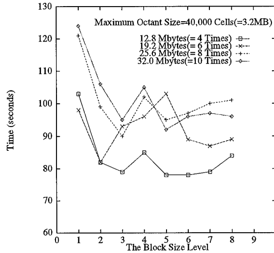
Figure 20: Timing of Constructing Streamlines by Using Non-Local Disk
