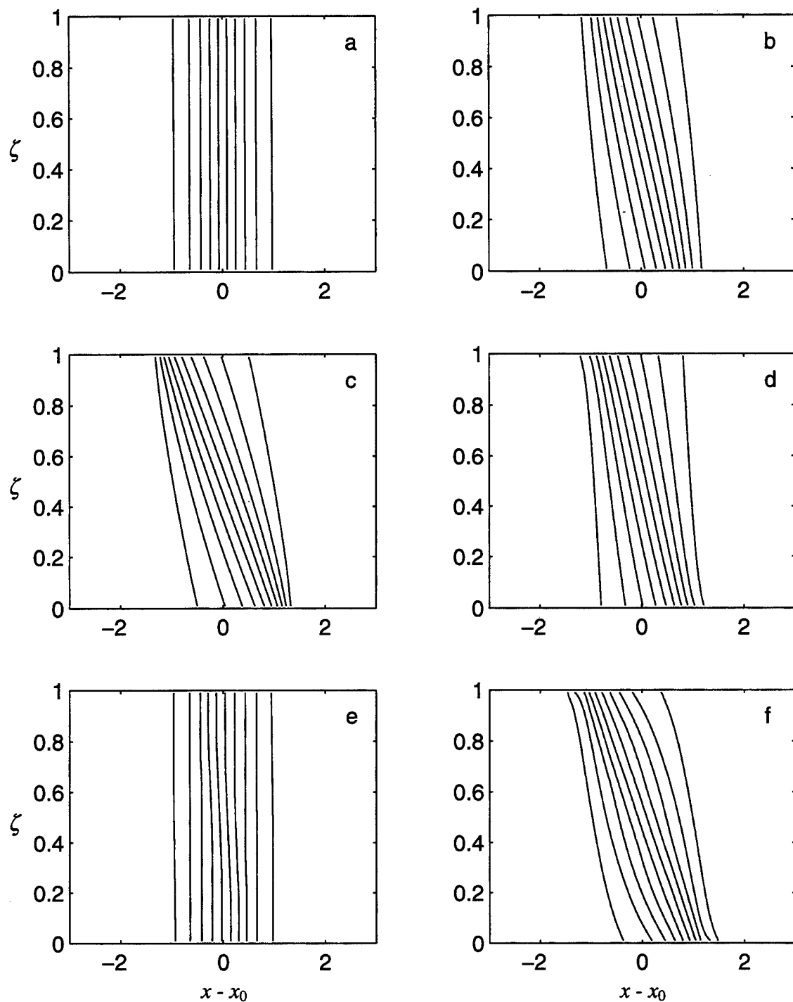
Figure 12. Time evolution of the total temperature cross-section for point 48 in Figure 7, for (a) t = 0 , (b) t = 1.8 f^{-1} , (c) t = \pi f^{-1} , (d) t = 4.7 f^{-1} , (e) t = 2\pi f^{-1} , and (f) t = 9.8 f^{-1} .
