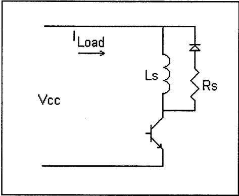
Figure 1-5 - Turn-On Snubber
