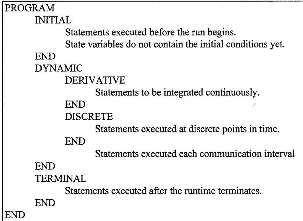
Figure 3-1 - ACSL Program Outline (from [Ref. 7])
