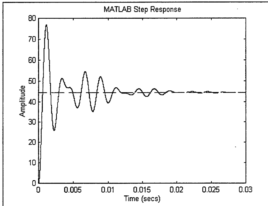
Figure 4-5 - Voltage Controller Transient Response from MATLAB
