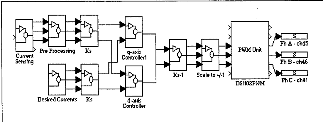
Figure F-1 - Stationary Controller
