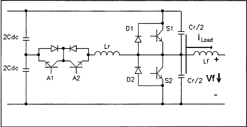
Figure 2-18 - Commutation, S1 Gated Off
