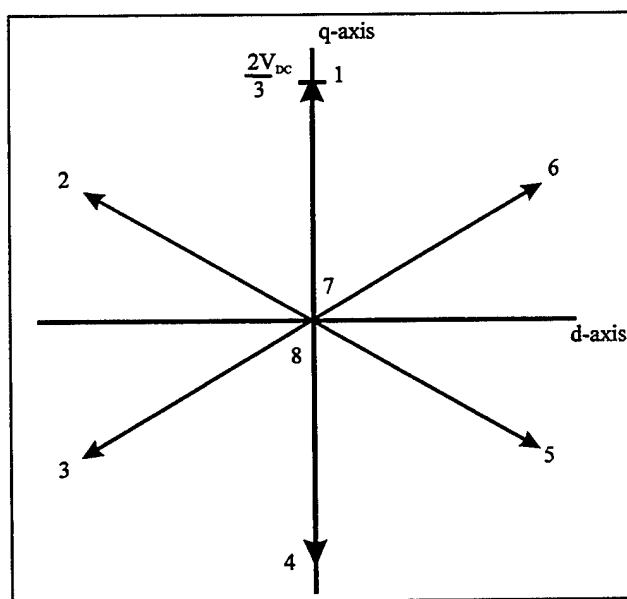
Figure 5-4 - Inverter Voltages in q-d Frame
