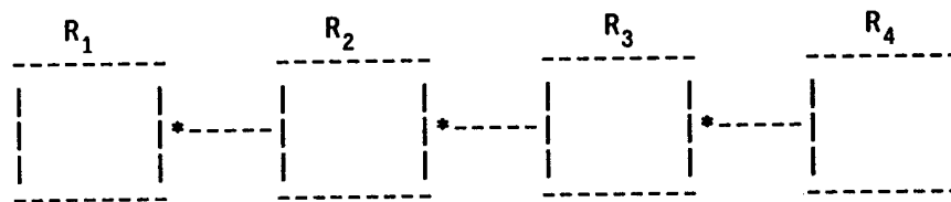
Figure 9-1: Four Relations. The symbol *— stands for an N-to-1 relationship.
