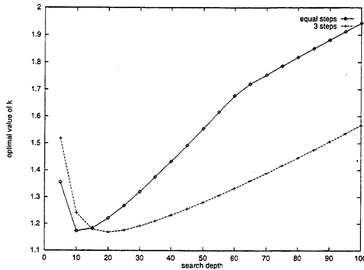
Figure 5.2: The optimal value of k increases with search depth.
