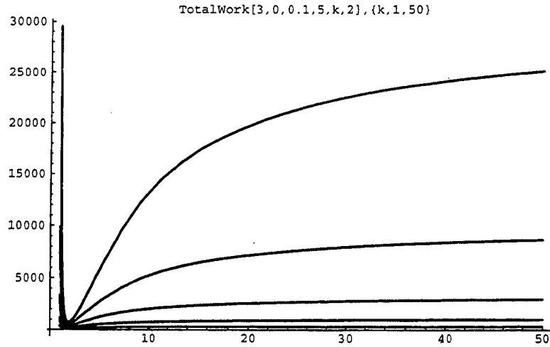
Figure 5.1: The amount of total work as a function of k , the ratio between levels of abstraction. The different curves result from different search depths.
