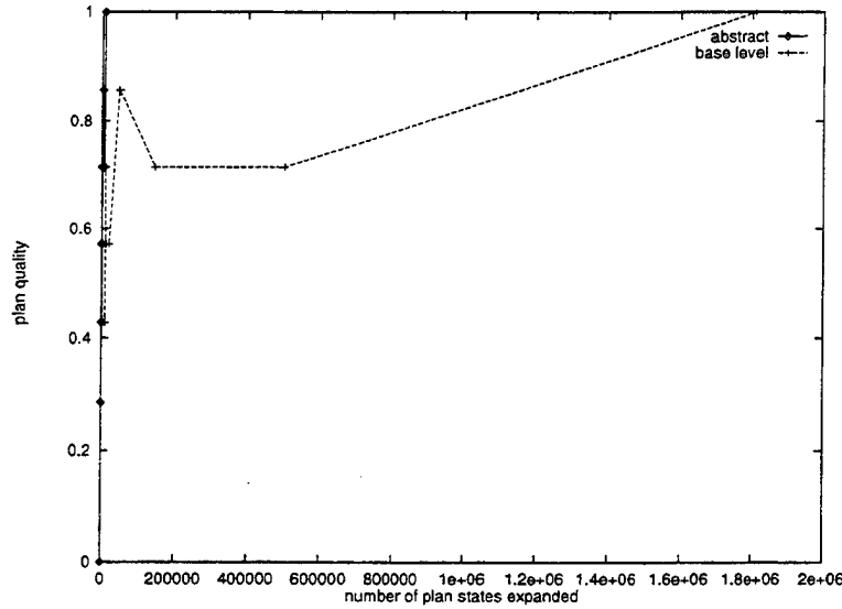
Figure 6.5: The quality of the plan in relation to the search effort expended, with abstraction and without. The abstract plan reaches the optimum near the left edge of the graph.
