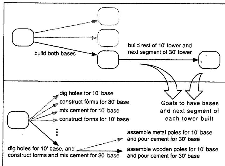
Figure 2.5: Further abstract search may constrain the lower-level search and may change the best plan at the lower level.
