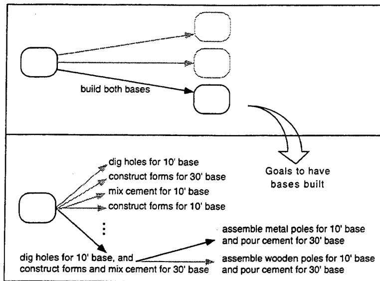
Figure 2.4: Abstract state information propagates to produce goals at the next lower level.
