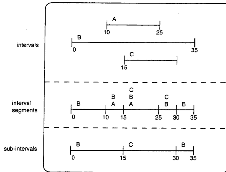
Figure 4.3: The representation of intervals in the implementation. Intervals are subdivided into interval segments and sub-intervals. In this example, interval C overrides B, which overrides A.
