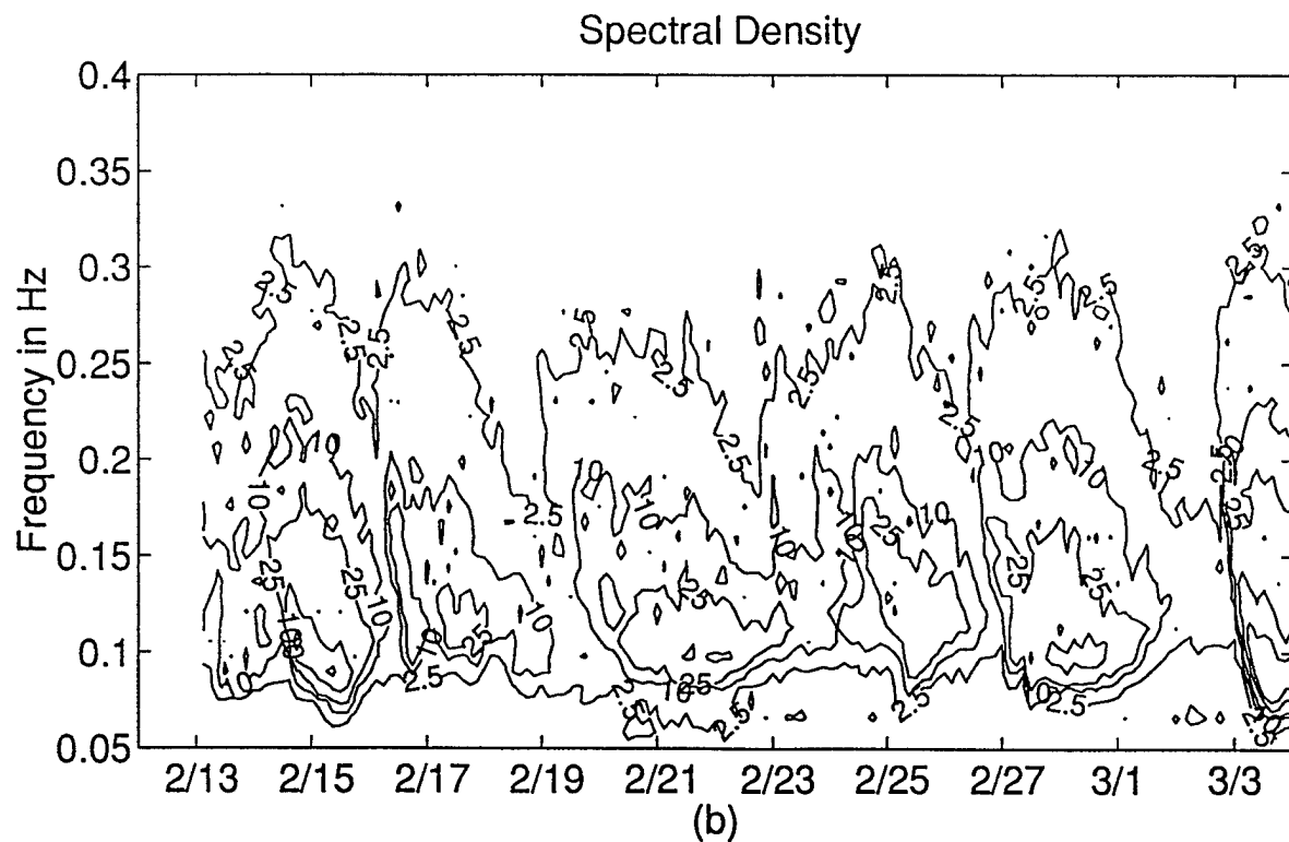
Figure 3.4.5: Spectral evolution of the surface waves. Contours of spectral density as a function of frequency over time. Contours at 2.5, 10, 25, 100, 250.
