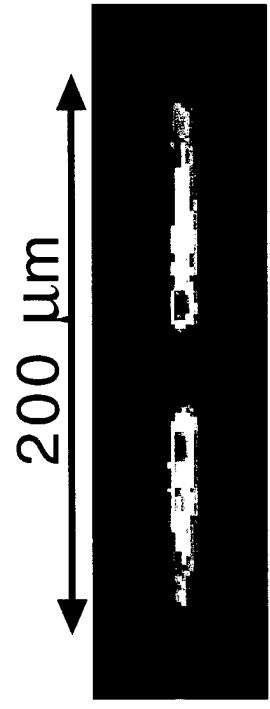
Two trapped condensates
