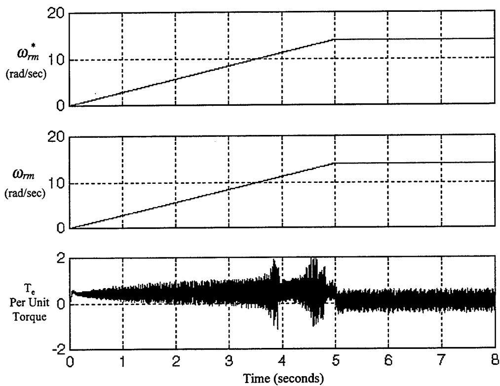
Figure 7-6. Transient Behavior of Cycloconverter Propulsion Motor Drive.
