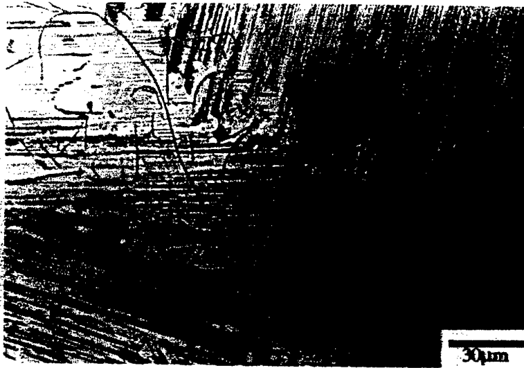
Boride morphology in Ti-47Al-2Cr-2Nb-1B
