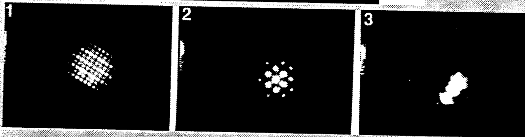
Dark field with reflection from \gamma_i showing relation between \gamma_i (area 1) and massive \gamma_m (area 2) and absence of relation between \alpha (area 3) and \gamma_m
