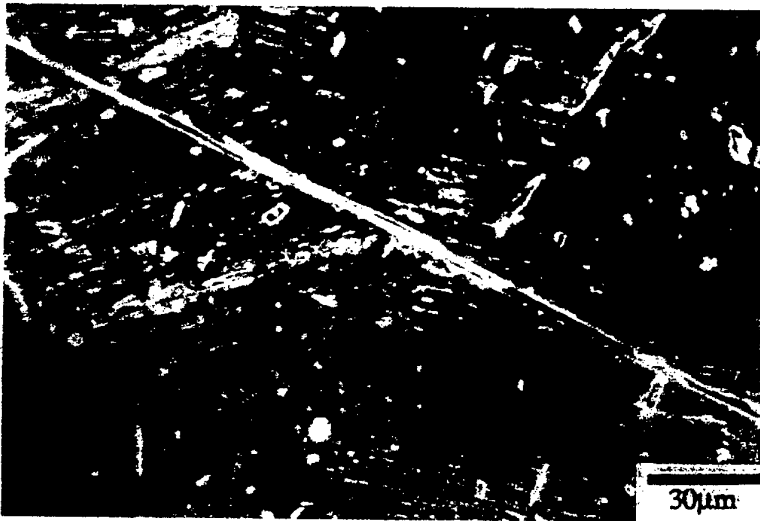
Boride morphology in Ti-47Al-2Ta-1Mn-1Cr-1B-0.2Si.
