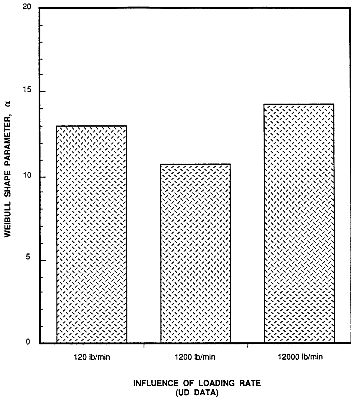
Figure A.8. Influence of Loading Rate on Static Strength Scatter (UD Data Ref. A.2).
