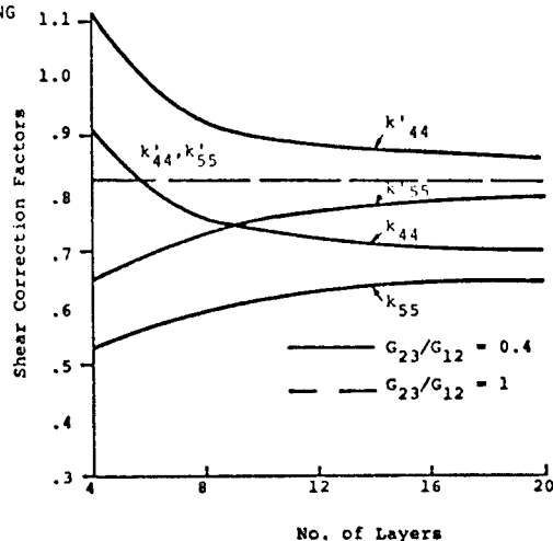
SHEAR CORRECTION FACTORS FOR A SYMMETRIC CROSS PLY LAMINATE WITH EQUAL PERCENTAGE OF 0° AND 90° LAYERS
