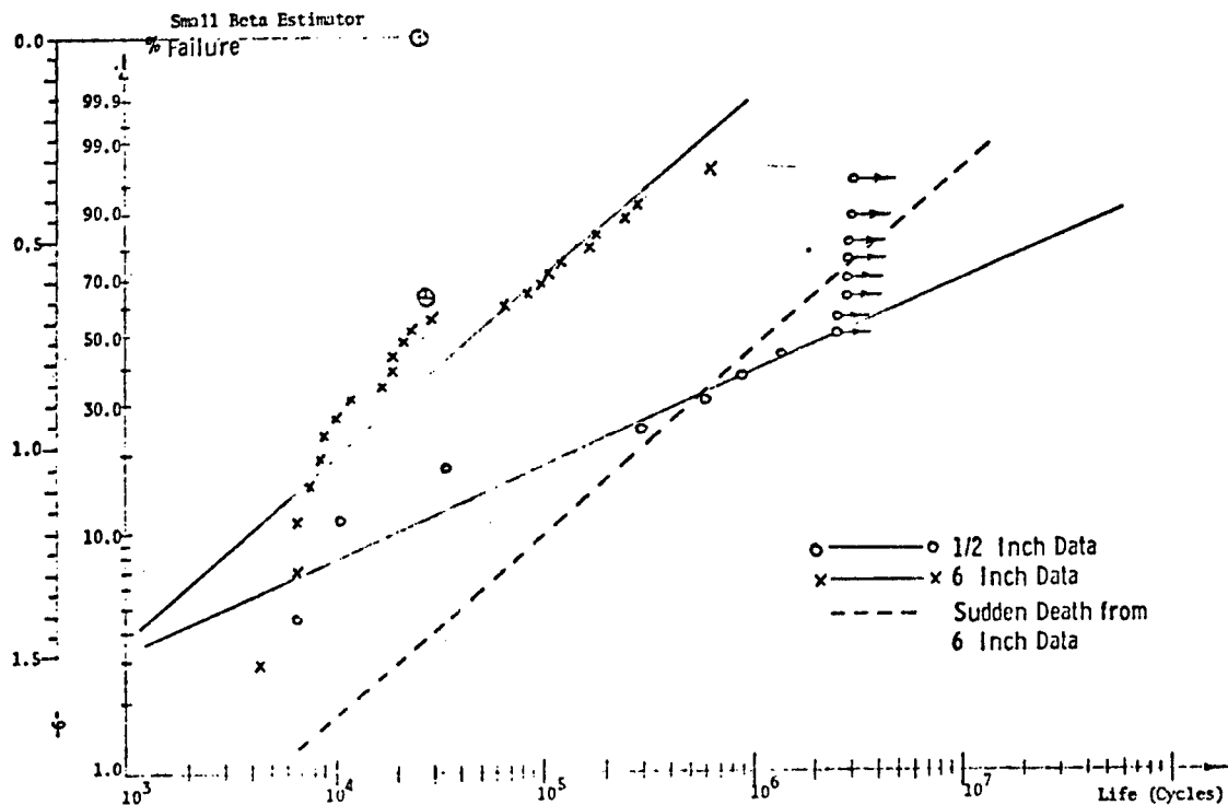
Applicability of In-Series Model to 6 Inch and 1/2 Inch Specimens Under Dynamic Loading (Weibull Coordinates)
