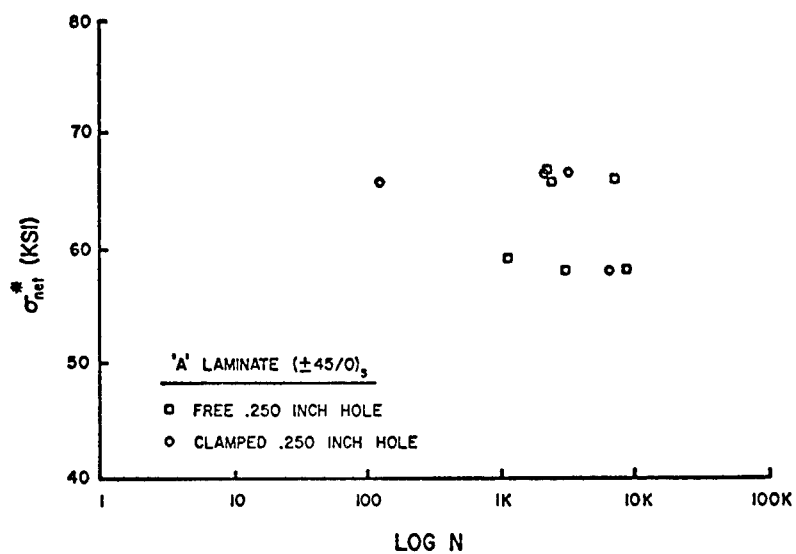
FIGURE 14 'A' laminate: Free hole vs. Clamped hole
