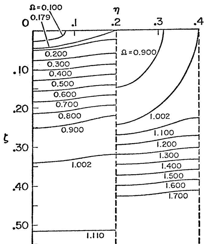
FIG. 4 CURVES OF CONSTANT \Omega ON THE ANTI-PLANE STRAIN DISPERSION SURFACE
