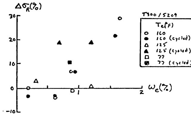
Figure 14 Altered Residual Stresses in Dry CY70/339 and T300/5209 (0 2 , 90 2 ) L Laminates After Hygrothermal Cycling. Specimens Previously Exposed to Equilibrium Moisture Content ω e at Three Temperatures (See Legend). Some Specimens Then Cycled 10 Times From 77 to 160°F. All Specimens Then Dried at 125°F.
