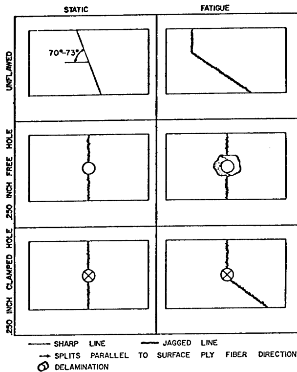
FIGURE 11 Schematic representation of failure modes - 'A' laminate.
