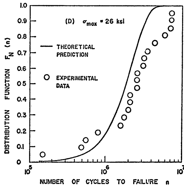
Fig. 9: Distribution Function of Fatigue Life, \sigma_{\min} = +16 \text{ ksi} , \sigma_{\max} = 26 \text{ ksi} .
