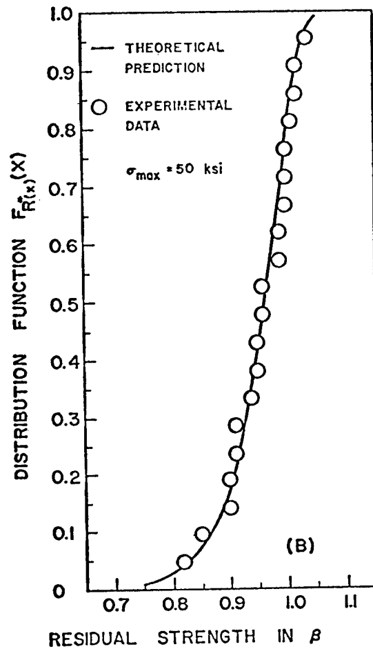
Fig. 5: Distribution Function of Residual Strength, \sigma_{\min} = -16 \text{ ksi} , \sigma_{\max} = 50 \text{ ksi} , n = 2,150 cycles.
