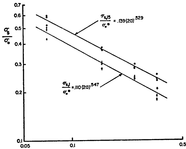
FIGURE 10 2a DISCONTINUITY LENGTH
