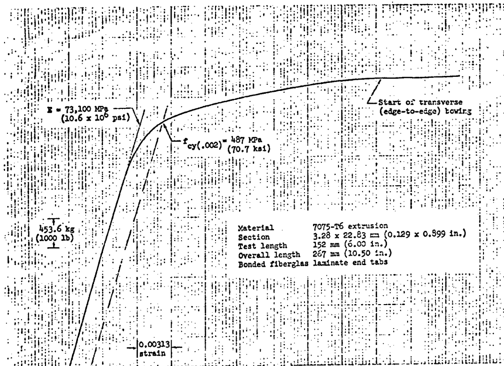
Automatically Recorded Extensometer Data Obtained During Compression Test of Al Alloy Coupon in Full Fixity Apparatus
