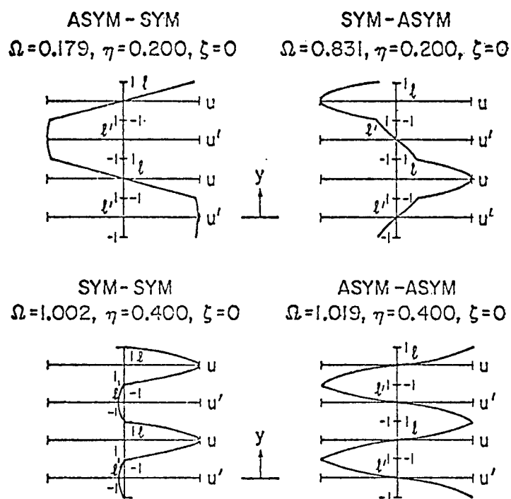
FIG. 9 NODE SHAPES AT POINTS ON THE ENDS OF BRILLOUIN ZONES ( \zeta = 0 ).
