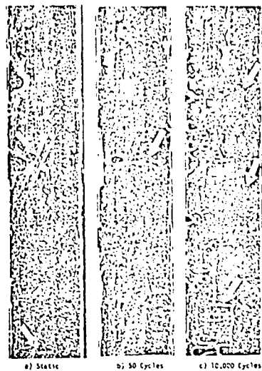
Replicas of 1600 lb. Type 1 Specimen
