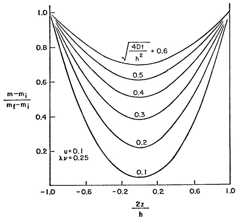
Distribution of mass of moisture per unit mass of solid for u = 0.10 and \lambda\nu = 0.25
