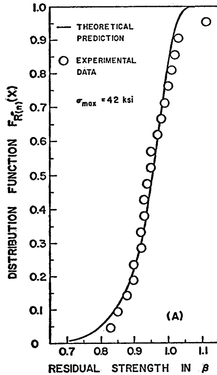
Fig. 4: Distribution Function of Residual Strength, \sigma_{\min} = -16 \text{ ksi} , \sigma_{\max} = 42 \text{ ksi} , n = 14,400 cycles.
