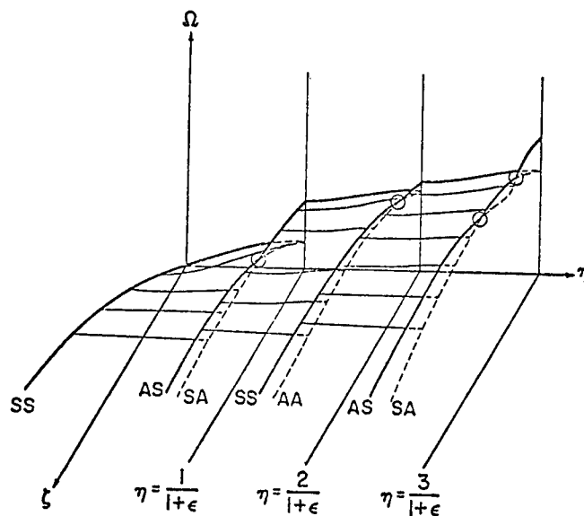
FIG. 2 ANTIPLANE STRAIN DISPERSION SURFACE ON THE EXTENDED ZONE SCHEME
