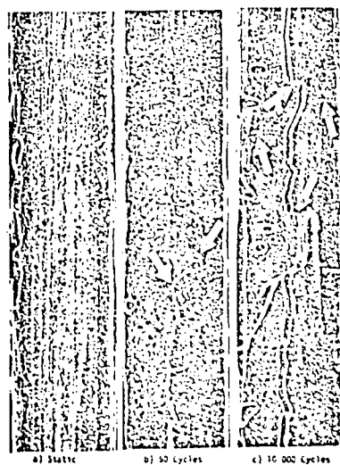
Replicas of 2000 lb. Type 1 Specimen
