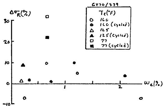
Figure 14 Altered Residual Stresses in Dry CY70/339 and T300/5209 (0 2 , 90 2 ) L Laminates After Hygrothermal Cycling. Specimens Previously Exposed to Equilibrium Moisture Content ω e at Three Temperatures (See Legend). Some Specimens Then Cycled 10 Times From 77 to 160°F. All Specimens Then Dried at 125°F.
