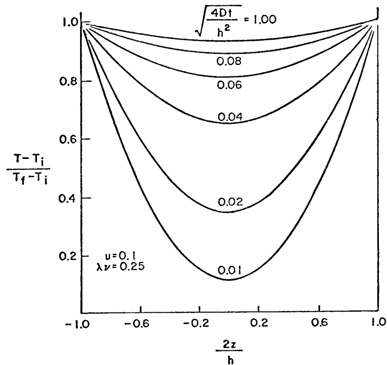
Variation of temperature through the slab for \lambda\nu = 0.25 and u = 0.1 when the moisture concentration at the surface is held constant
