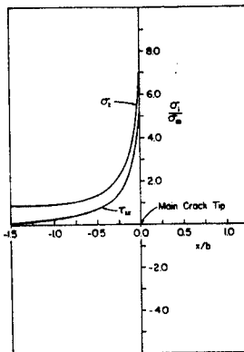
IN-PLANE STRESS
