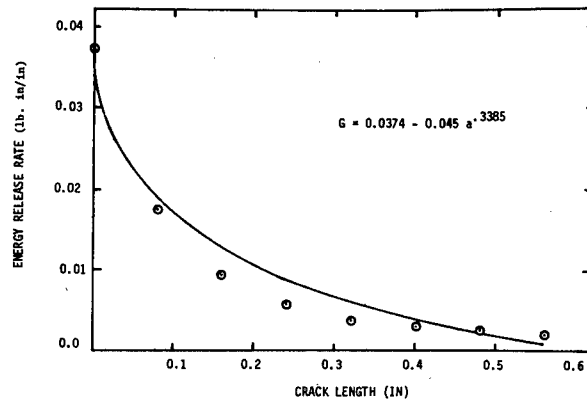
Energy Release Rate for Transverse Cracking in a [90]_S lamina.
