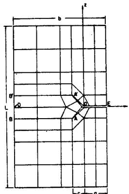
CRACK-BRANCH MODELING
