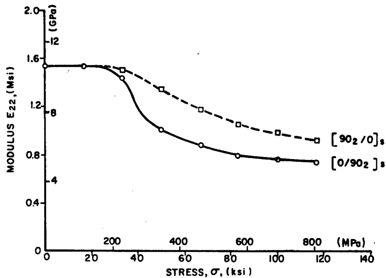
Fig. 12. Effective Transverse Modulus of 90-deg Layer in [0/90_2]_s and [90_2/0]_s Graphite/Epoxy Laminates under Uniaxial Tensile Loading.
