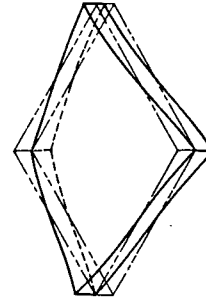
SPURIOUS ZERO ENERGY MODES (QHD28 ELEMENT)
