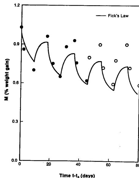
Figure 18. Moisture content (in % weight gain) during cyclic exposure to 0% and 95% relative humidity at 130°F, with cycle interval of 9 days.
