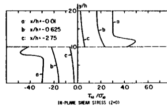
IN-PLANE SHEAR STRESS (2-D)
