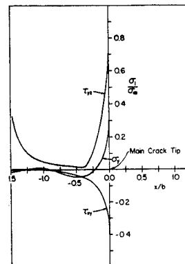
INTERLAMINAR STRESSES (45 PLY, 2-D)
