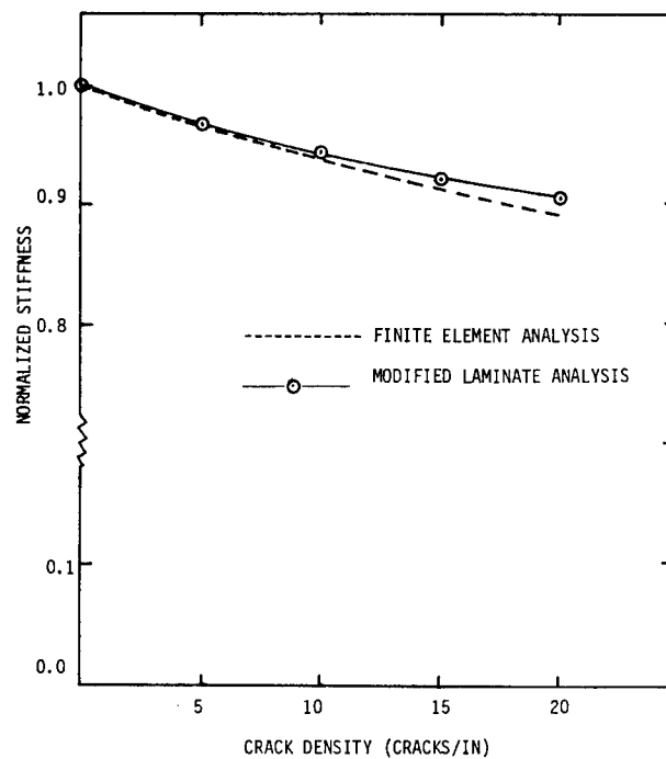
STIFFNESS REDUCTION FOR TRANSVERSE CRACKING IN A [0,90]_5 LAMINATE.
