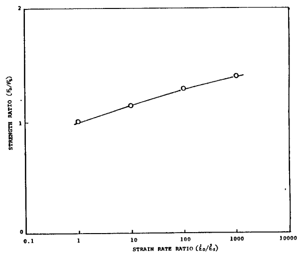
Tensile strength ratio of F-105/T300 90-deg unidirectional composite
