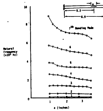
FREQUENCY (F.E. PREDICTION)
