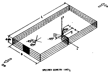
SPECIMEN GEOMETRY (1985)
