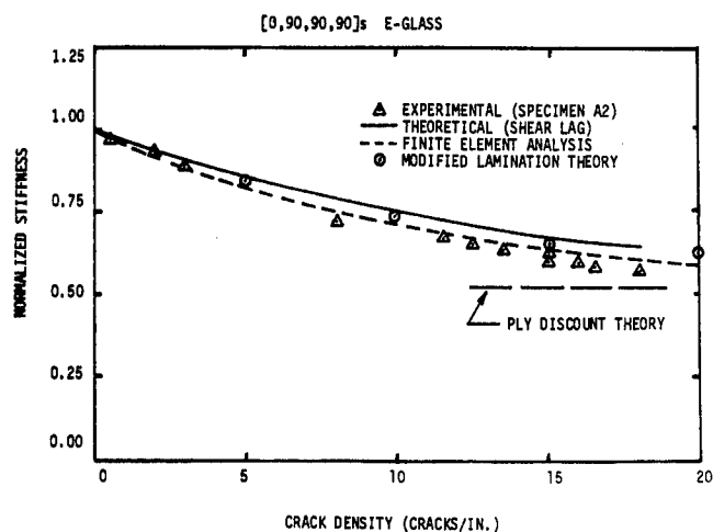
PREDICTIONS AND MEASUREMENTS OF STIFFNESS AS A FUNCTION OF CRACK DENSITY FOR A [0,90]_8 LAMINATE.
