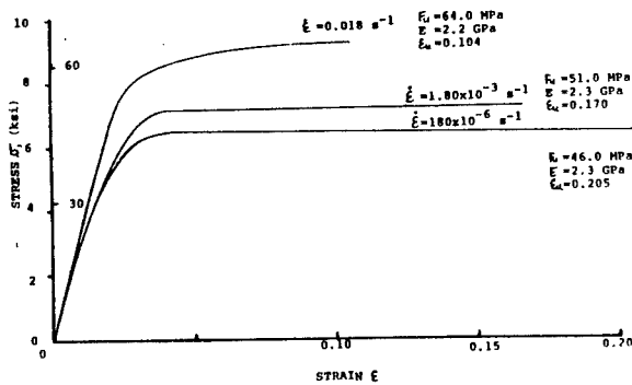
F-105 resin under tensile loading
