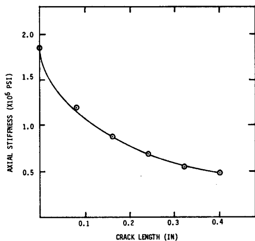
STIFFNESS REDUCTION IN [0,90]_5 LAMINATE FOR TRANSVERSE CRACKING
