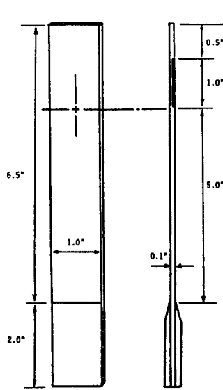
IMPACT SPECIMEN GEOMETRY
