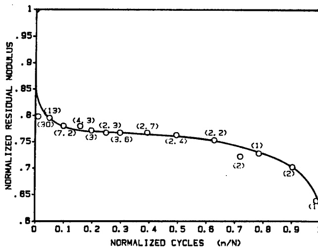
Normalized Residual Modulus for [0/90_4]_S Graphite/Epoxy Specimen under Fatigue Loading at R = 0.1 and \sigma_{\max} = 345 \text{ MPa} (50 ksi)
