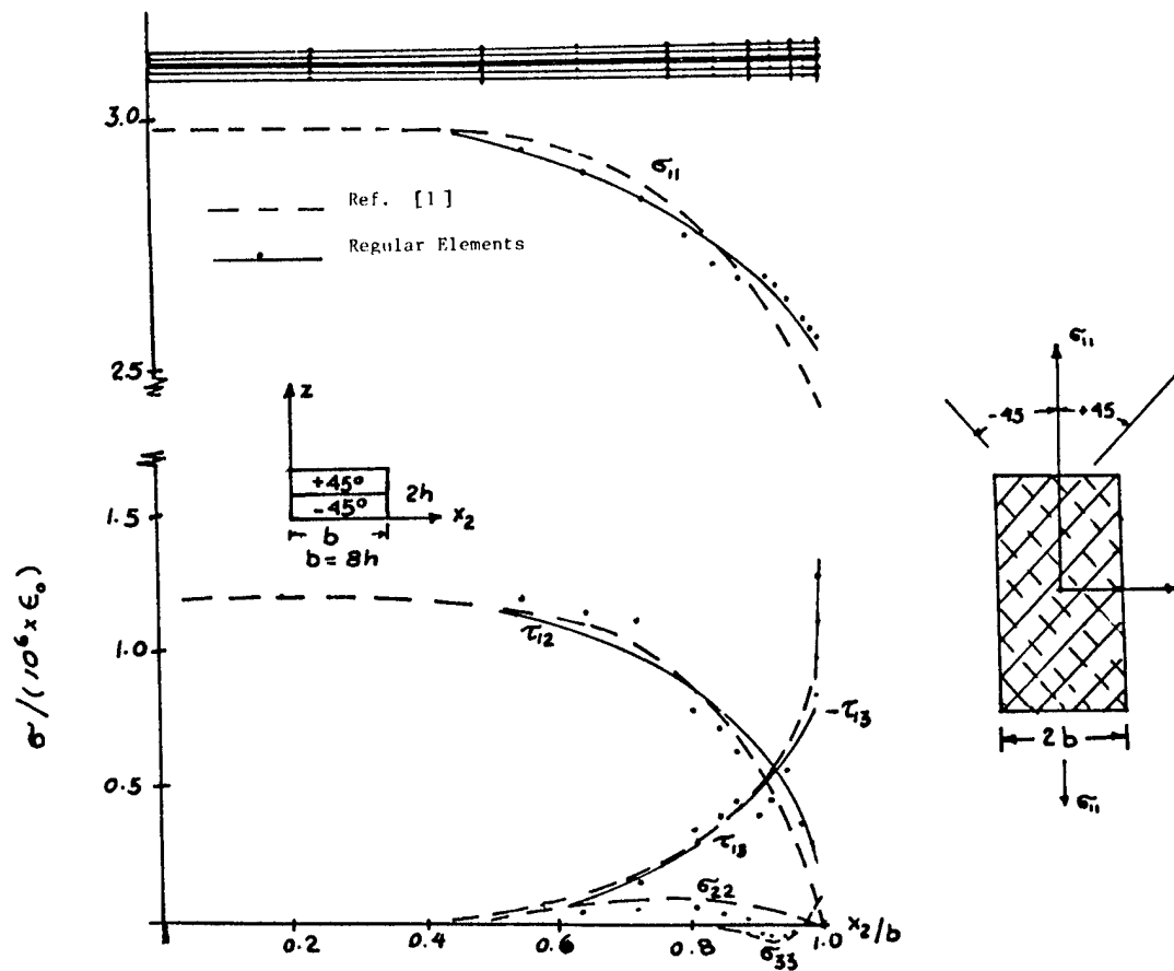
Figure 9. (+45/-45)_s Laminate
