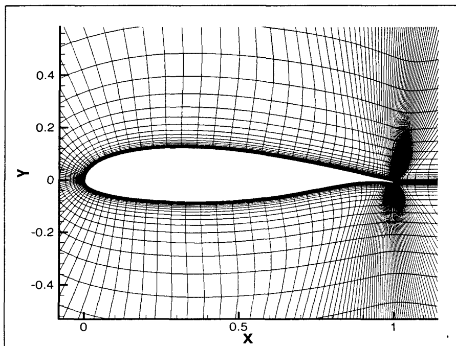
Fig. 3-3 MS-21 Airfoil
