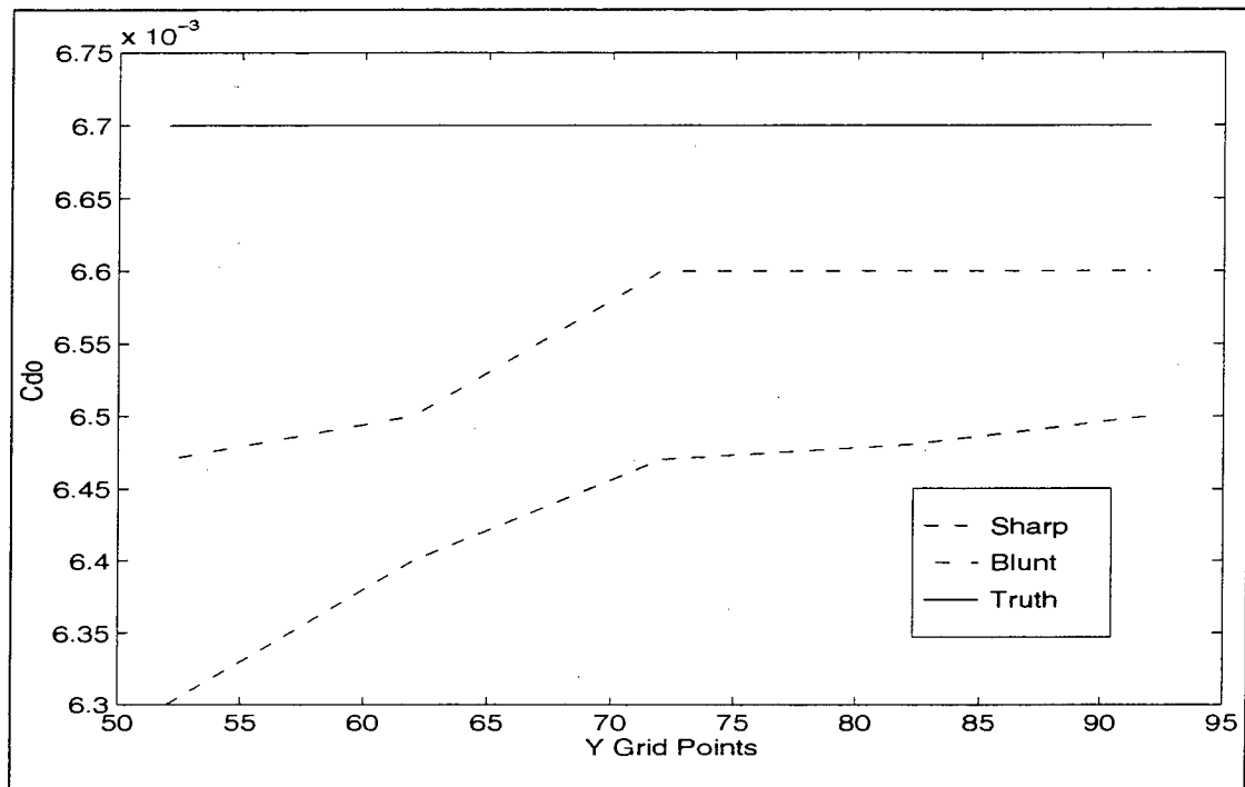
Fig. 3-9 Baldwin-Barth Model at y^+ \sim 1.0
