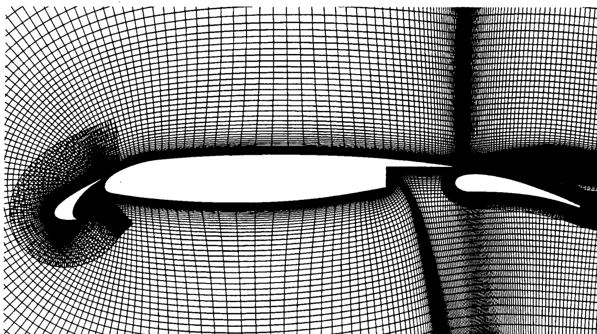
Fig. 6-1 High Lift Airfoil Section Using Chimera Gridding
