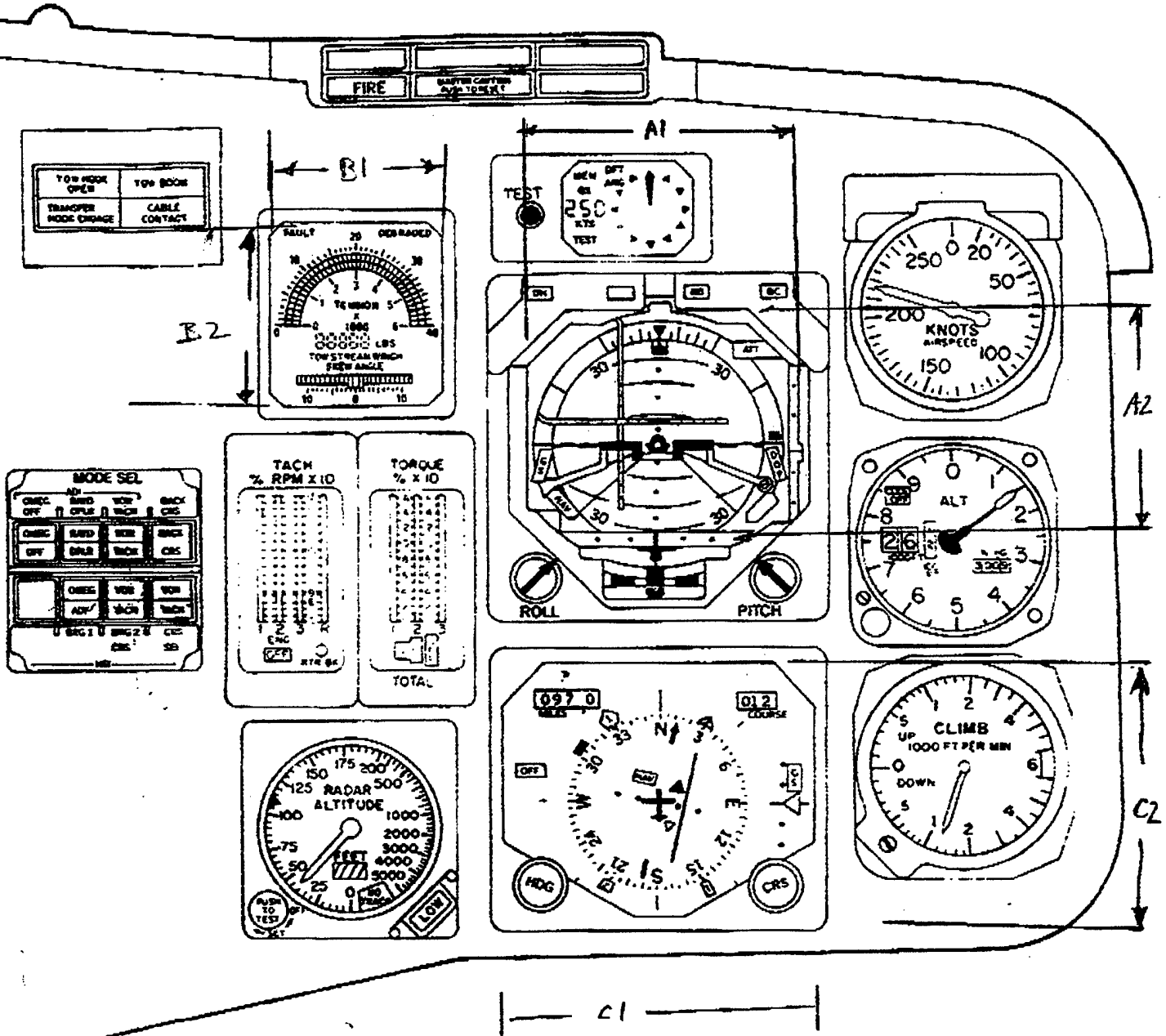
INSTRUMENT PANEL
