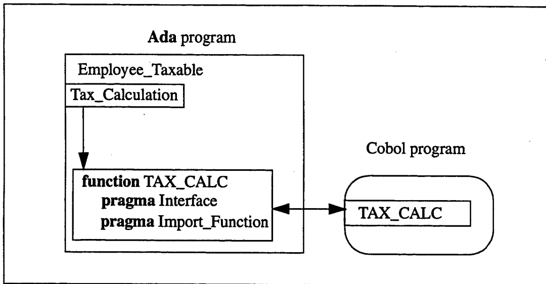
Figure 20. Function Wrapping Example in Ada.
