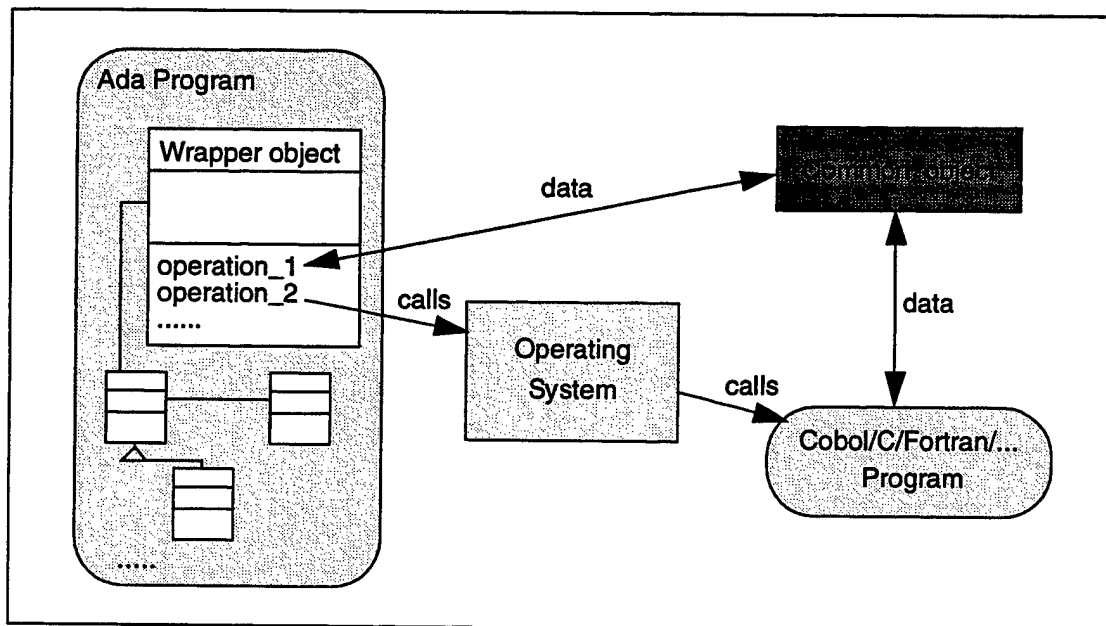
Figure 25. Interfacing Using a Common Area
