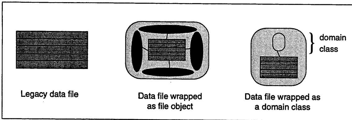
Figure 9. Wrapping Data Files
