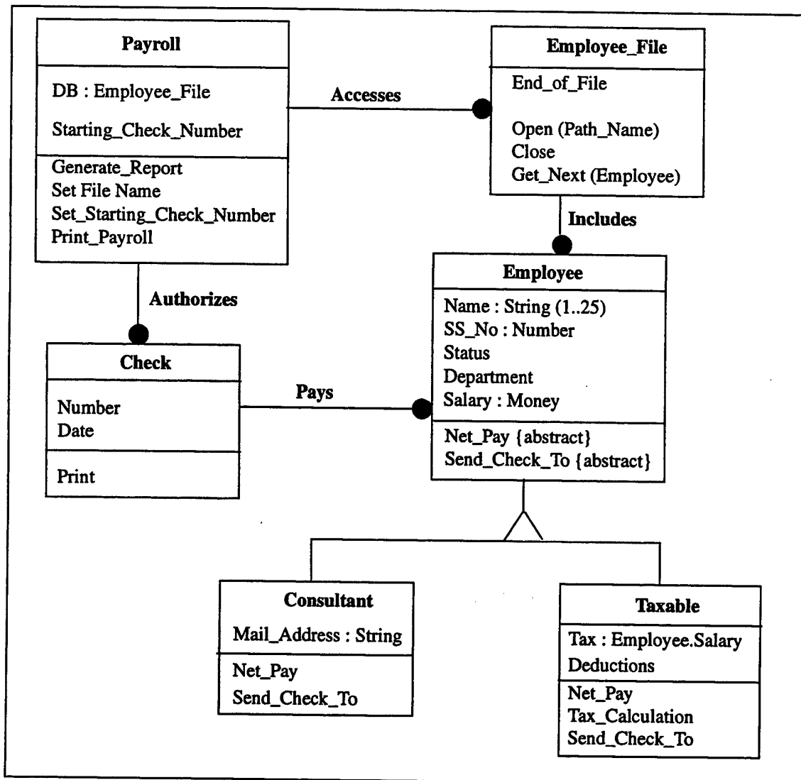
Figure 22. Object Model
