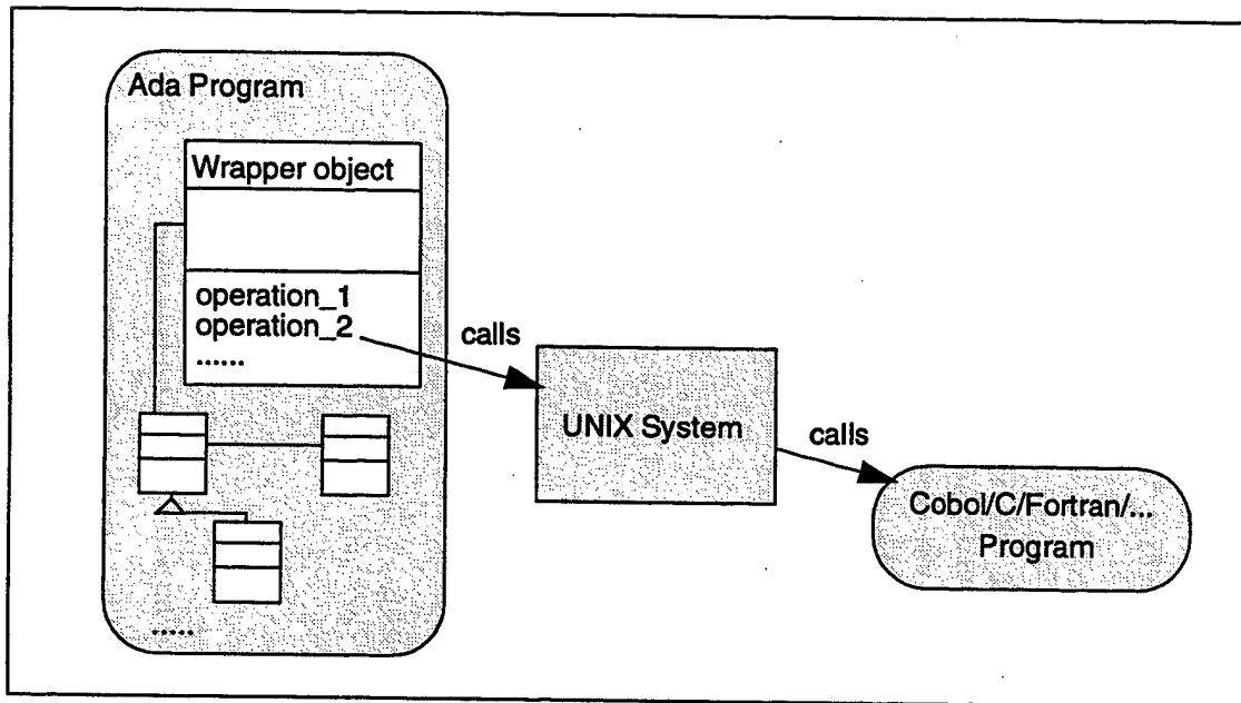
Figure 24. Linking via a Unix Shell
