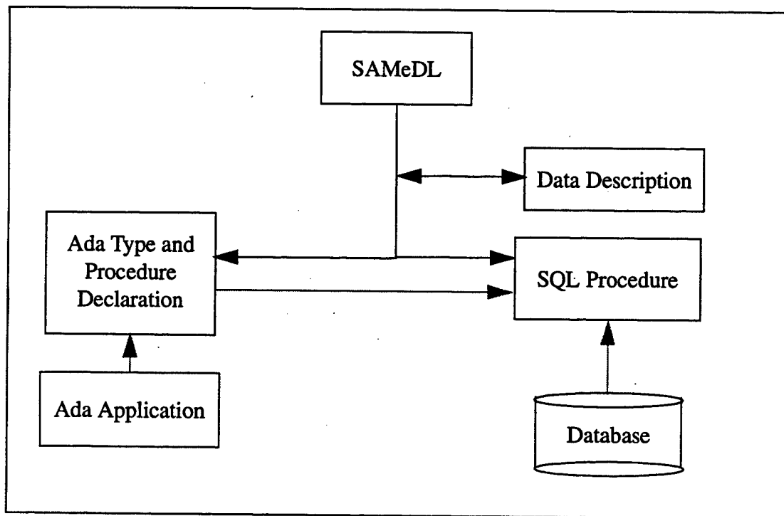
Figure 27. The Meaning of SAMeDL Text
