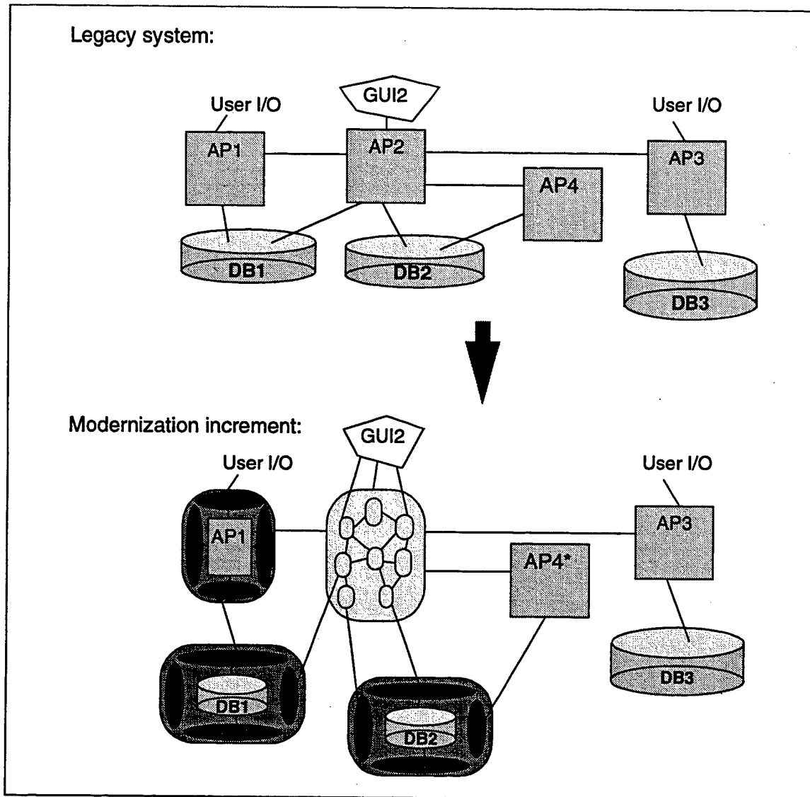
Figure 5. Divide-and-Conquer With Some Wrapping
