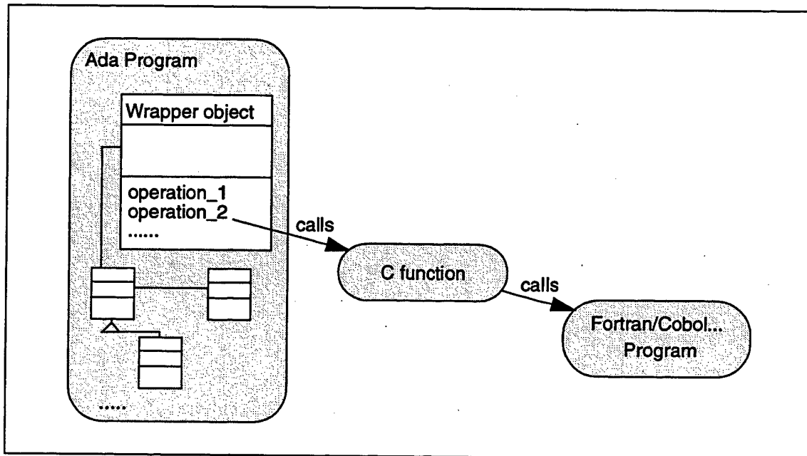
Figure 26. Interfacing via an Intermediate Language
