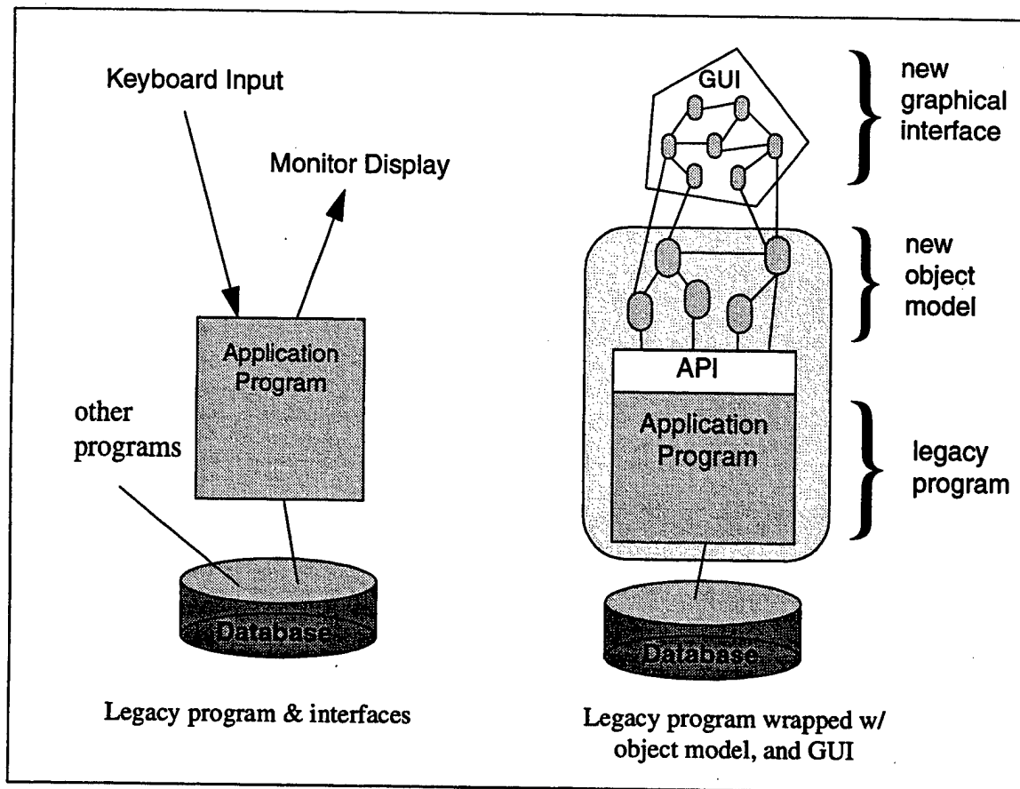
Figure 15. Wrapping Programs with Object Models
