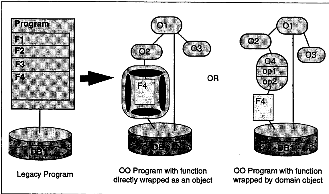
Figure 8. Wrapping Program Functions
