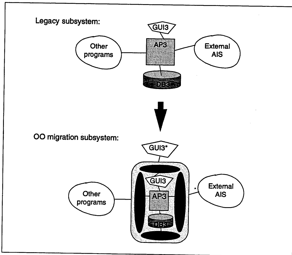
Figure 17. Wrapping Entire Subsystems
