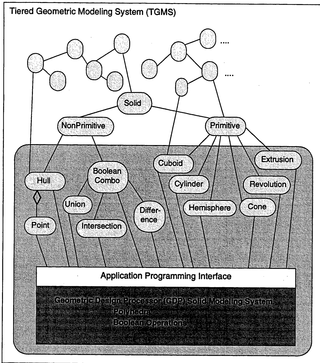
Figure 3. Example of System Wrapping for a Geometric Modeling System
