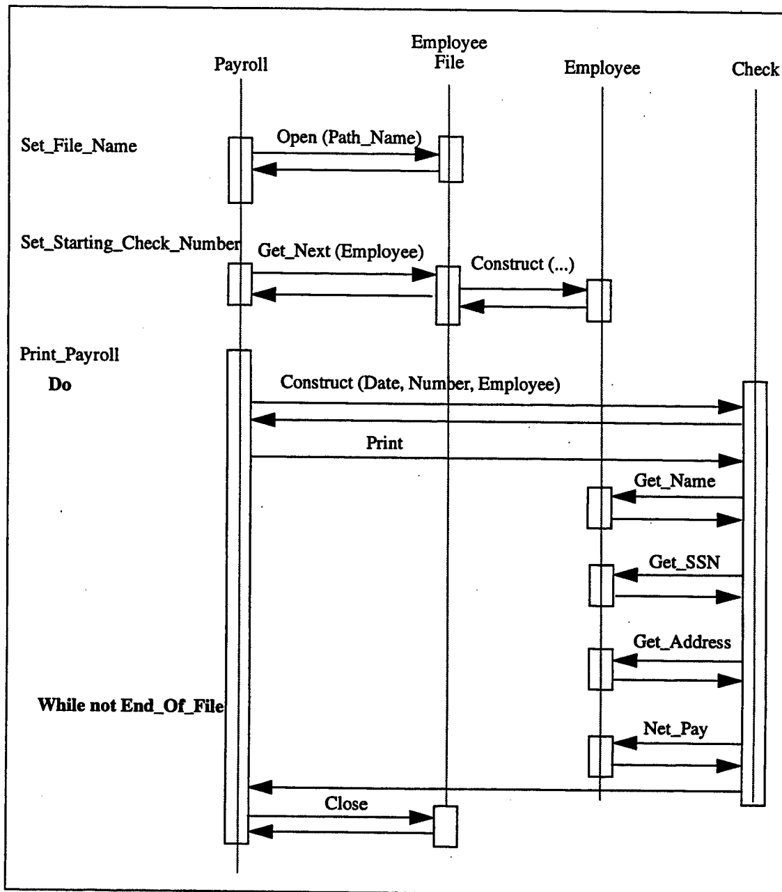
Figure 23. Interaction Diagram
