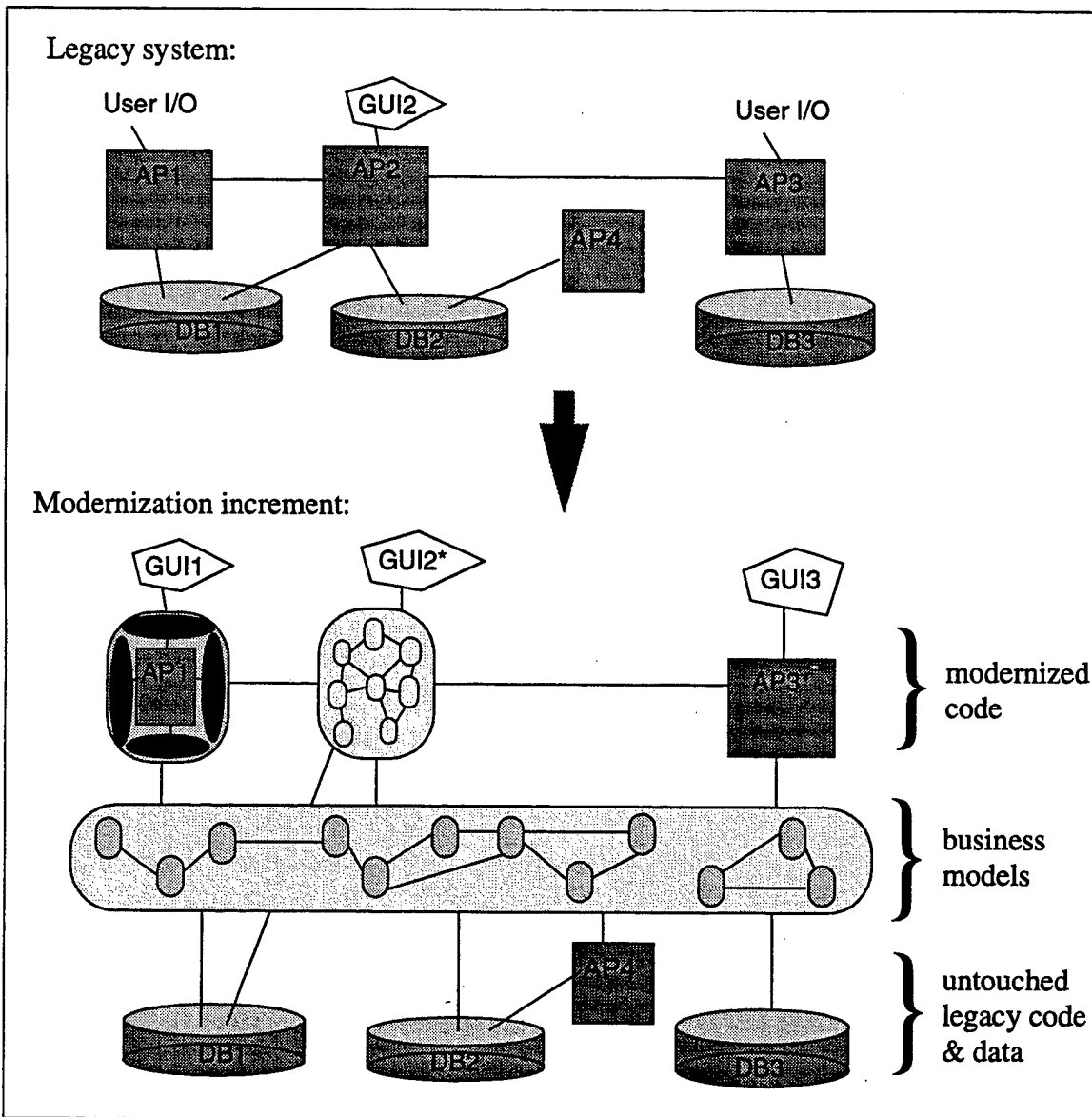
Figure 7. Unite-and-Conquer Strategy
