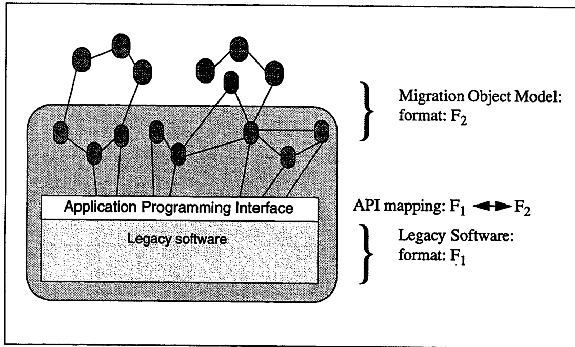
Figure 4. Wrapping Supports Translation to Standard Data Element Formats
