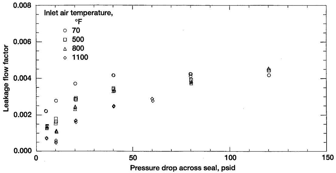
Figure 6.—Static test: leakage flow factor vs. pressure drop across seal as a function of inlet air temperature. Conventional low hysteresis brush seals, S/N 1 and 2.
