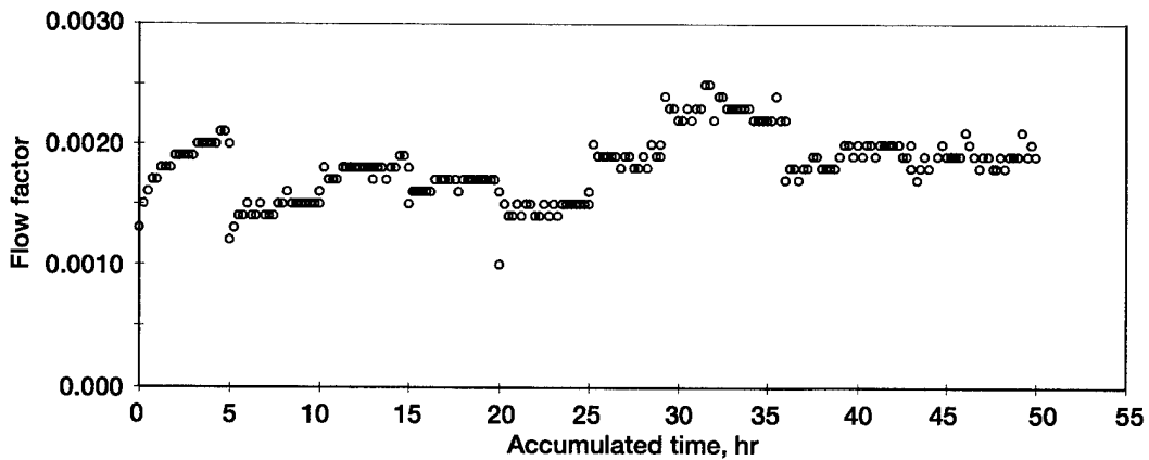
Figure 17.—Endurance test: flow factor vs. accumulated run time. Advanced low hysteresis brush seals, S/N 5 and 7.
