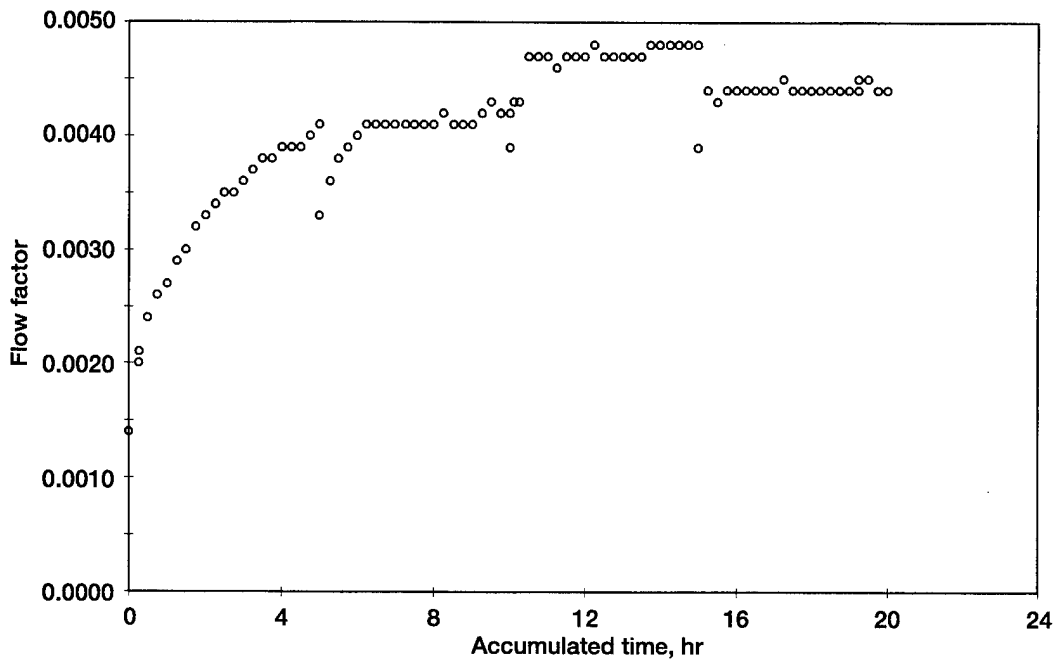
Figure 16.—Rotor runout test: flow factor vs. accumulated run time. Conventional low hysteresis brush seals, S/N 6 and 8.
