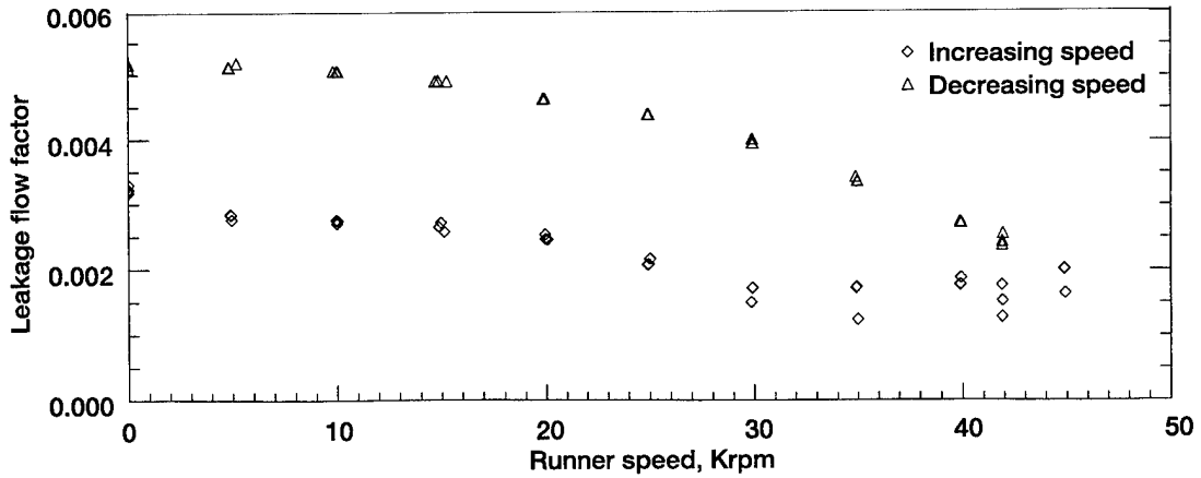
Figure 14.—Effect of speed ramp up and down on leakage flow factor for advanced low hysteresis brush seals, S/N 5 and 7, after endurance test. Inlet air temperature, 800 °F; pressure drop across seals, 60 psid.
