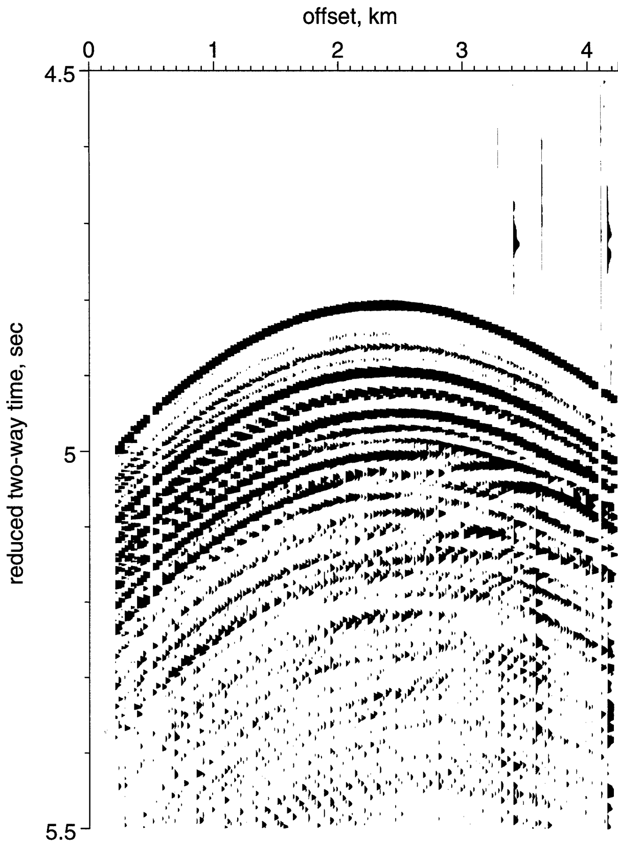
Crustal age -11 my. Layer 2A base refraction appears on only a few traces
