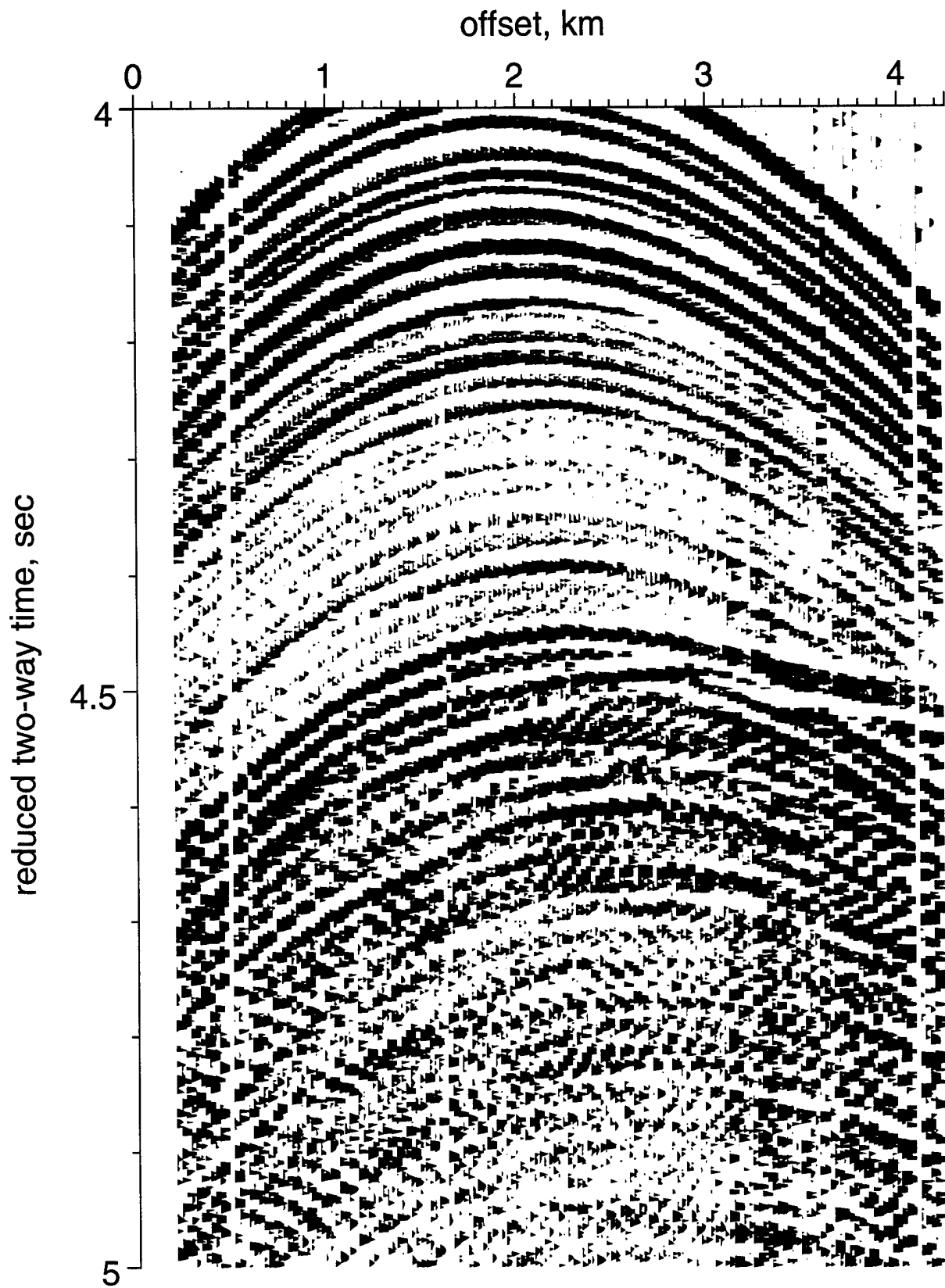
Crustal age 5.2my. Layer 2A is very thin L-DEO mcs line 1266 cdp 60825
