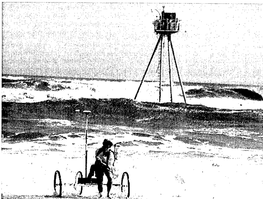
Figure 6. The CRAB conducting a minigrad survey with the "Dolly" surveying in the foreground
